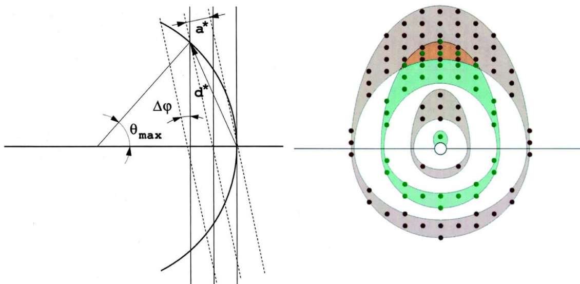
Figure 26: Origin of the reflections zones overlap and calculation of the limiting rotation range. From Dauter Acta Crystallographica D. 1999
