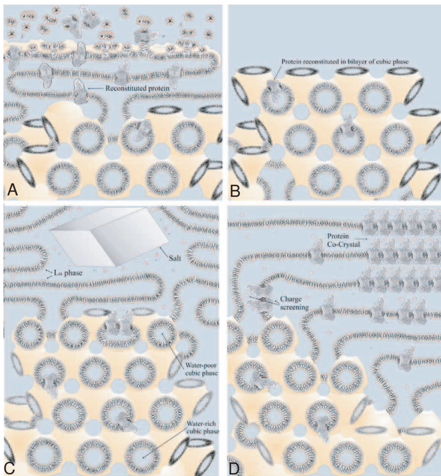
Figure 17: Crystallization mechanism in cubic lipidic phase. (A) Protein reconstitution and dispersion in mesophases. (B) Reconstituted protein in bilayer of cubic phase. (C) Addition of precipitant (salt) to initiate crystallization by water-withdrawing and charge screening effect. Bilayer curvature in cubic phase increases as water content drops. (D) Reversible crystallization of the protein from cubic phase through lamellar portal. From Caffrey et al. [59]
