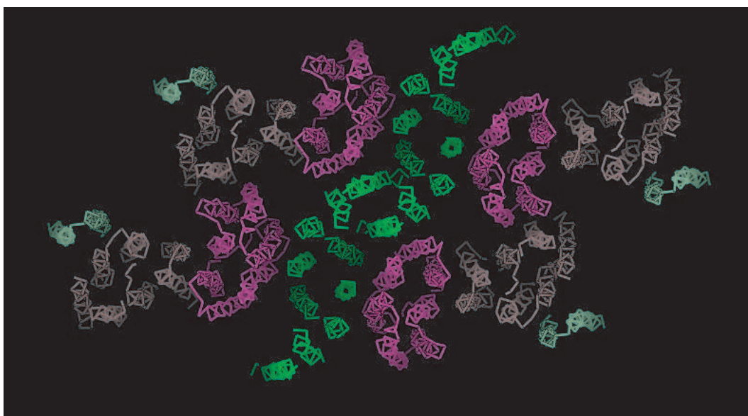
Figure 43: Putative trace model of the transducer including several helical fragments derived for the twinned crystal model
