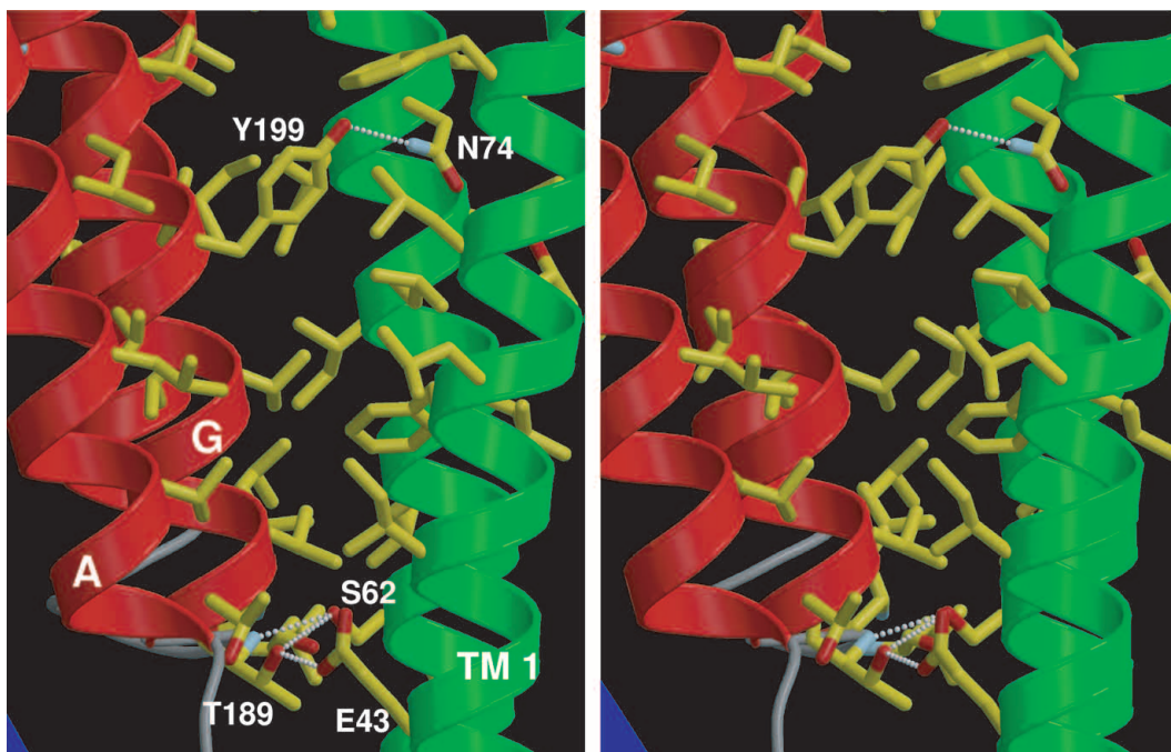
Figure 12: Stereo view of the hydrogen bonds and van der Waals contacts between receptor and transducer. The residues that are involved in hydrogen bonds are labelled. From Gordeliy et al. [47]
