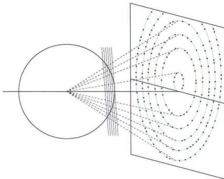
Figure 25: A still exposure with a stationary crystal contains only a small number of reflections arranged in a set of narrow ellipses. From Dauter Acta Crystallographica D . 1999
