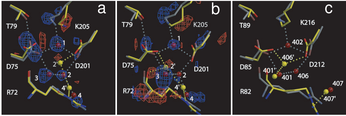
Figure 57: Extracellular vicinity of the retinal Schiff Base. Hydrogen bond pattern including 4 water molecules, Lys205, aspartic acids Asp75 and Asp201, Arg72 and Thr79 side chains: ground state (grey), intermediate states (yellow), negative (blue) and positive (red) electron densities, water molecules of ground state red and intermediate state yellow balls, hydrogen bonds in dotted lines in grey for ground state and in yellow for M state. (a) K state of pSRII-HtrII(1-114) complex with electron density maps contoured at 4.5\sigma and -4.5\sigma , respectively. (b) M state of pSRII-HtrII(1-159) complex with electron density maps contoured at 3\sigma and -3\sigma , respectively. (c) ground and M state conformations of Bacteriorhodopsin
