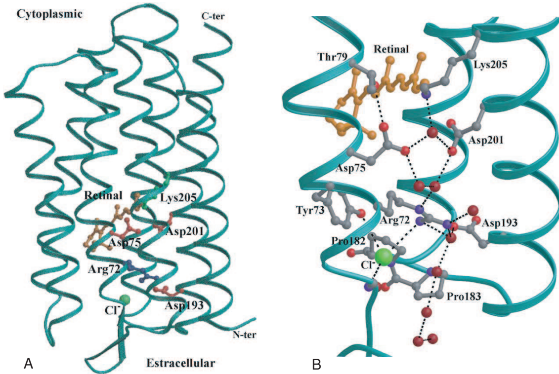
Figure 9: Sensory rhodopsin pSRII structure overview. (A) C_{\alpha} trace representation. Key residues and the retinal are highlighted. (B) Hydrogen bonding network between the retinal binding site and extracellular surface. The retinal, water molecules and key residues are highlighted. From Pebay-Peyroula et al. BBA 2002.
