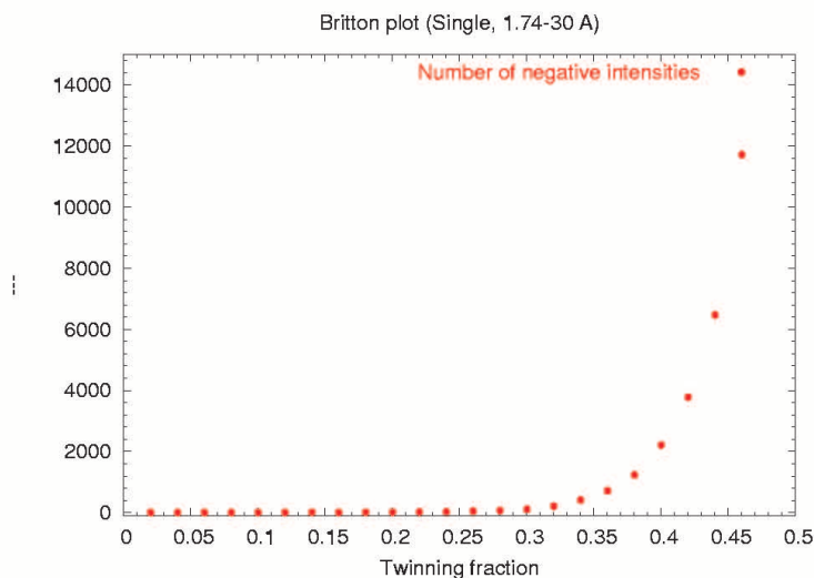
Figure 40: Britton plot for the ground state data collected from pSRII-HtrII complex crystals
