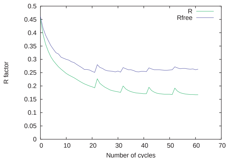
Figure 33: Refinement R factors monitored during the refinement run following ARP protocol. Green - conventional R factor, blue - free R factor
