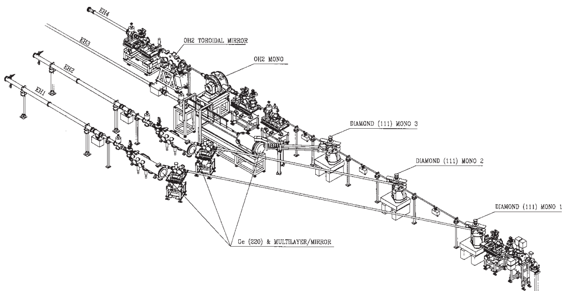
Figure 23: Schematic view of the Quadriga beamline ID14 at the ESRF. From Lindley [67]
