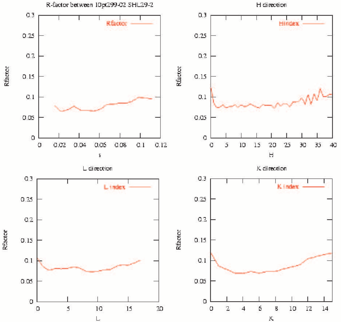
Figure 45: Scaling of the derivative data to native data. Overall R factor and R factor for the selected axial direction (h00), (0k0) or (00l) are presented
