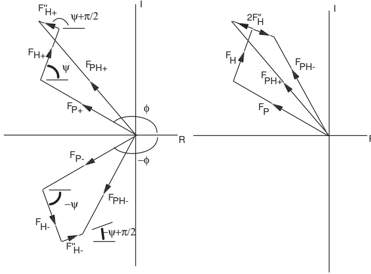
Figure 21: Anomalous difference within the Bijvoet pair
