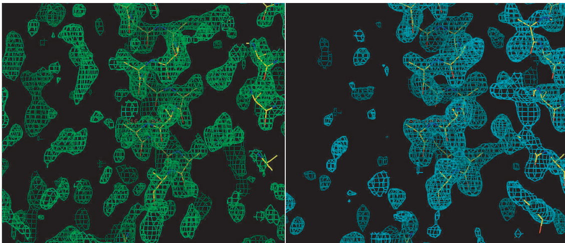
Figure 42: 2F_o - F_c electron density maps for located polyalanine helical fragments. Green - electron density map for the case of crystal with two orientations of pSRII following molecular replacement solutions. Blue - electron density map for the twinned model of the crystal. Both maps are contoured at 0.8\sigma
