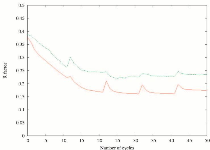
Figure 49: R factors monitored during the refinement run following ARP protocol. Red - conventional R factor, green - free R factor
