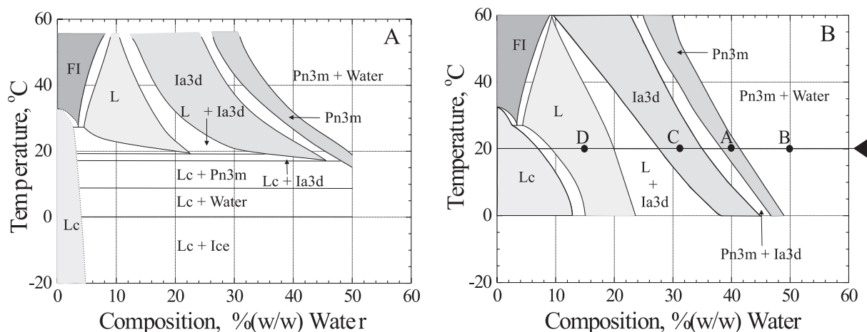
Figure 16: Monooleyl-water phase diagram. A. Equilibrium phase diagram. B. Metastable phase diagram. From Caffrey et al. Journal of Structural Biology . 2003
