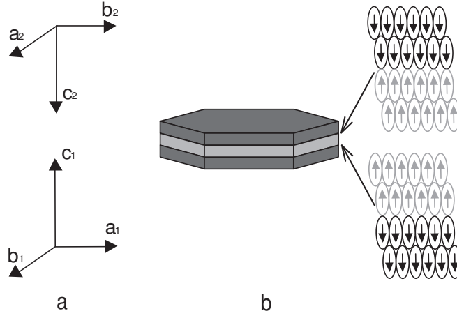
Figure 37: Example of the twinning. Crystal consists of several twin domains which have an identical crystalline structure. From Efremov et al. [84]
