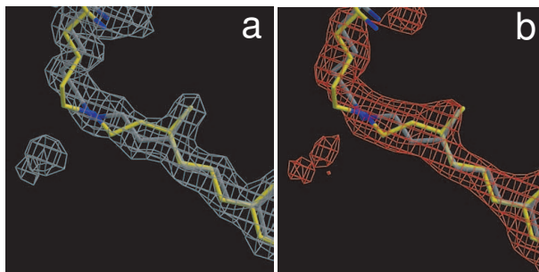
Figure 51: 2F_o - F_c electron density and retinal models for pSR11-Htr11 complex. (a) Ground state density and retinal models of ground and M state. (b) Composite omit map for illuminated crystal data and retinal models. Grey model - ground state, yellow model - M state.
