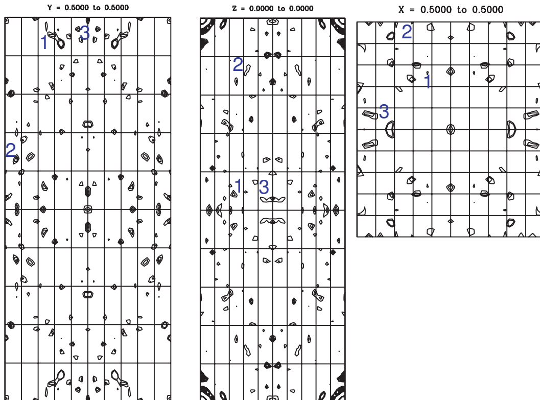
Figure 46: Harker sections plot for the isomorphous Patterson map calculated for F_{PH} - F_P
