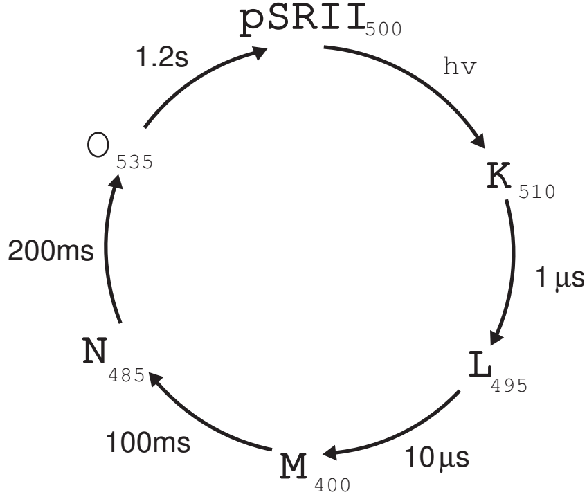
Figure 8: Sensory rhodopsin pSRII photocycle. The spectral intermediates, their absorption maxima and their lifetimes at room temperature are shown
