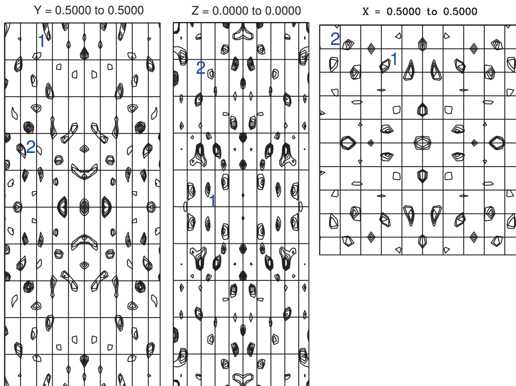
Figure 48: Harker sections plot for the anomalous difference Patterson map calculated for F_+ - F_-
