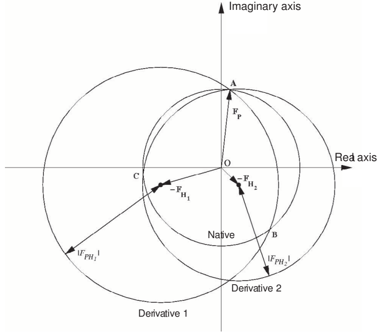
Figure 19: Harker construction for multiple isomorphous replacement
