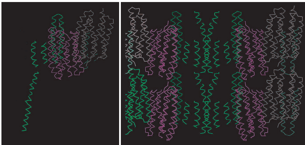
Figure 43: Putative trace model of the transducer including several helical fragments derived for the twinned crystal model
