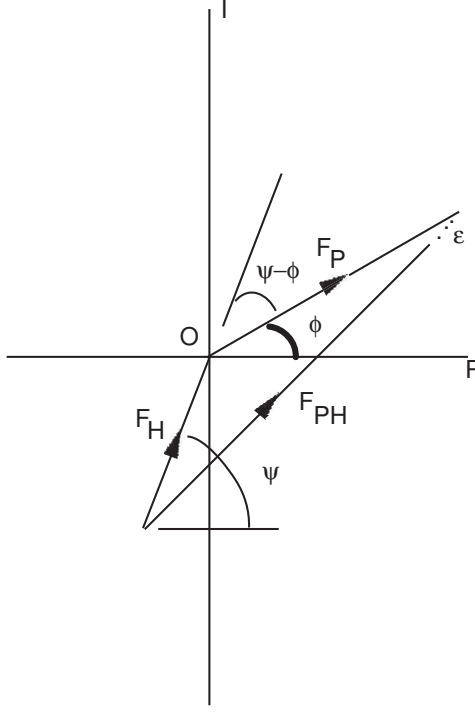
Figure 20: Introduction of the lack of closure of the triangle error to evaluate the phase probabilities
