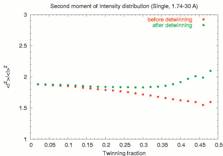
Figure 39: Plot of the second moment of the intensity distribution for the ground state data collected from pSRII-HtrII complex crystals
