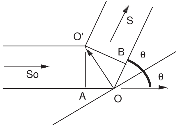
Figure 18: Diffraction of the scattered X-ray wave from two point object
