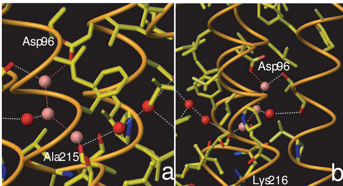
Figure 62: Proton translocation pathway between Asp96 and Schiff base in late M state. Pink are water molecule chain appearing in the M state.
