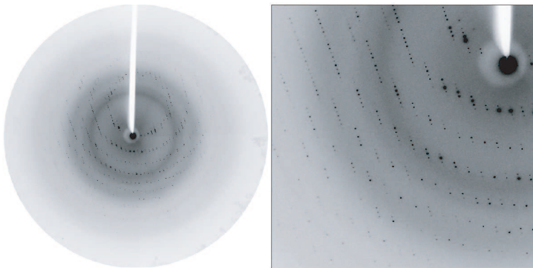
Figure 32: Diffraction pattern to 1.8 Å resolution recorded from pSRII-HtrII complex crystals.
