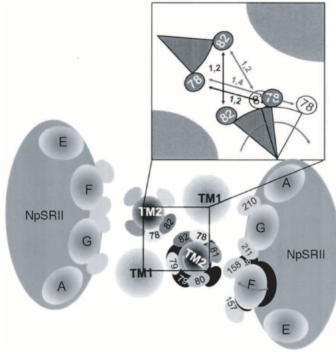
Figure 13: Schematic representation of the light induced conformational changes in 2:2 receptor-transducer complex. View from the cytoplasmic side. Arrows shows the conformational changes. Wegener et al. EMBO Journal 2001
