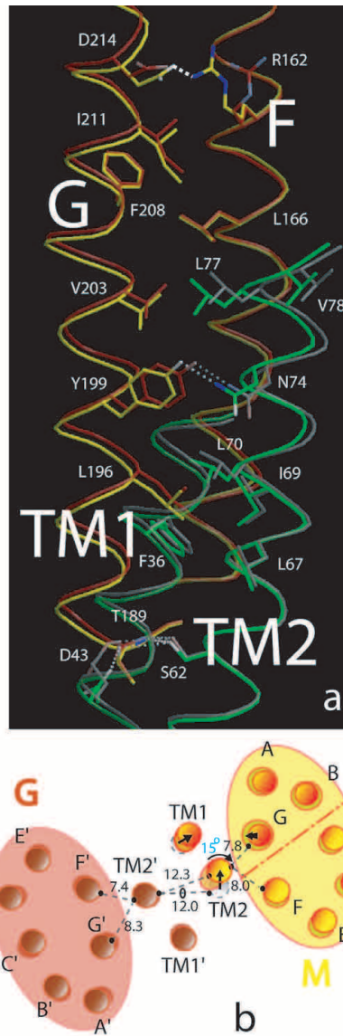
Figure 59: Overall views on helices F, G, TM1 and TM2 in ground and late M state. a. Structural changes along this helices; b. schematic picture of helical displacements viewed from the cytoplasmic surface, ground state complex in red and M state complex in yellow, black numbers gives the distances between C_{\alpha} atoms of the following amino acids in ground and in M state: F(L70)-TM2(L77): ground state - 7.4 Å, M state - 8.0 Å, G(V203)-TM2(L77): ground state - 8.3 Å, M state - 7.8 Å, TM2(V78)-TM2'(V78): ground state - 12.0 Å, M state - 12.3 Å. The arrows on TM1 and TM2 depict displacements parallel to the membrane plane in M state, the arrow on helix G depicts its downward movement. A clockwise rotation of 15^{\circ} is observed for TM2 and an in-plane displacement of 0.9 Å (black arrow) near the cytoplasmic membrane surface in M state with respect to the ground state. A red line in the receptor (colored in yellow) divides the molecule into the two functionally important domains ABG and CDEF
