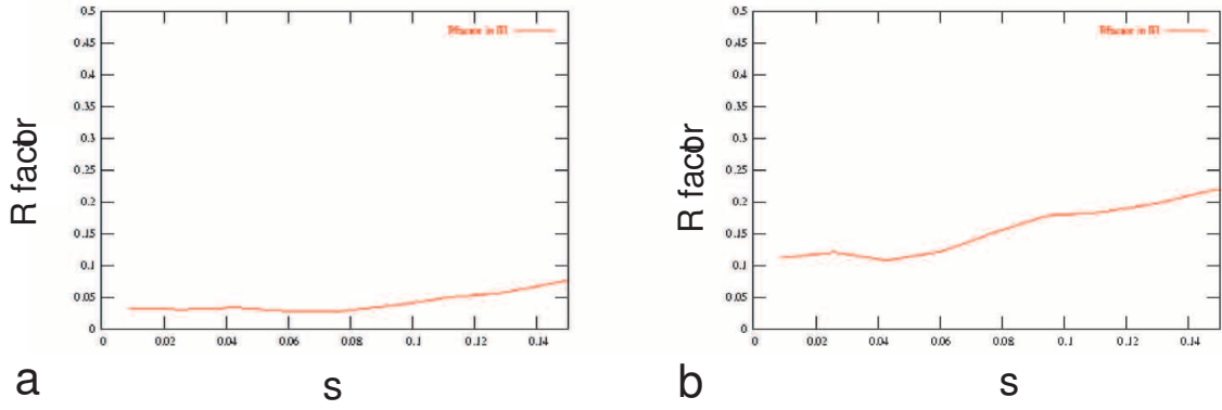
Figure 50: R factor calculated between A. the not illuminated data from different crystals and B. illuminated and not illuminated data from the same crystal
