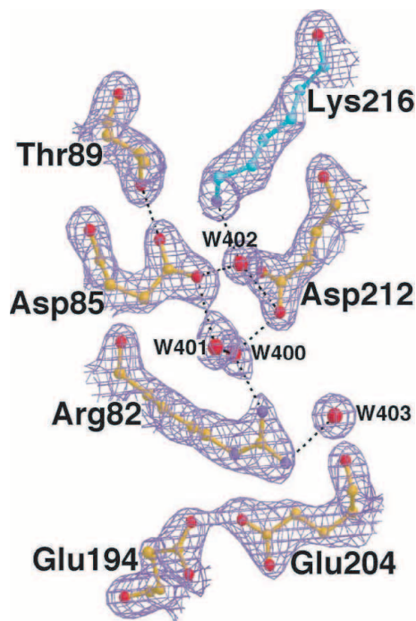
Figure 5: Refined structure and electron density of the extracellular half of BR in the ground state. 2F_{obs} - F_{calc} refined electron density map contoured at 1.2 \sigma shows the structure of the Schiff base counter ion formed by Asp85, Asp212, Wat400, Wat401, Wat402, Arg82. The proton release group is thought to be formed by Glu194, Glu204 and water molecules. (From Neutze et al. BBA 2002)
