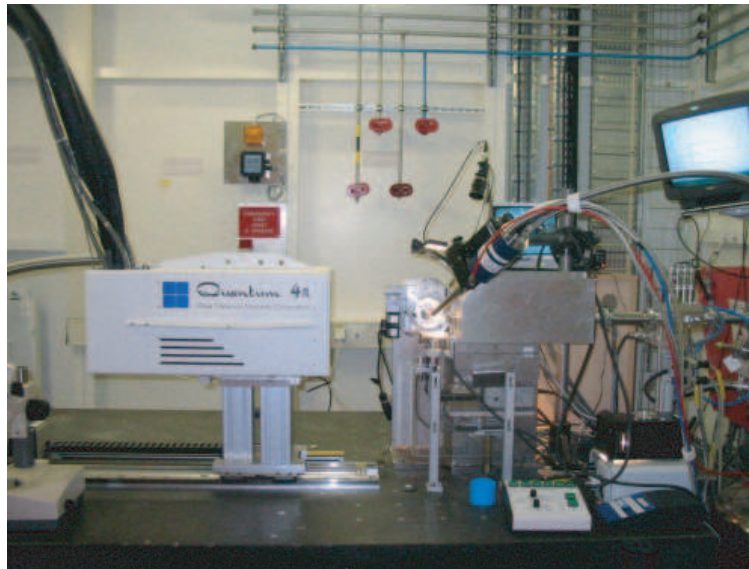
Figure 24: Beamline ID14-1 experimental hutch overview. From http://www.esrf.fr/UsersAndScience/Experiments/MX/ID14-1/
