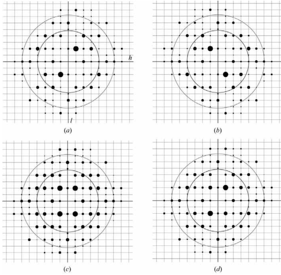
Figure 38: The effect of twinning by a two fold rotation about a -axis on the diffraction pattern of monoclinic crystal. (a) h0l -zone from a single crystal, representing diffraction from one domain. (b) same pattern but rotated around a . (c) superposition of a and b simulating the perfect twinning \alpha = 0.5 case. (d) superposition of a and b simulating twinning with \alpha = 0.2 . From Parsons [83]
