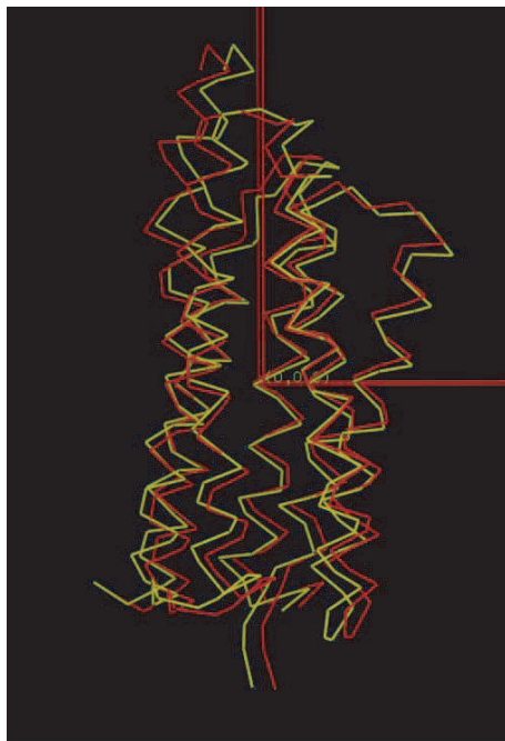
Figure 36: 4 degree difference in rotation angles between two solutions of molecular replacement rotation search for pSR11
