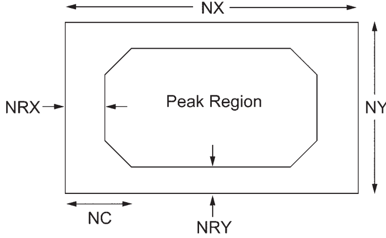
Figure 27: Definition of the peak and background regions for summation integration and profile fitting. Listed are the parameters to define the profile. From Leslie [68]
