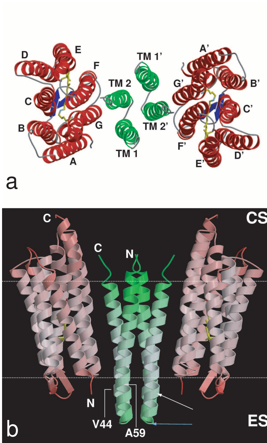
Figure 11: Fold of the receptor-transducer complex. (A) Ribbon diagram of the top view from the cytoplasmic side. (B) Side view of the complex. From Gordeliy et al. [47]
