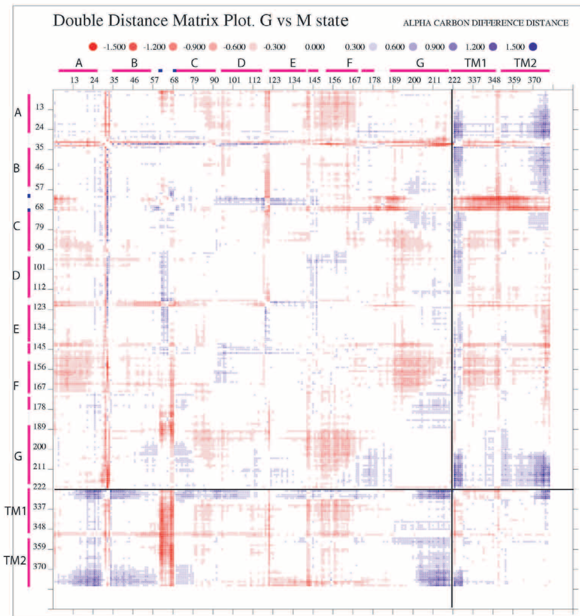
Figure 55: Double distance matrix plot for pSRII-HtrII(1-159) complex conformations of ground and M state. Contoured at the 1.5 Å level in color grade steps of 0.3 Å. Calculated for residues 3-222 of pSRII and 27-79 of HtrII denoted as 327-379 respectively.
