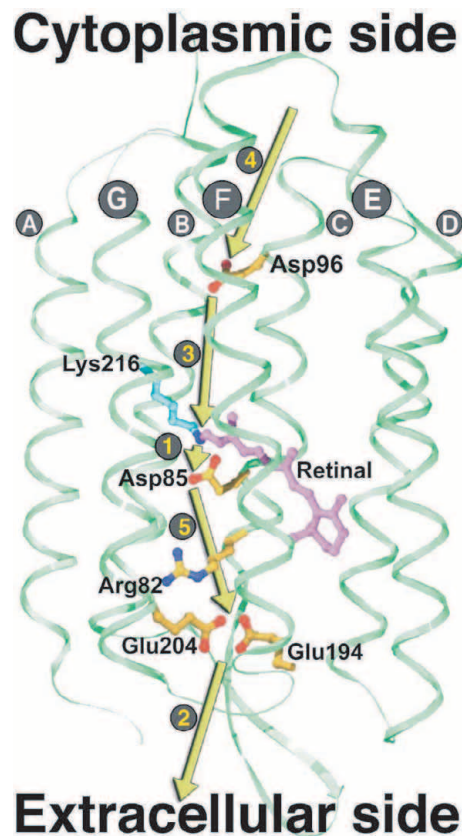
Figure 6: Schematic representation of the proton transfer steps in BR pumping cycle, overlaid on the ground state model. The primary proton transfer (1) is from the Schiff base to Asp85. A proton is released to the extracellular medium (2) by a proton release group, thought to be formed by Glu194 and Glu204 and/or water molecules. The Schiff base is subsequently reprotonated from Asp96 (3) which is then reprotonated from the cytoplasmic medium (4). The final proton transfer step (5) from Asp85 to the proton release group (via Arg82) restores the ground state. (From Neutze et al. BBA 2002.)
