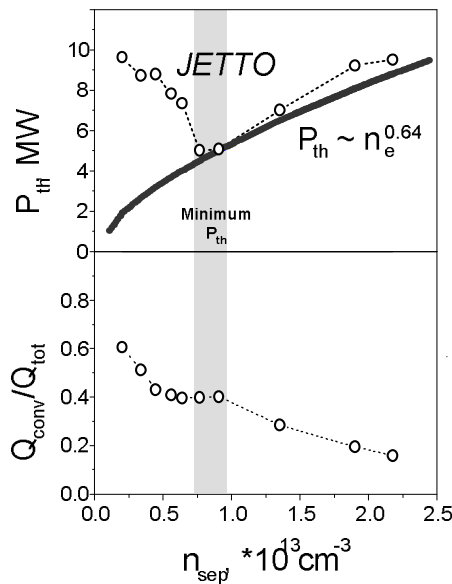
Fig.3 L-H power threshold computed with the JETTO code for low density conditions: the minimum of P_{th}(n_e) dependence correspond to the critical fraction of convective heat losses at the edge, Q_{conv}/Q_{tot} \sim 0.4 .
