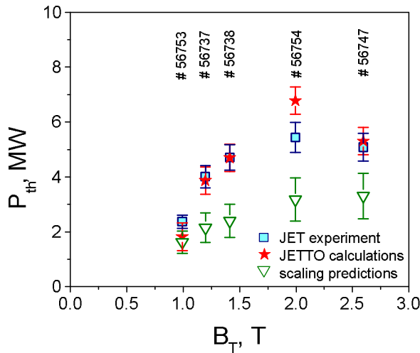
Fig.2 Comparison of the L-H power threshold computed with the JETTO code to the values obtained in experiment and predicted by the inter-machine scaling, for the set of discharges with various magnetic field.
