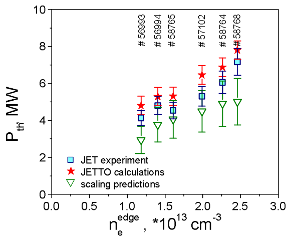
Fig.1 Comparison of the L-H power threshold computed with the JETTO code to the values obtained in experiment and predicted by the inter-machine scaling, for the set of discharges with various densities.
