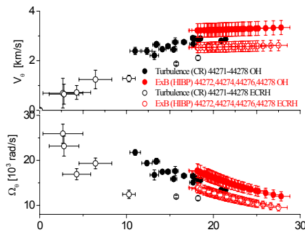
Fig. 4. Comparison of rotation velocities of density perturbations (black) with core plasma rotation (red) in OH (filled) and ECRH (open) plasma.
