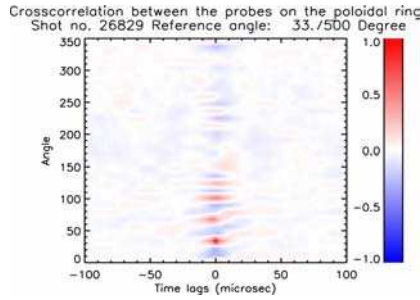
Fig.1. Spatial-temporal correlation function along the poloidal ring of probes.
