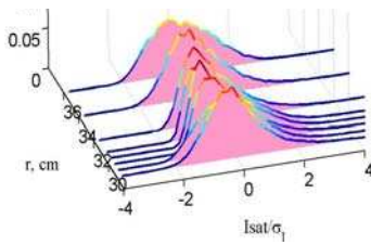
Fig.5. PDF in the SOL of T-10
