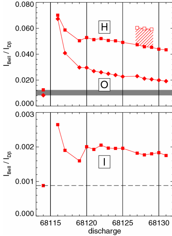
Figure 2: Evolution of Be II intensity normalised to D_{\beta} for main chamber (H), outer (O) and inner divertor (I). The hatched area denotes the effect of a 6 cm plasma shift towards the central wall.
