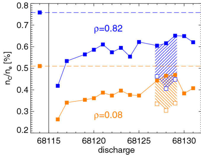
Figure 4: Evolution of carbon plasma concentration f_C = n_C/n_e in plasma centre (normalised radius \rho=0.08 ) and outer plasma region ( \rho=0.82 ). The hatched areas denote the effect of a 6 cm plasma shift towards the central wall. In 3 discharges, the plasma was also shifted by 6 cm towards the central wall. This leads to increased erosion of Be and C at the central column (Figure 2 and Figure 3), however, at the same time the carbon concentration decreases significantly. From these observations one infers that carbon sources at the outboard wall and limiters contribute much more to the carbon level in the plasma than C sources at the central column.
