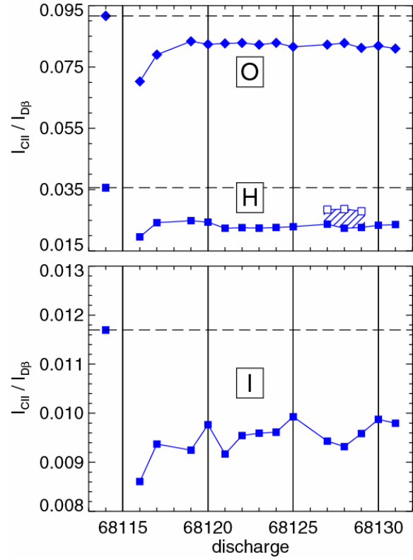
Figure 3: Evolution of C II intensity normalised to D_{\beta} for main chamber (H), outer (O) and inner divertor (I). The hatched area denotes the effect of a 6 cm plasma shift towards the central wall.
