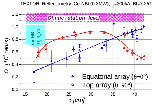
Figure 3: Turbulence angular velocity for a regime with co-NBI ( 0.3\text{MW} ).
