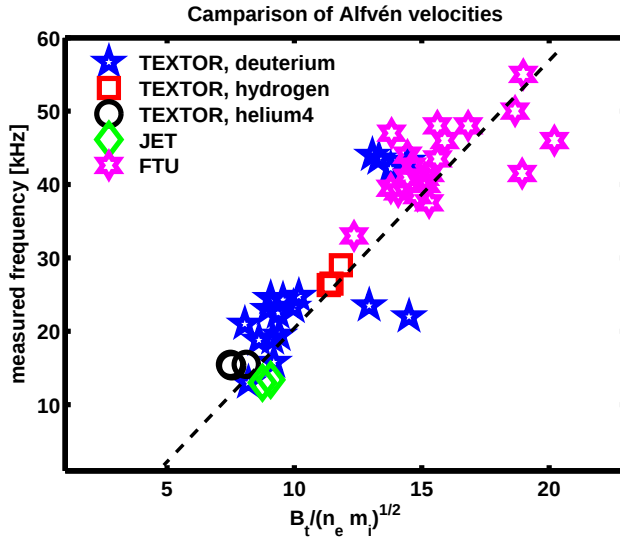
Figure 3: The measured mode frequency of JET, FTU and TEXTOR show its linear dependency on the Alfvén velocity. The TEXTOR discharges are distinguished into those with different operation gases: Hydrogen, Deuterium and Helium4.
