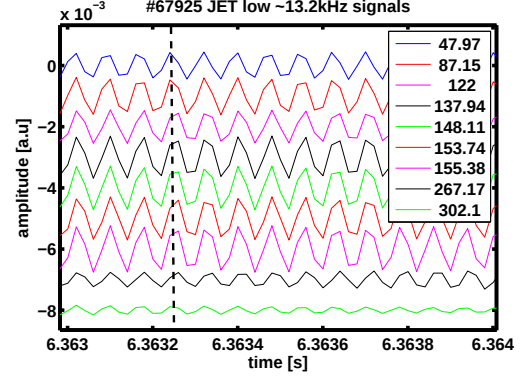
Figure 2: Band pass filtered signals from several toroidally separated Mirnov show no phase shift of the oscillation. The included legend presents the toroidal angle of the coil position.
