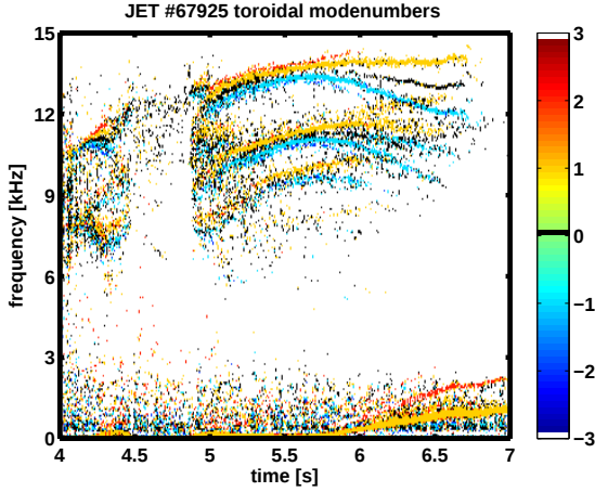
Figure 1: The toroidal mode number estimation of a JET discharge shows a slowly rotating n=1 mode below 1 kHz, which accelerates at 5.5s. In the frequency range of 7 – 15 kHz several pairs of n=1 and n=-1 modes are seen. Between these modes a n=0 mode is seen.
