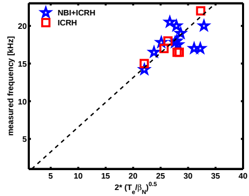
Figure 6: Referring to equ. 3 and equ. 4 c_s/\sqrt{\beta} \sim v_A . Here the measured mode frequency is used to determine v_A . The linear dependency indicates, that these modes scale with the Alfvén speed and not with the sound speed. Again the blue stars indicate discharges with slight NBI heating for diagnostic purpose and ICRH, the red squares show discharges with ICRH only.
