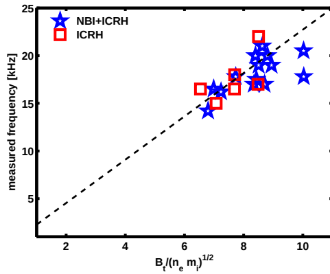
Figure 5: Two groups of discharges of the \beta scan are shown. The blue stars indicate discharges with slight NBI heating for diagnostic purpose and ICRH, the red squares show discharges with ICRH only. The Alfvén velocity scaling of the measured frequency is seen. The linear dependency is indicated by the dashed straight line.
