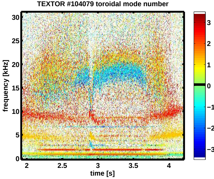
Figure 4: The toroidal mode number estimation of a TEXTOR discharge shows a rotating n=1 mode at 1 kHz, which was excited by the DED in 3/1 configuration. From 2.1 s in the frequency range of 13 – 20 kHz n = 1 and n = -1 modes appear, which can be seen more clearly, when the 2/1 is excited at 2.7 s. A rotating external perturbation field below the mode onset threshold is able to excite the Alfvén like modes [1].
