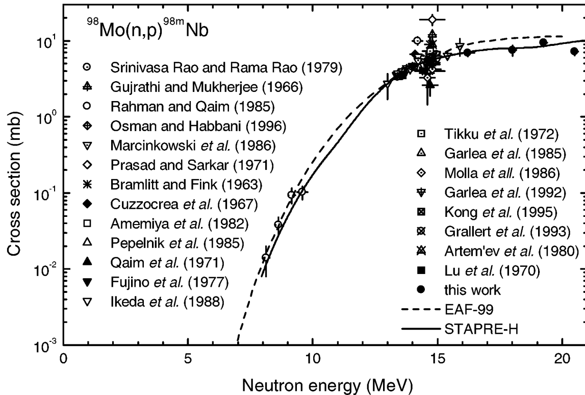
Figure 5.6: Comparison of the measured reaction cross sections for the ^{98}\text{Mo}(n,p)^{98m}\text{Nb} reaction with existing experimental data [89, 95, 102, 103, 107, 112, 113, 115, 116, 121–127], evaluations and STAPRE-H calculation.
