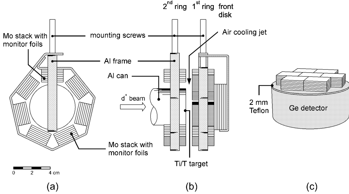
Figure 3.1: Sketch of the used Mo-target: (a) the front view shows the front disk and the first ring (b) a part of the second ring is not shown in order to allow a view on the beam line (c) counting geometry for the 1 st and 2 nd ring
