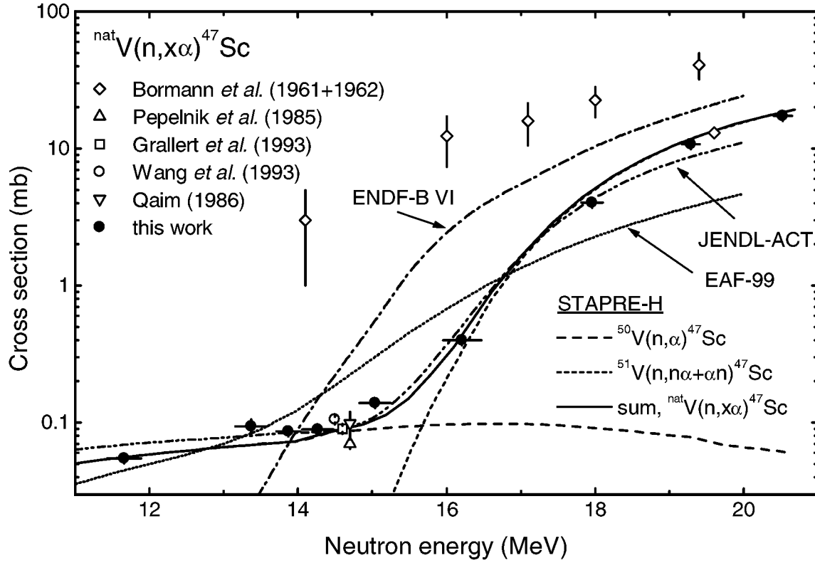
Figure 5.1: Comparison of the measured cross sections for the {}^{\text{nat}}\text{V}(n,x\alpha){}^{47}\text{Sc} reaction with existing experimental data [31–33,35,89,90], evaluations and STAPRE-H calculations
