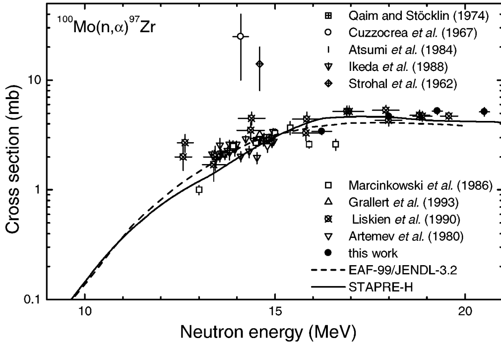
Figure 5.12: Comparison of the measured cross sections for the ^{100}\text{Mo}(n,\alpha)^{97}\text{Zr} reaction with existing experimental data [42,89,95,106,114,120,121,129], evaluations and STAPRE-H calculations.
