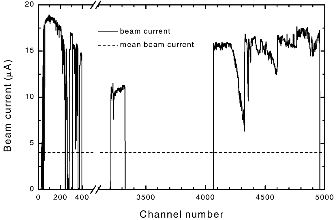
Figure 3.8: Neutron flux of the irradiation performed for the ^{\text{nat}}\text{Mo}(n,x)^{94}\text{Nb} cross section measurement. The total irradiation time was 410 h with an average beam current of 4 \mu\text{A} . Taking into account the interruptions and maintenance breaks, an effective irradiation time of 110 h with a mean beam current of 15 \mu\text{A} is obtained.
