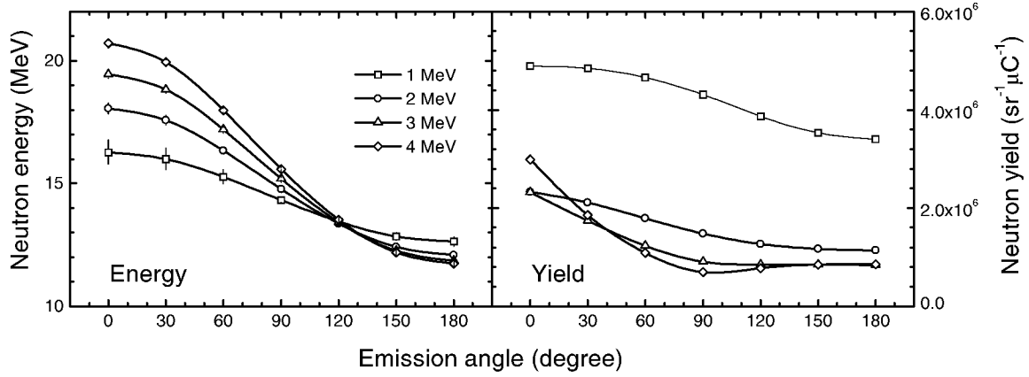
Figure 1.3: Angular distribution of neutron energy and neutron yield for the {}^3\text{H}(\text{d},\text{n}){}^4\text{He} reaction. The calculations were done for four different incident deuteron energies using the program KINEMA (cf. section 3.3.2)
