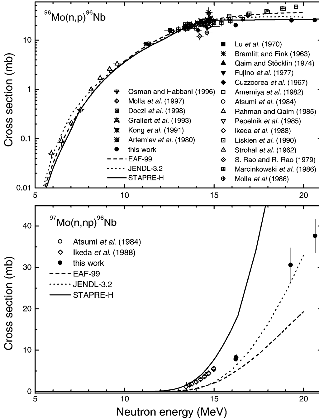
Figure 5.8: Comparison of the measured cross sections for the ^{96}\text{Mo}(n,p)^{96}\text{Nb} and ^{97}\text{Mo}(n,np)^{96}\text{Nb} reactions with existing experimental data [89, 95, 98, 103, 105–107, 109, 112–116, 120–123, 126, 128, 129], evaluations and STAPRE-H calculations.
