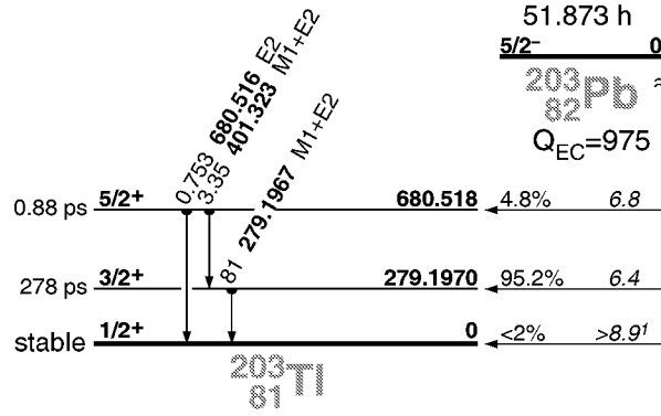
Figure 3.13: Decay scheme of ^{203}\text{gPb} to illustrate the summing coincidence corrections, taken from [74]
