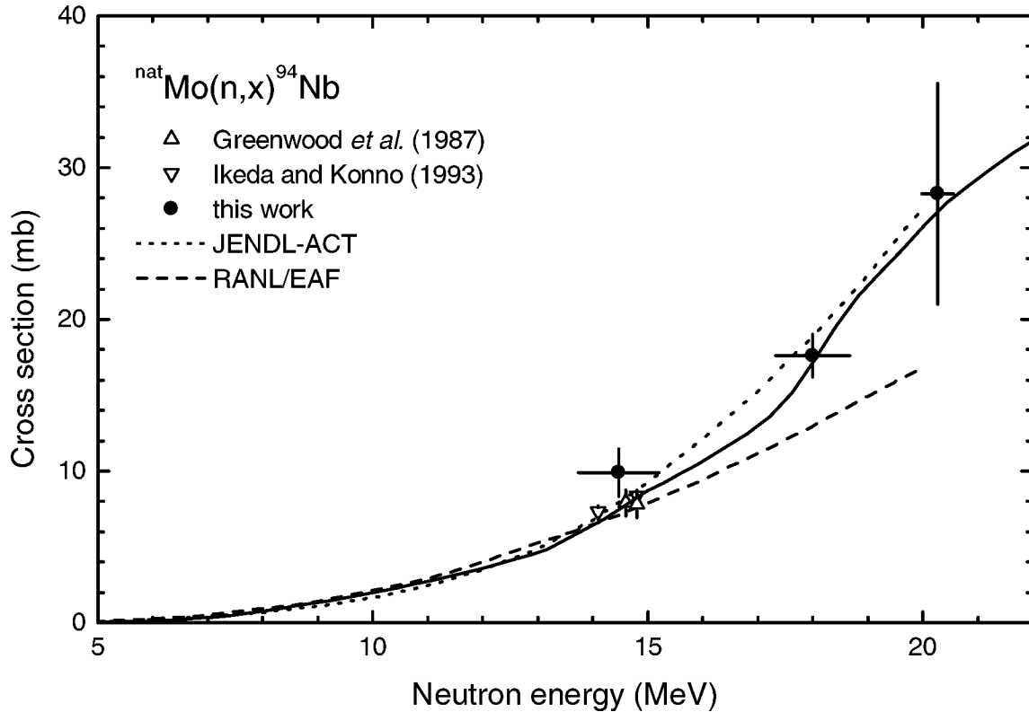
Figure 5.4: Comparison of the measured cross section for the ^{\text{nat}}\text{Mo}(\text{n},\text{x})^{94}\text{Nb} reaction with existing experimental data in the 14 MeV region [40, 41], evaluations and STAPRE-H calculations.
