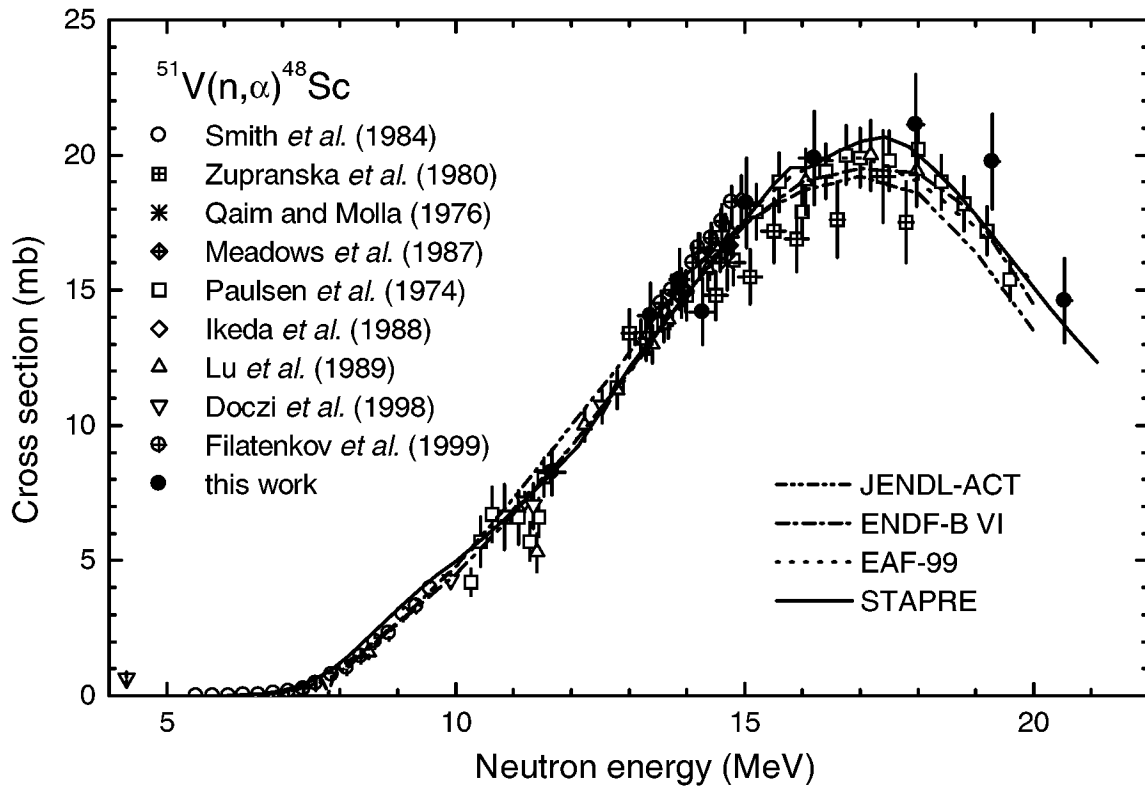
Figure 5.2: Comparison of the measured cross sections for the ^{51}\text{V}(n,\alpha)^{48}\text{Sc} reaction with existing experimental data [92–99], evaluations and STAPRE-H calculations
