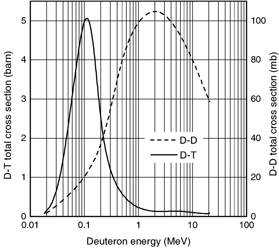
Figure 1.2: Energy dependence of the total cross section for the {}^2\text{H}(\text{d},\text{n}){}^3\text{He} and {}^3\text{H}(\text{d},\text{n}){}^4\text{He} reactions, taken from [17]
