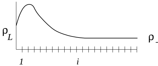
FIG. 2. Coupling of a semi-infinite driven particle system to a reservoir of constant particle density \rho_L . The (interpolated) density profile \rho_i ( i = 1, 2, \dots ) approaches some constant value \rho_- after some finite distance from the boundary.
