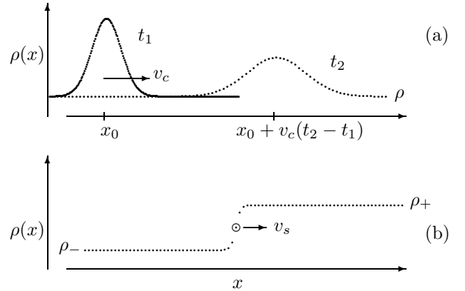
FIG. 3. (a) Diffusive spreading of a density perturbation in the stationary state at two times t_2 > t_1 . The collective velocity describes the motion of the center of mass of the perturbation. (b) Motion of a shock. To the left of the domain wall particles are distributed homogeneously with an average density \rho_- . To the right of the domain wall the background density is \rho_+ > \rho_- .
