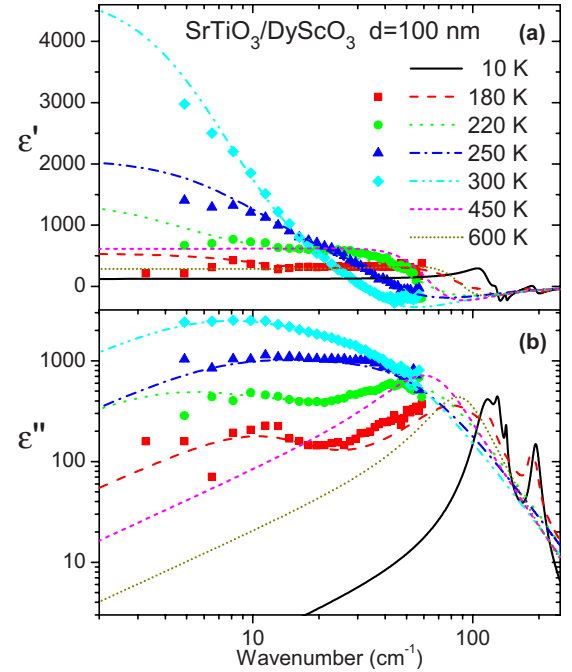
FIG. 2. (Color online) (a) Real and (b) imaginary part of the dielectric function (lines) of the 100 nm STO film obtained from fitting the IR reflectance along with the terahertz data (symbols).
