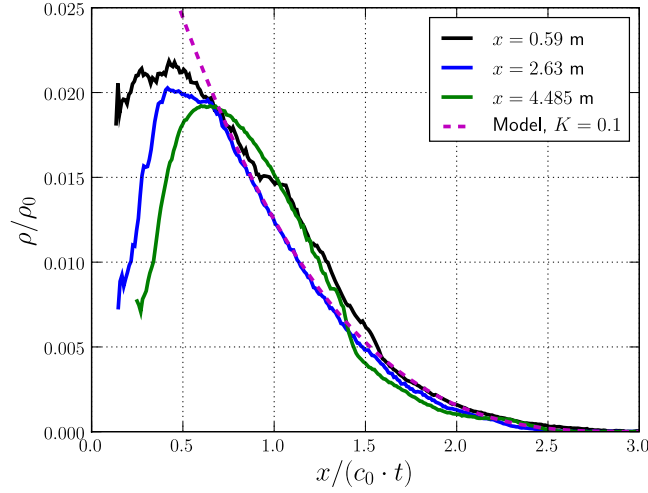
Figure 3: Comparison of the model with interferometric density measurement (neon, c_0 \approx 450 m/s, S_{\text{orifice}}/S_{\text{tube}} \approx 0.06 ).
