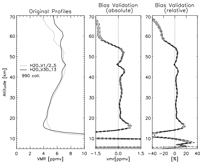
Fig. 1. Left panel: MIPAS H2O_V3O_V13 (solid) and H2O_V1/2.5 (dotted) mean profiles. Middle panel: Absolute bias MIPAS (V1/2) – MIPAS (V3O) (solid) with its uncertainty (dashes). Right panel: Relative bias MIPAS (V1/2) – MIPAS (V3O) (solid) with its uncertainty. The uncertainties in the middle and right panel are given in terms of two standard deviations of the mean (dashes).
