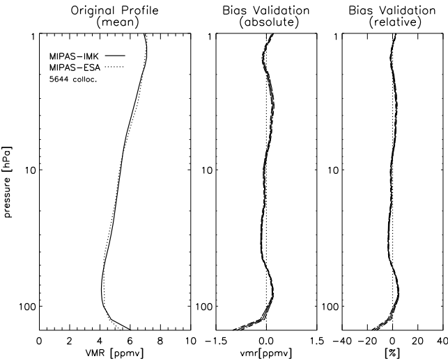
Fig. 25. Comparison of MIPAS H 2 O profiles retrieved by IMK (solid) and the official ESA version 4.61/4.62 H 2 O data product (dotted), northern mid-latitudes, 5644 coincidences.
