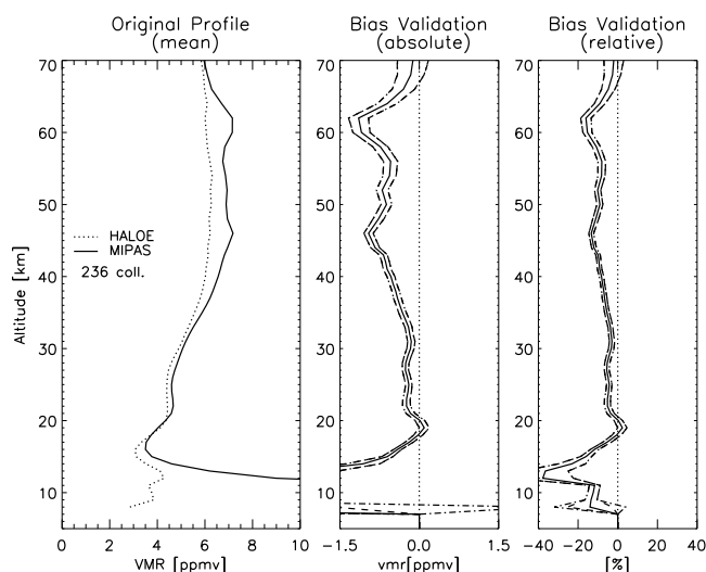
Fig. 4. As Fig. 2 but for HALOE sunset measurements.
