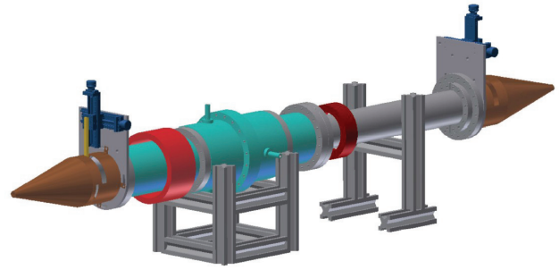
Figure 2: The test station for the beam current measurement devices. Different beam current sensors can be implemented in to the test stand. The wire inside the tube is moved using XY tables (blue) mounted on both sides of the system. The wire tension system is covered inside the tapers (copper colored).
