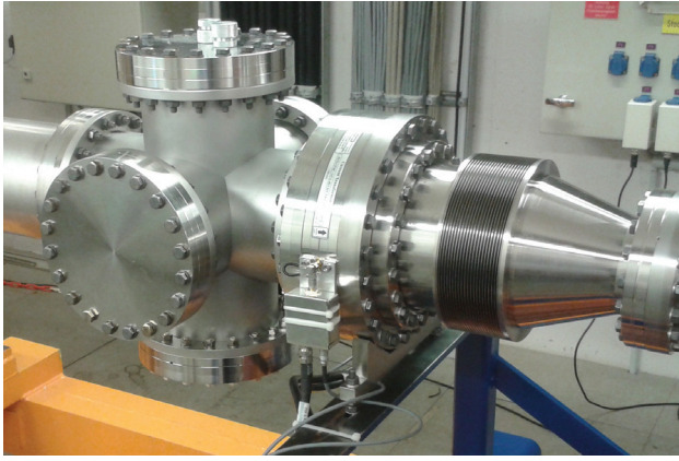
Figure 1: The Fast Current Transformer from Bergoz Instrumentation installed at COSY. The FCT in the ring is equipped with a custom build preamplifier and a current source for calibration. The main parts of the readout and calibration module are installed outside the tunnel.
