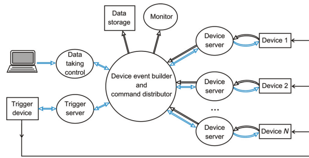
Figure 5: Layout of the DAQ prepared for the high resolution beam current measurement system. All the physical devices (rectangles), including custom build trigger model, are communicating with software (ovals) running on a readout and control PCs over the 1Gb Ethernet. All the readout devices get hardware trigger signals from the trigger device via dedicated coaxial lines.
