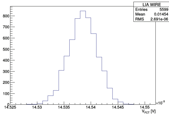
Figure 6: Current in the wire measured using the FCT in the laboratory. An electrical current which simulates 1 mA beam current of COSY has been measured by an FCT in the test stand using the measurement scheme presented in Fig. 4. The voltage signal generated by FCT was measured for 1.5 h using a LIA.
