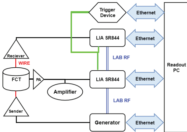
Figure 4: The Fast Current Transformer readout scheme in the laboratory. Similar to the readout scheme presented in Fig. 3 all the devices controlled by a common DAQ discussed in a next section but instead of COSY beam, an electrical signal in a conductive wire is generated by an arbitrary wave form generator.
