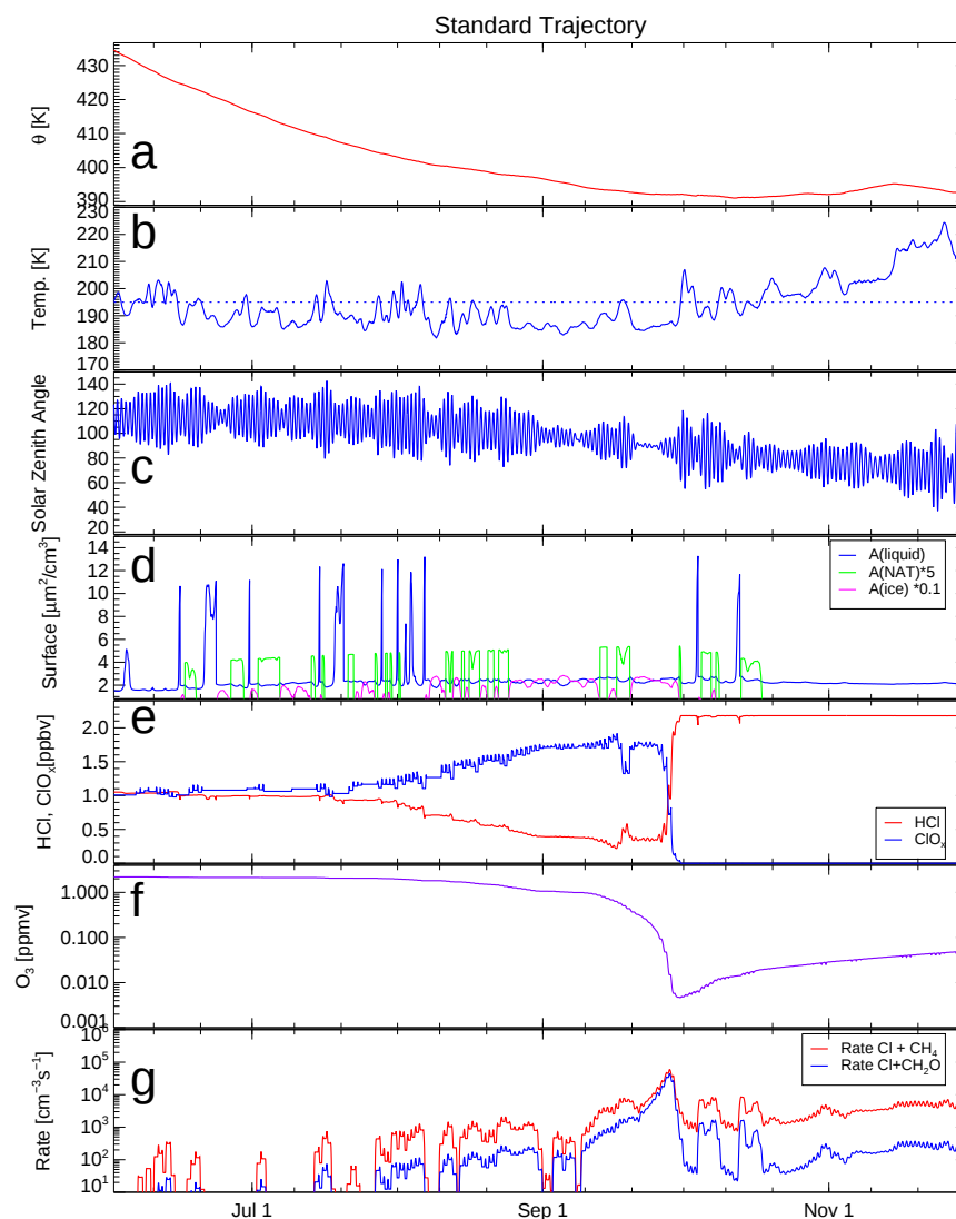
Figure 1. Box-model simulations along a trajectory passing through the location of the ozone sonde observation at South pole of 14 ppbv on 74 hPa (391 K) on 24 September 2003 (Groß et al., 2011). The different panels show a time series of the relevant parameters: (a) potential temperature of the air parcel, (b) temperature, (c) solar zenith angle, (d) surface area density of ice (red, scaled by 0.1), NAT (green, scaled by 5) and liquid aerosol particles (blue), (e) \text{ClO}_x (red), and HCl (blue), (f) ozone, and (g) rates of reaction of atomic chlorine with \text{CH}_4 (blue) and \text{CH}_2\text{O} (red). For reasons of clarity, the reaction rates in panel (g) are plotted as 24 h running averages. The model simulation covers the time period from 1 June to 30 November 2003.
