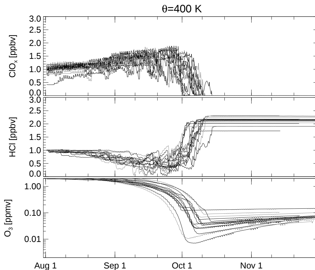
Figure 4. Results from multi-trajectory simulations of CLaMS. Box-model simulations were performed for a set of trajectories passing the South pole at 400 K taken from (Groß et al., 2011). The box-model simulations cover the time period from 1 August to 30 November 2003. A few trajectories showing very little diabatic descent (and thus much smaller values of total chlorine) were neglected. Initial values were chosen consistently with the reference run (Fig. 1). Individual trajectories are shown in different shades of grey to allow them to be distinguished more easily.
