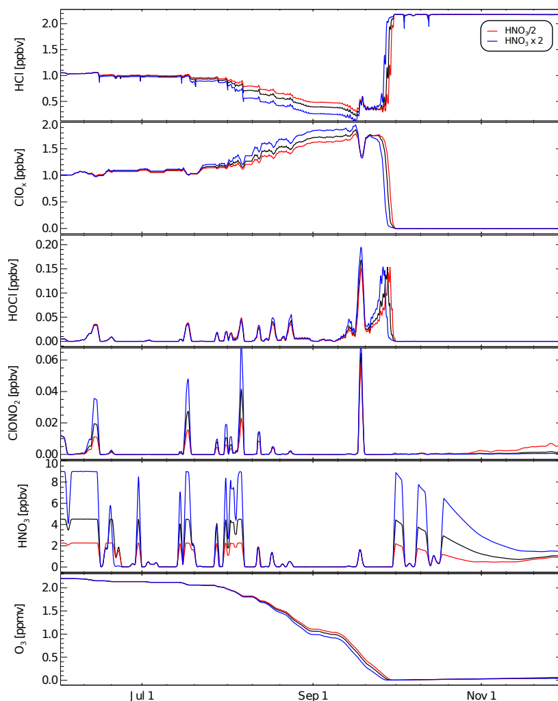
Figure A2. Simulation for the impact of denitrification. The impact of denitrification is tested by initialising the model run with HNO 3 doubled and halved.
