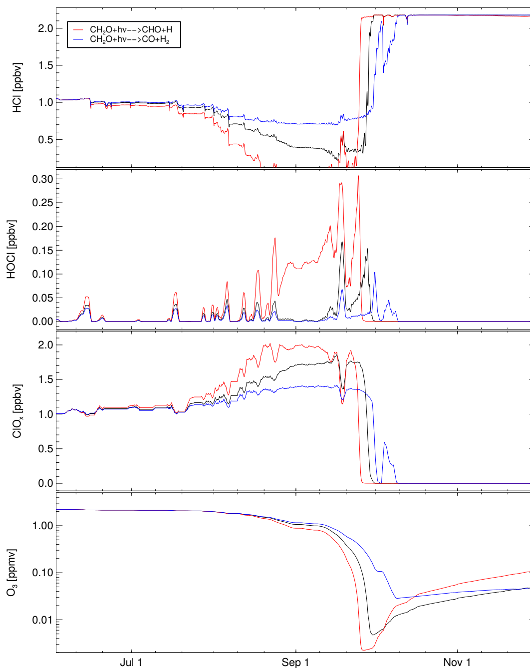
Figure 2. Sensitivity of the ozone hole chemistry on \text{HO}_2 production in the photolysis of \text{CH}_2\text{O} . Black lines show the reference case, red line a case assuming 100% efficiency for \text{HO}_2 production (i.e. for reaction R14), and blue line a case assuming no \text{HO}_2 production in the photolysis of \text{CH}_2\text{O} (100% efficiency for reaction R23).
