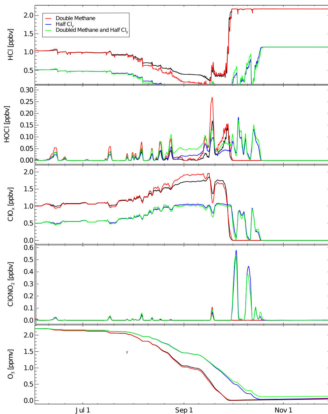
Figure 3. Sensitivity of the ozone hole chemistry on stratospheric methane and chlorine levels. Black lines show the reference case, red line a case assuming initial methane to be doubled, blue line a case assuming initial inorganic chlorine ( \text{Cl}_y ) to be halved, and green line a case for initial methane doubled and \text{Cl}_y halved.
