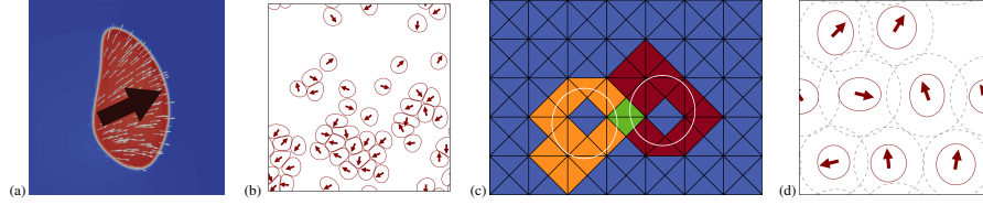
Figure 1. (a) Phase field variable \phi_i \approx 1 (red) cell bulk and \phi_i \approx -1 (blue) and polarisation field (white arrows) together with net polarisation (black arrow). (b) Evolution of 48 cells by cell activity. The arrows indicates the net polarisation of each cell. The cell boundaries \Gamma_i are the 0 level lines of the phase field variables. (c) The grid-elements of two overlapping interaction-regions are highlighted. (d) Cells with enclosing balls (dashed lines) defining neighbourhoods by overlap.
