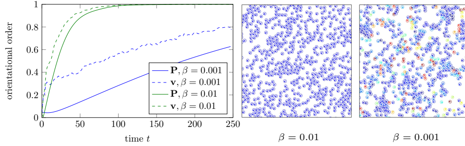
Figure 2. (left) Orientational order \theta for two different values of \beta simulated for N = 576 cells in setup-2. (centre) Configuration for \beta = 0.01 at time t = 200 . (right) Configuration for \beta = 0.001 at time t = 200 , different cell colours indicate different orientations.
