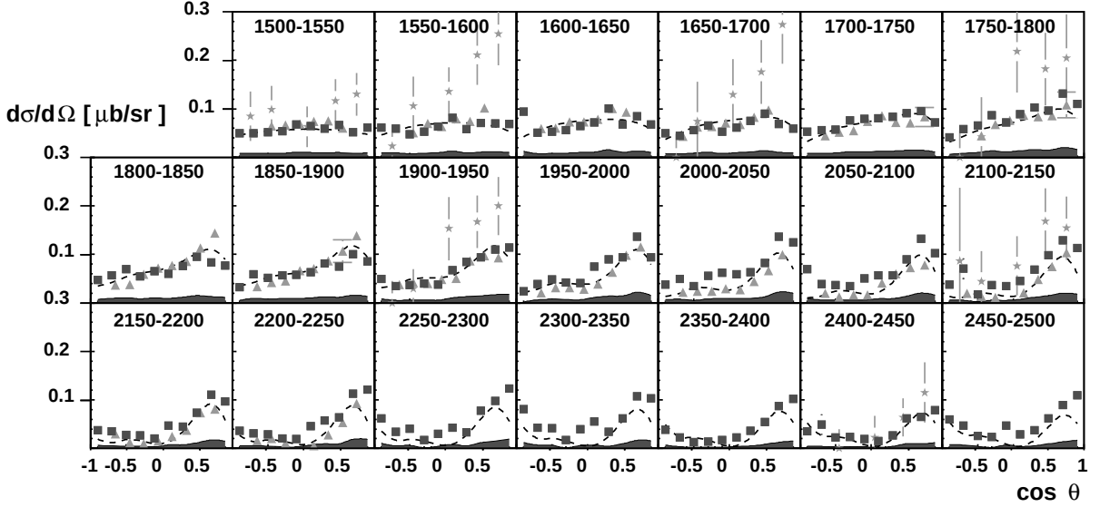
FIG. 10: Differential cross sections for the reaction \gamma p \rightarrow p\eta' \rightarrow 2\pi^0\eta \rightarrow p6\gamma (■) using 50-MeV wide energy bins and \cos\theta_{c.m.}^{\eta'} bins of width 0.2. The data cover the full angular range; energies are given in MeV. For comparison, data are shown from SAPHIR [27] (★) and CLAS [28] (▲). The SAPHIR data are based on only 250 events and thus, have large error bars. The dashed line represents the SAID model [39].
