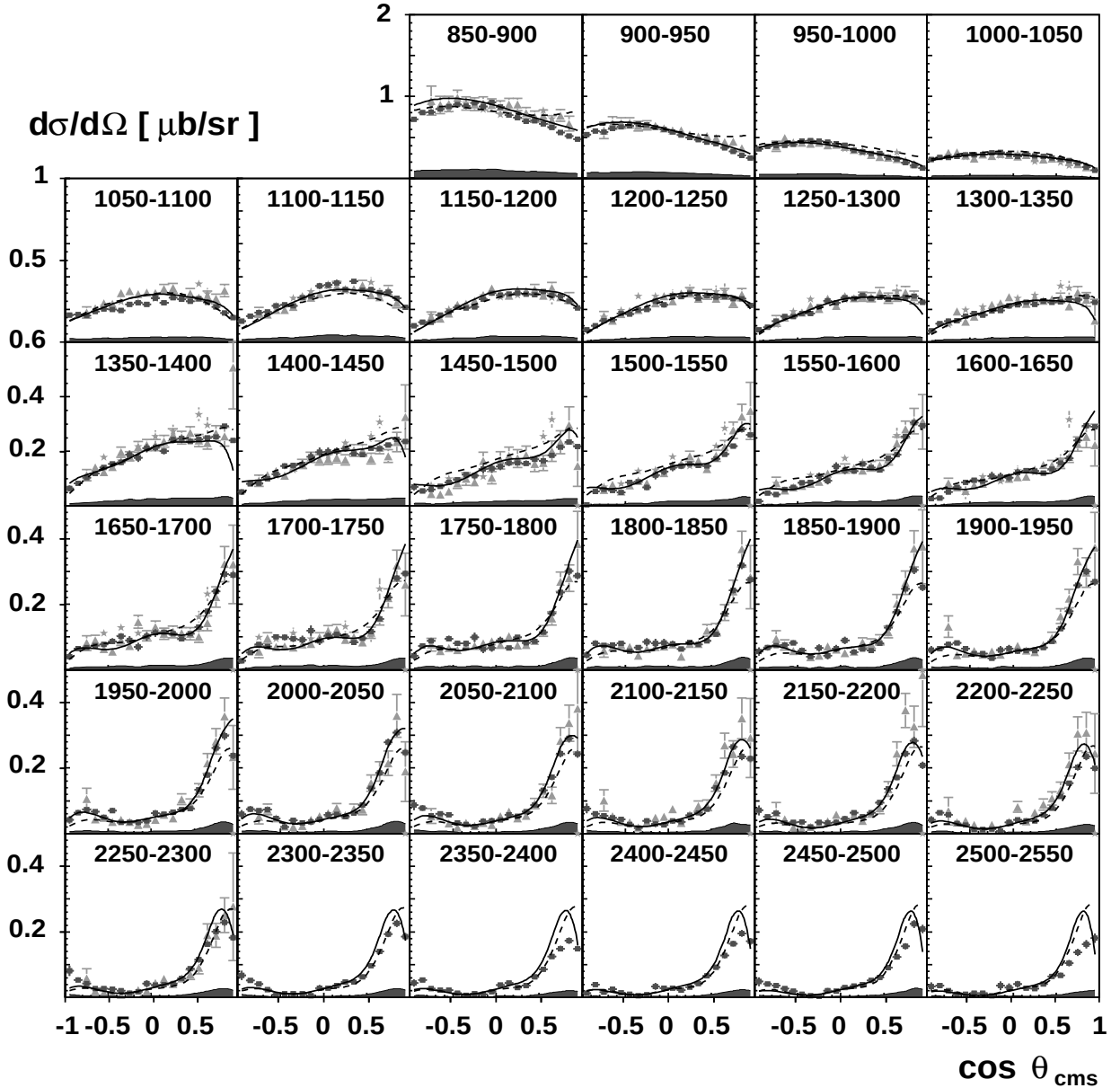
FIG. 9: Differential cross sections for \gamma p \rightarrow p\eta ( \blacksquare ) using the combined data set of \eta \rightarrow 2\gamma and \eta \rightarrow 3\pi^0 \rightarrow 6\gamma events. For comparison, CB-ELSA data [8] are represented by ( \blacktriangle ) and CLAS data by ( \star ). The solid line shows our previous PWA solution [8] and the dashed line represents the SAID model [39]. The data points include statistical errors only; the total systematic error is given as error bands at the bottom of each plot.
