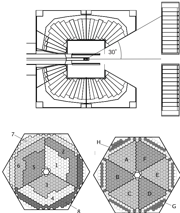
FIG. 2: Top: Schematic drawing of the liquid hydrogen target, scintillating-fibre detector, Crystal-Barrel and TAPS calorimeters. Bottom: Front view of TAPS; the left side shows the logical segmentation for the LED-low trigger, the right side the logical segmentation for the LED-high trigger (see text for more details).
