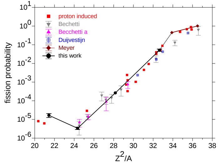
FIG. 5: (Color online) The fission probability as a function of the fissility parameter. The dots with error bars are the present results and diamonds are from Ref. [21]. The lines are to guide the eye. The squares are for proton-induced fission at energies 150 to 200 MeV [22, 23]. The other data shown were measured with 190 MeV protons: triangles down [24], triangles up [25], and those shown by crossed squares were measured by radiochemical methods [26].
