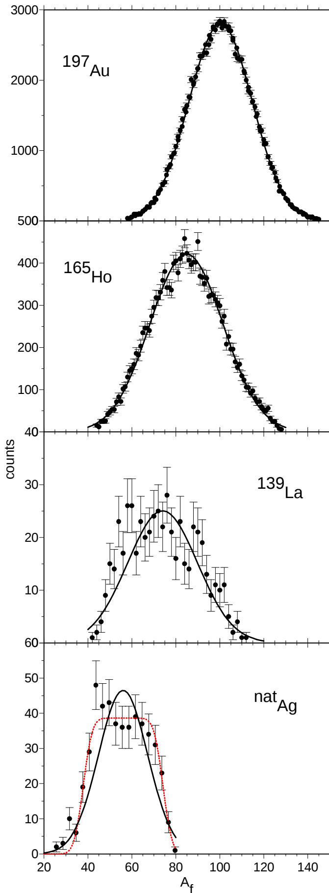
FIG. 3: (Color online) Fragment mass distributions for the four target nuclei studied. The data are shown as dots with error bars; fits with Gaussians are shown as solid curves. The fit with a symmetric double Gaussian cumulative in the case of ^{nat}\text{Ag} is shown as a dashed red line.
