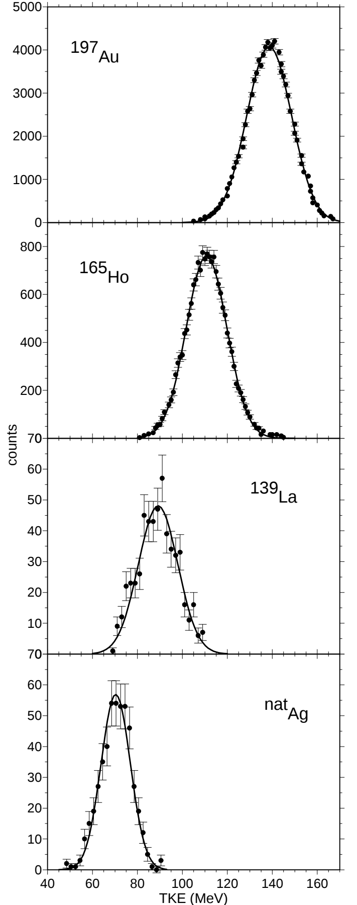
FIG. 2: Distributions of the total kinetic energy ( TKE ) for the four target nuclei studied. The data are shown as dots with error bars; fits with Gaussians are shown as solid curves.
