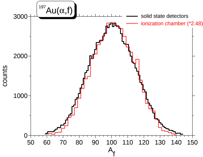
FIG. 1: (Color online) Comparison of the fragment distribution measured with two solid state detectors and one solid state detector and an ionization chamber.
