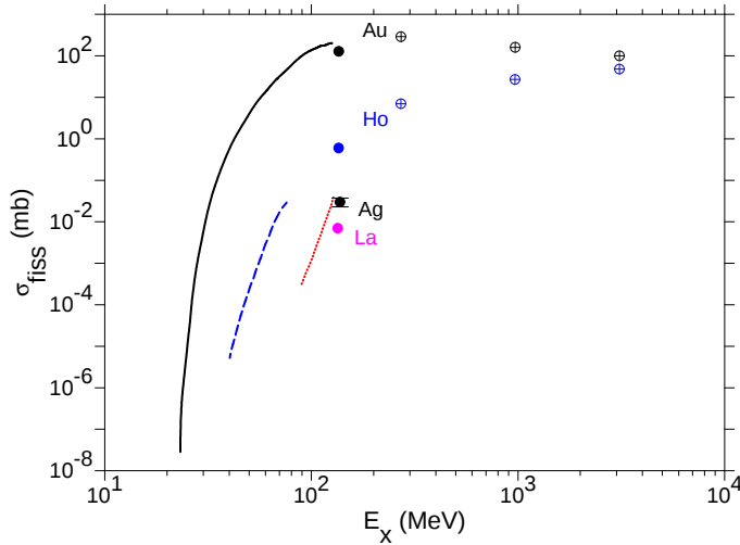
FIG. 4: (Color online) Excitation function for \alpha -particle induced fission. The present data are shown as full dots with error bars with the target nucleus being indicated. The curves are calculations from Moretto [19] for In (dotted), Tm (dashed) and Au (solid). The results from Ref. [20] for Au and Ho are shown by crossed circles.
