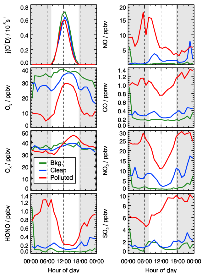
Figure 4. Mean diurnal profiles of measured photolysis frequencies ( j(\text{O}^1\text{D}) ) and concentrations of NO, CO, \text{O}_3 , \text{O}_x ( = \text{O}_3 + \text{NO}_2 ), \text{NO}_2 , HONO, and \text{SO}_2 for background (green), clean (blue), and polluted (red) episodes. The grey areas denote nighttime.
