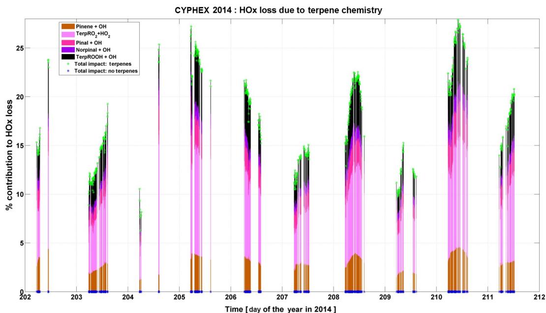
Figure 5. Contribution of different terpene-related reactions to the total \text{HO}_x loss. Additional peroxy radicals are produced in the model by terpenes rather than organics, e.g. isoprene degradation. Pinene includes \alpha -pinene and \beta -pinene. \text{TerpRO}_2 includes only \text{C}_8\text{H}_{13}\text{O}_3 (C85O2), \text{C}_8\text{H}_{13}\text{O}_4 (C86O2), \text{C}_9\text{H}_{15}\text{O}_3 (C96O2), \text{C}_9\text{H}_{15}\text{O}_4 (C97O2), \text{C}_9\text{H}_{15}\text{O}_5 (C98O2), \text{C}_{10}\text{H}_{15}\text{O}_5 (C106O2), \text{C}_5\text{H}_7\text{O}_4 (C511O2), \text{C}_6\text{H}_9\text{O}_5 (C614O2), \text{C}_{10}\text{H}_{15}\text{O}_4 (PinalO2), and \text{C}_{10}\text{H}_{17}\text{O}_3 (BPinaO2). \text{TerpROOH} includes only \text{C}_{10}\text{H}_{16}\text{O}_4 (PinalOOH), \text{C}_8\text{H}_{14}\text{O}_3 (C85OOH), \text{C}_8\text{H}_{14}\text{O}_4 (C86OOH), \text{C}_9\text{H}_{16}\text{O}_4 (C97OOH), \text{C}_9\text{H}_{16}\text{O}_5 (C98OOH), \text{C}_{10}\text{H}_{16}\text{O}_5 (C106OOH), and \text{C}_5\text{H}_8\text{O}_4 (C511OOH). The names in brackets are MCM nomenclature. Only those species are selected whose contribution is at least 0.25 % to the \text{HO}_x sink.
