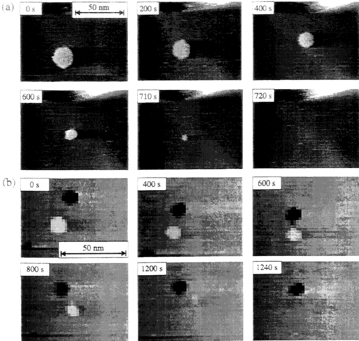
Abbildung 4.2: Adatominselzerfall: Monoatomare hohe Ag-Inseln; (a) Zerfallszeit \tau = 720 s; I_t = 5 nA; U_t = 0,5 V, RT; (b) \tau = 1240 s; I_t = 5 nA; U_t = 0,49 V, RT.
