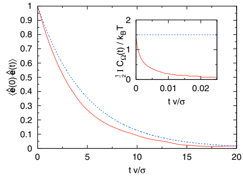
FIG. 2. (Color online) Orientation autocorrelation function \langle \hat{\mathbf{e}}(0) \cdot \hat{\mathbf{e}}(t) \rangle for a single squirmer, with Péclet number Pe=1155 . The full line shows the simulation data, while the dashed line corresponds to the theoretical result \exp(-2D_r t) . The inset shows the angular velocity autocorrelation function C_{\Omega}(t) = \langle \mathbf{\Omega}(0) \cdot \mathbf{\Omega}(t) \rangle . The dashed line represents the theoretical value at t=0 .
