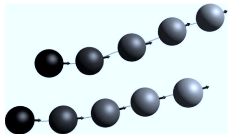
FIG. 11. Same as Fig. 8, but with an initial offset \Delta x=\sigma , \Delta z=2\sigma . The time interval is \Delta tv/\sigma=1.67 . Movies of the motion of interacting squirmer pairs are provided in Ref. [49].
