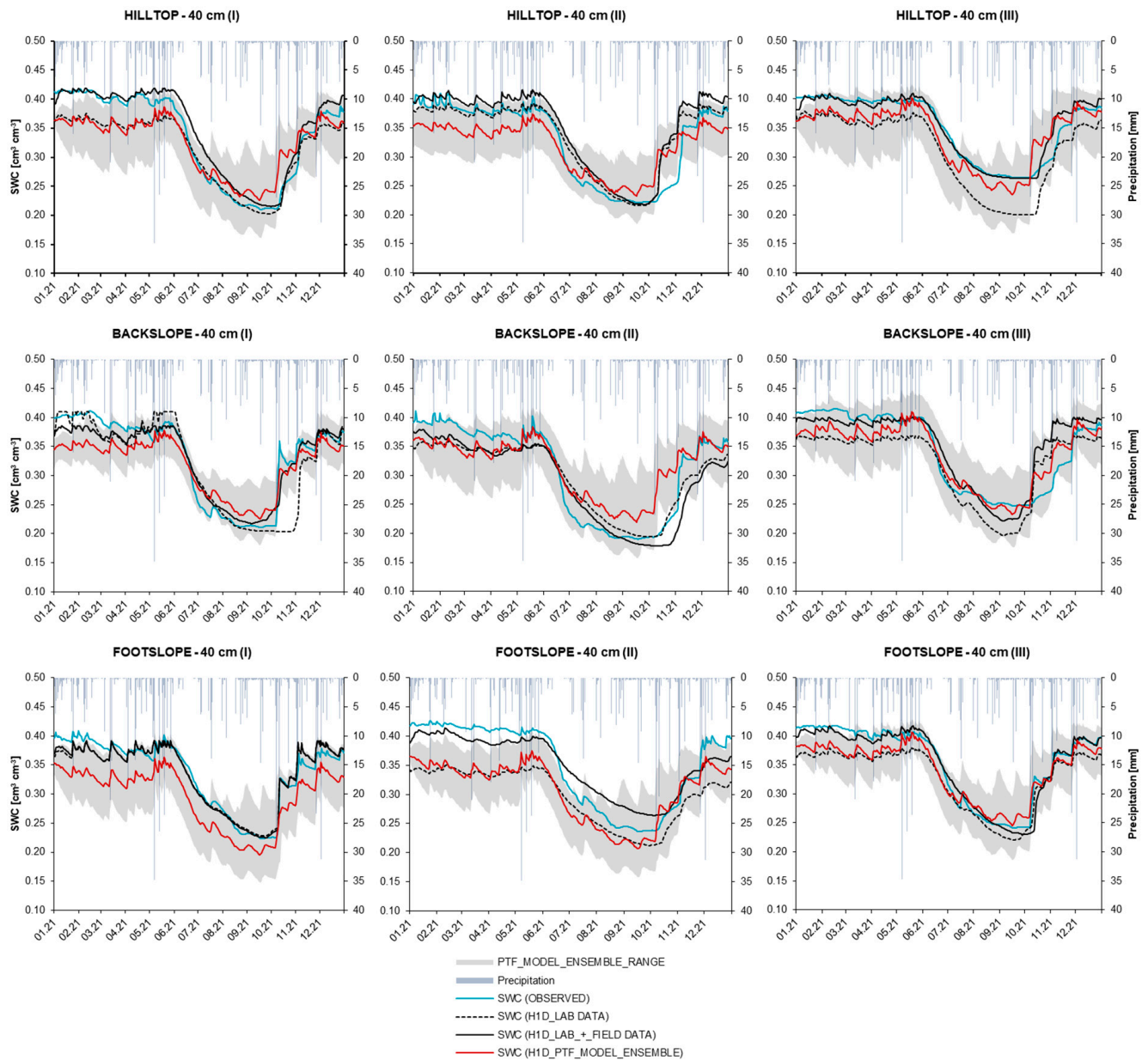
Figure 5. Simulated soil water content (SWC) [cm 3 cm -3 ] in HYDRUS-1D: pedotransfer (PTF) model ensemble (red line), PTF model ensemble spread (5–95 percentile range) (grey area), laboratory dataset (dashed black line) and combination of lab and field data (black line), and field SWC measurements (blue line) in three vineyard rows at 40 cm depth, with precipitation data obtained with weighing lysimeter in 2021 at the SUPREHILL Critical Zone Observatory.
