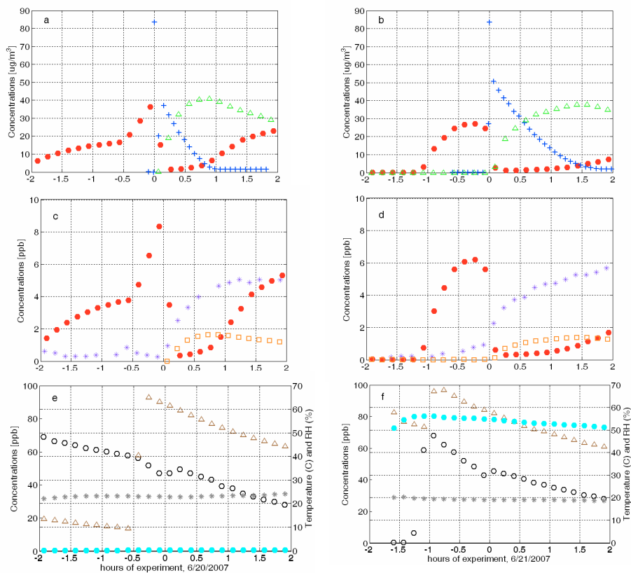
Fig. 1. Time evolution of \text{N}_2\text{O}_5 + \text{NO}_3 ( \bullet ) and \beta -pinene ( + ) mass concentrations and total particle mass loading ( \Delta ) [ \mu\text{g}/\text{m}^3 ] (not corrected for losses), during the dry ( a ) and humid ( b ) experiments; time evolution of \text{N}_2\text{O}_5 + \text{NO}_3 ( \bullet ), total alkyl nitrates ( * ) and aerosol nitrate ( \square ) concentrations [ppb], during the dry ( c ) and humid ( d ) experiments; and time evolution of \text{O}_3 ( \circ ) and \text{NO}_2 ( \Delta ) concentrations [ppb], temperature ( * ) [ ^\circ\text{C} ], and relative humidity ( \circ ) [%] during the dry ( e ) and humid ( f ) experiments.
