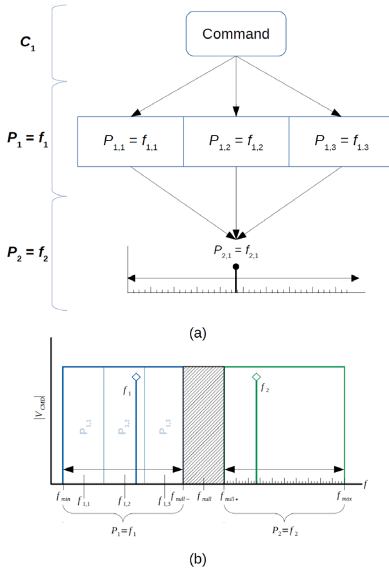
Figure 3. Example two-parameter command. Command tree (a) and frequency allocation graph (b) for each parameter.
