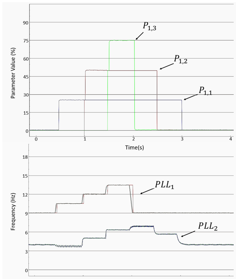
Figure 10. Results of the experiment: Assigning values to three sub-parameters (upper) and frequency detection by each PLL (lower).
