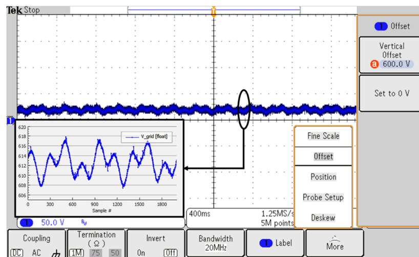
Figure 8. Oscilloscope screen capture of 600 V positive DC microgrid voltage rail.
