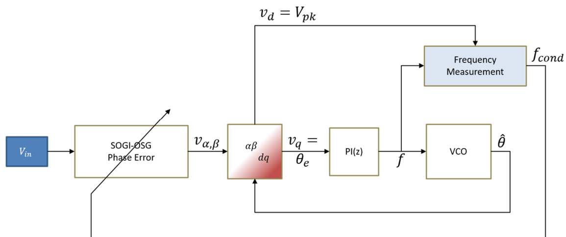
Figure 4. Block diagram of the second order generalized integrator (SOGI) phase locked loop (PLL) (SOGI-PLL).
