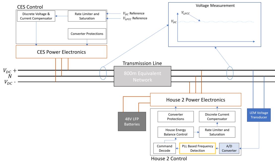
Figure 6. Live-scale DC microgrid experimental setup diagram.
