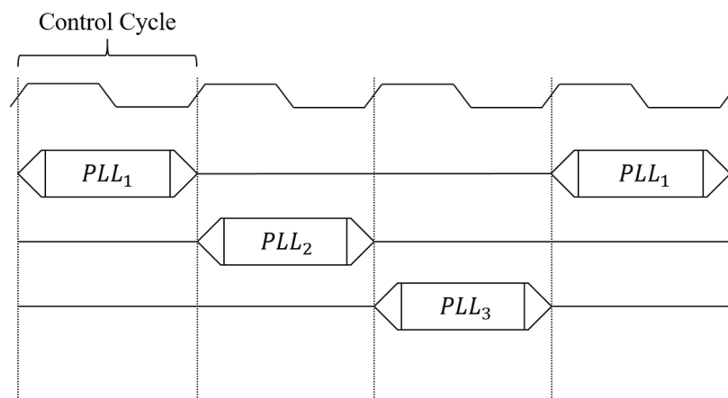
Figure 5. PLLs operated under the multiplexed detection scheme.
