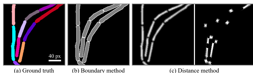
Fig 4. Training data representations of the two microbeSEG methods. From the ground truth (a – instances: color-coded), the boundary representation (b – cell interior: gray, cell boundary: white) and the distance representations (c – distance to background, inverse distance to neighbors) can be computed. A deep learning model is trained to predict either the boundary representation or the distance representations, and the single instances are recovered in the post-processing.
