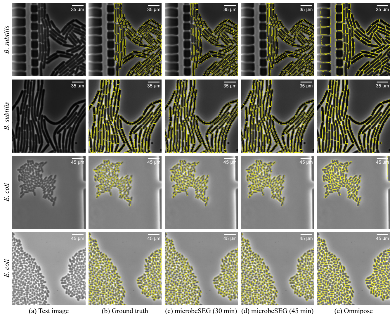
Fig 5. Exemplary images and segmentation overlays for B. subtilis and E. coli . Shown are the results of the median distance method microbeSEG models from Table 1.
