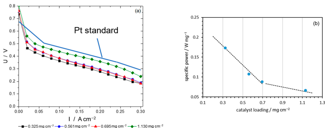
Figure 12. Polarization curves of MEAs with spray-deposited cathodes of different loadings with I/C of 0.5 and W/P of 56/44 (Methanol 0.8 mol L -1 ; sea level pressure; anode 3.0 mg cm -1 PtRu), Pt standard MEA with ~1.5 mg/cm 2 see also Figure 3 (a), specific power in W mg -1 catalyst over the catalyst loading in mg cm -2 at 225 mA/cm 2 (b).
