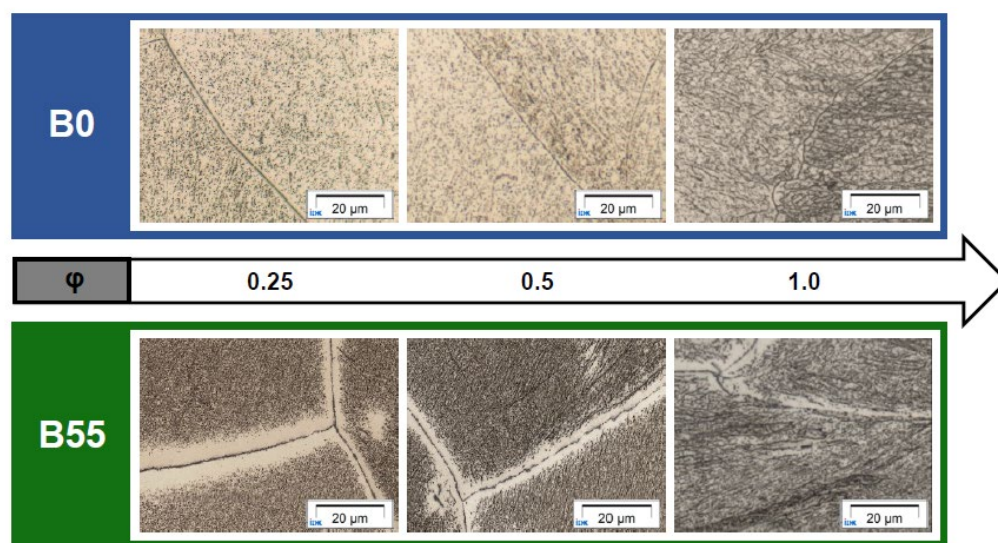
Figure 6. Impact of the deformation grade variation (0.25/0.5/1) at an 800 °C deformation temperature on precipitation in the reference B0 in comparison to the boron-alloyed B55 steel.
