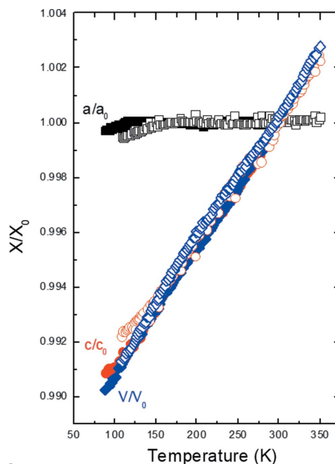
Figure 3 Normalized unit-cell parameters and unit-cell volumes to the values at 298 K as a function of temperature. The open and solid symbols are for \text{Rb}_2\text{V}_3\text{O}_8 and \text{K}_2\text{V}_3\text{O}_8 , respectively.
