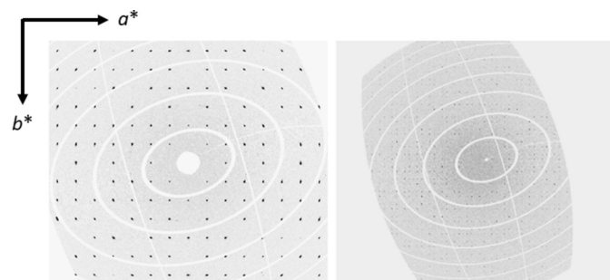
Figure 2 Reciprocal space sections hk0 (left) and hk0.5 (right) at 100 K.
