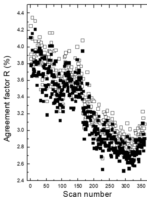
Figure 13 Agreement factors R_{\text{obs}} (full symbols) and R_{\text{all}} (open symbols) as a function of the scan number in \text{K}_2\text{V}_3\text{O}_8 at 100 K.
