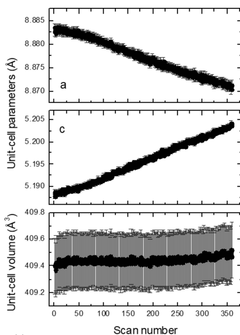
Figure 11 Unit-cell parameters and unit-cell volumes as a function of the scan number in \text{K}_2\text{V}_3\text{O}_8 at 100 K. Standard uncertainties of all the parameters are plotted in the figure.
