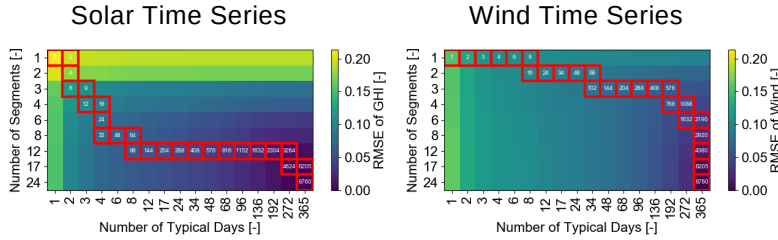
Figure 3.27. The proposed algorithm for the root-mean-square error (RMSE) of an exemplary global horizontal irradiance and a wind speed profile (taken from Hoffmann et al. [3])
