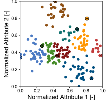
Figure 3.11. A clustered data cloud including the cluster's maxoids
