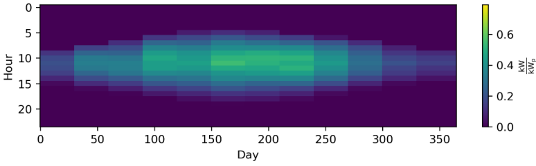
Figure 2.10. The time series of photovoltaic capacity factors represented by twelve monthly averaged periods as used in other studies [60, 104, 105] and reproduced by Kotzur et al. [48] using the python package tsam [48] (i.e., 288 different time steps) (RMSE=0.1126) (taken from Hoffmann et al. [1])
