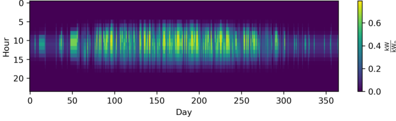
Figure 2.13. The time series of photovoltaic capacity factors represented by twelve typical days (typical days) using k -means clustering and the python package tsam [48] (i.e., 288 different time steps) (RMSE=0.0552) (taken from Hoffmann et al. [1])
