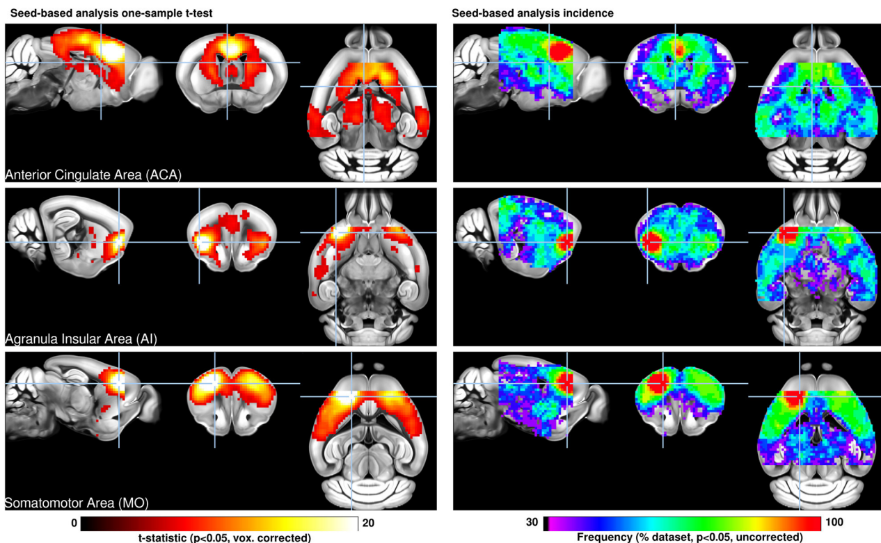
FIGURE 1 | Seed-based analysis (SBA) for three selected seeds positioned in the left hemisphere. One-sample t -test maps of individual functional connectivity maps reveal the full extent of SBA-derived resting-state networks in the mouse brain across 98 independent scans. Functional connectivity (FC) related to a seed located in the anterior cingulate area reveals the extent of the mouse default mode network including dorsal caudate-putamen, dorsal thalamus, and peri-hippocampal areas. The seed in the insular area reveals significant FC in dorsal cingulate and amygdalar areas, corresponding to areas associated with the human salience network. Interhemispheric homotopic FC is found relative to the somatomotor seed, together with lateral striatal FC. Overlap maps indicate the percentage of data sets presenting significant FC which recapitulate the features above. Reproduced with permission from Grandjean et al. (2020).
