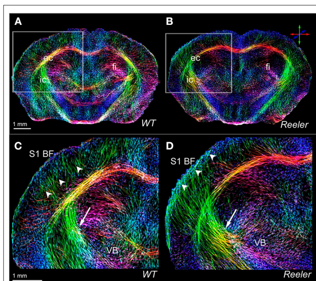
FIGURE 2 | High-resolution views of the thalamocortical fiber architecture of the wild-type and reeler mouse brain. In vivo high-resolution fiber maps of normal (A,C) and reeler (B,D) brain captures major features of normal (C) vs. remodeled (D) subcortical (arrows) and thalamocortical (arrow heads) fiber trajectories of the somatosensory thalamocortical pathway. The magnified views (C,D) illustrate the fiber bundles emerging from the ventrobasal thalamic nucleus (VB) to target S1BF (S1 barrel field); they cross the internal capsule (C,D, arrow) and gather beneath the cortical gray matter before extending intracortically up to presumptive layer IV of the wild-type S1BF (C, arrow heads). Note that the reeler thalamic fibers (D) are defasciculated to form a broader array projecting diagonally (D, arrow) into the cortical areas. Reproduced with permission from Harsan et al. (2013).
