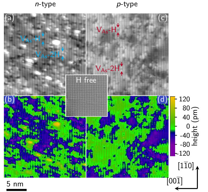
FIG. 1. Atomically resolved constant-current STM images of the (a,b) n - and (c,d) p -doped GaAs(110) surfaces after 0.5 L hydrogen exposure (acquired at set-points of V_s = -1.8 \text{ V} , I_T = 50 \text{ pA} and V_s = -2.0 \text{ V} , I_T = 50 \text{ pA} , respectively). (b) and (d) represent false color images of (a) and (c), respectively, illustrating a phase separation characterized by slightly lowered (blueish) and elevated (greenish) areas. The height difference between those areas is about 40 pm. Inset: Atomically resolved constant-current STM image of the GaAs(110) surface without hydrogen exposure. The arrows in (a) and (c) mark defects, further analyzed using height profiles in Fig. 2.
