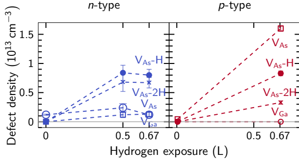
FIG. 3. Concentration of the various observed defects on (a) n -type and (b) p -type GaAs(110) vs. hydrogen exposure. The data at 0 L exposure corresponds to the hydrogen free cleavage surfaces, extracted from prior measurements.[27, 29]
