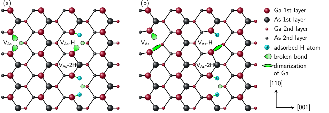
FIG. 5. Schematic illustrating the defect-molecule model discussion of the single As vacancy V_{\text{As}} as well as hydrogen vacancy defect complexes ( V_{\text{As}}\text{-H} and V_{\text{As}}\text{-2H} ). (a) Upon vacancy formation, three bonds are broken, leaving behind two broken bridge- and one broken back-bond. (b) The broken bonds rehybridize and form defect states and/or interact with one or more hydrogen atoms.
