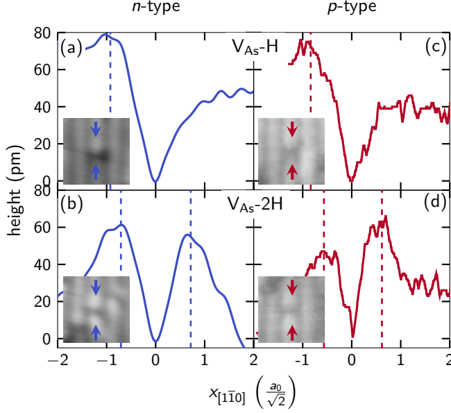
FIG. 2. Height profiles along the [1\bar{1}0] direction through the V_{As} -H (top) and V_{As} -2H (bottom) defects marked in Fig. 1 for (a,b) n - and (c,d) p -type GaAs(110) surfaces after hydrogen exposure. Dashed vertical lines mark the positions of the filled dangling bonds above the neighboring As atoms. For the V_{As} -2H defects, the profiles indicate an inward displacement of the neighboring As atoms. The insets illustrate STM images of the corresponding defects.
