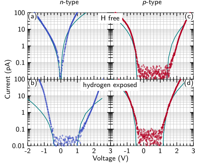
FIG. 4. Scanning tunneling current spectra of the n - (a,b) and p -type (c,d) GaAs(110) surfaces in the hydrogen free state (top) and after hydrogen exposure of (b) 0.5 L and (d) 0.67 L (bottom). The experimental data, shown as symbols, has been acquired at tip-sample separations fixed at set currents of 50 pA at (a,c,d) -1.4 V and (b) -1.2 V. Self-consistent simulations are illustrated as lines.
