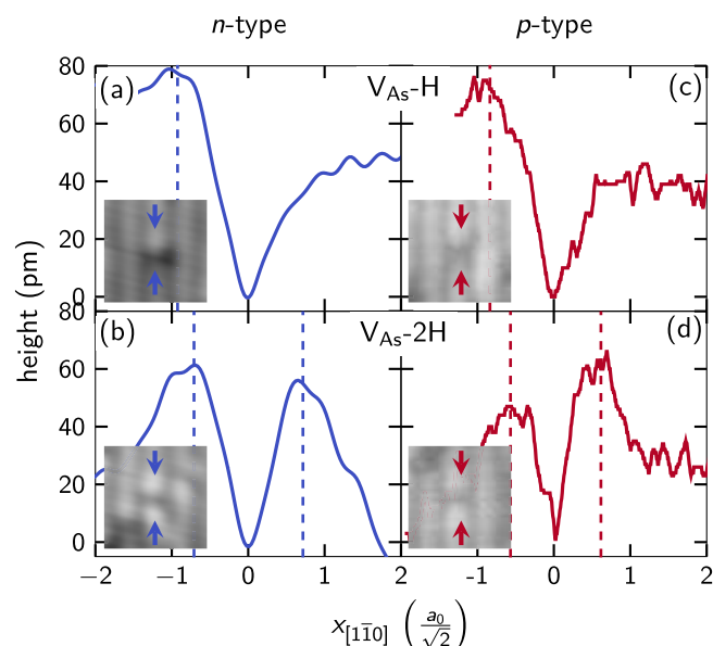
FIG. 2. Height profiles along the [1\bar{1}0] direction through the V_{\text{As}}\text{-H} (top) and V_{\text{As}}\text{-2H} (bottom) defects marked in Fig. 1 for (a), (b) n - and (c), (d) p -type GaAs(110) surfaces after hydrogen exposure. Dashed vertical lines mark the positions of the filled dangling bonds above the neighboring As atoms. For the V_{\text{As}}\text{-2H} defects, the profiles indicate an inward displacement of the neighboring As atoms. The insets illustrate STM images of the corresponding defects.
