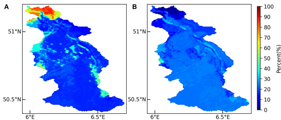
FIGURE 2 Sand (A) and clay (B) content (%) for the Rur catchment derived from the BK50 soil map.
