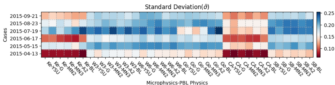
Figure 17. Heat map of the ensemble standard deviation ( \bar{\sigma} ) of the mean total cloud fraction, averaged over the last 36 h of the simulations, shown for each cluster of microphysics and PBL physics (columns) for all test cases (rows). In this heat map, blue indicates larger \bar{\sigma} and greater ensemble spread.
