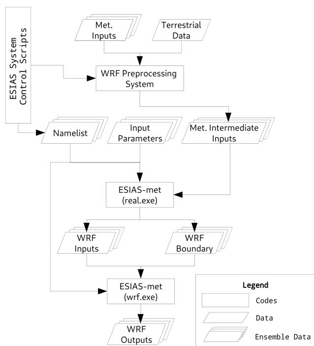
Figure 1. The concept of ESIAS-met scheme and the whole process of ESIAS-met. The ESIAS system control scripts control the WRF preprocessing system and the namelist to generate necessary inputs.
