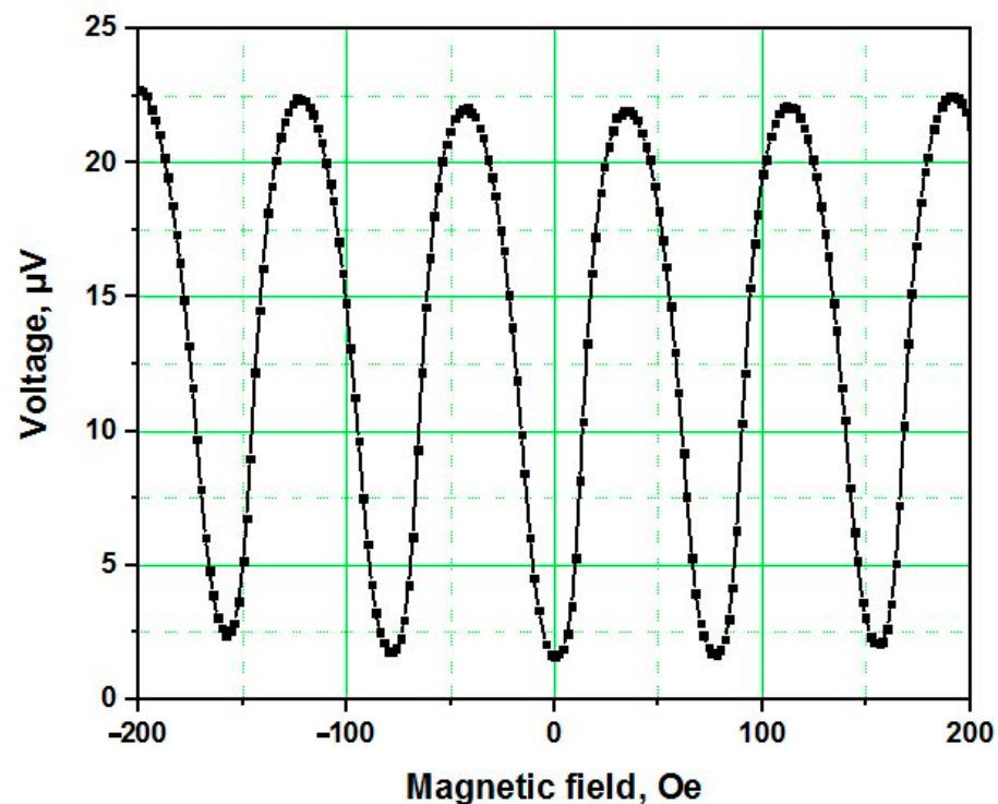
Figure 2. V(B) -characteristic of a planar nanoSQUID with TiN-NbN-TiN nJJs measured using a QD PPMS with a bias current of 12 \mu\text{A} at 5 K.
