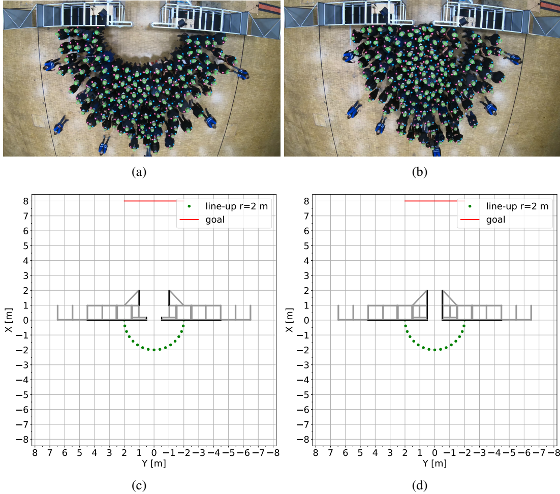
Figure 13 Snapshots of experiments with 0.2 m bottleneck length and an initial line-up being a) a 2 m semi-circle and b) standing directly at the bottleneck. Schematics of a setup with a bottleneck length of c) 0.2 m and d) 2 m.
