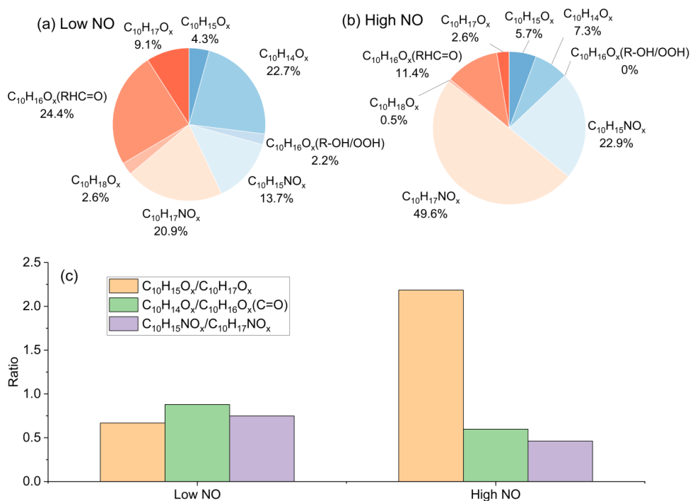
Figure 3. Product distribution within C_{10} monomers at low (a) and high NO (b) and the ratio of C_{10}H_{15}O_x^\bullet to C_{10}H_{17}O_x^\bullet and of their termination products (c). As in Fig.2, data of the first 60 min of the experiments were used.
