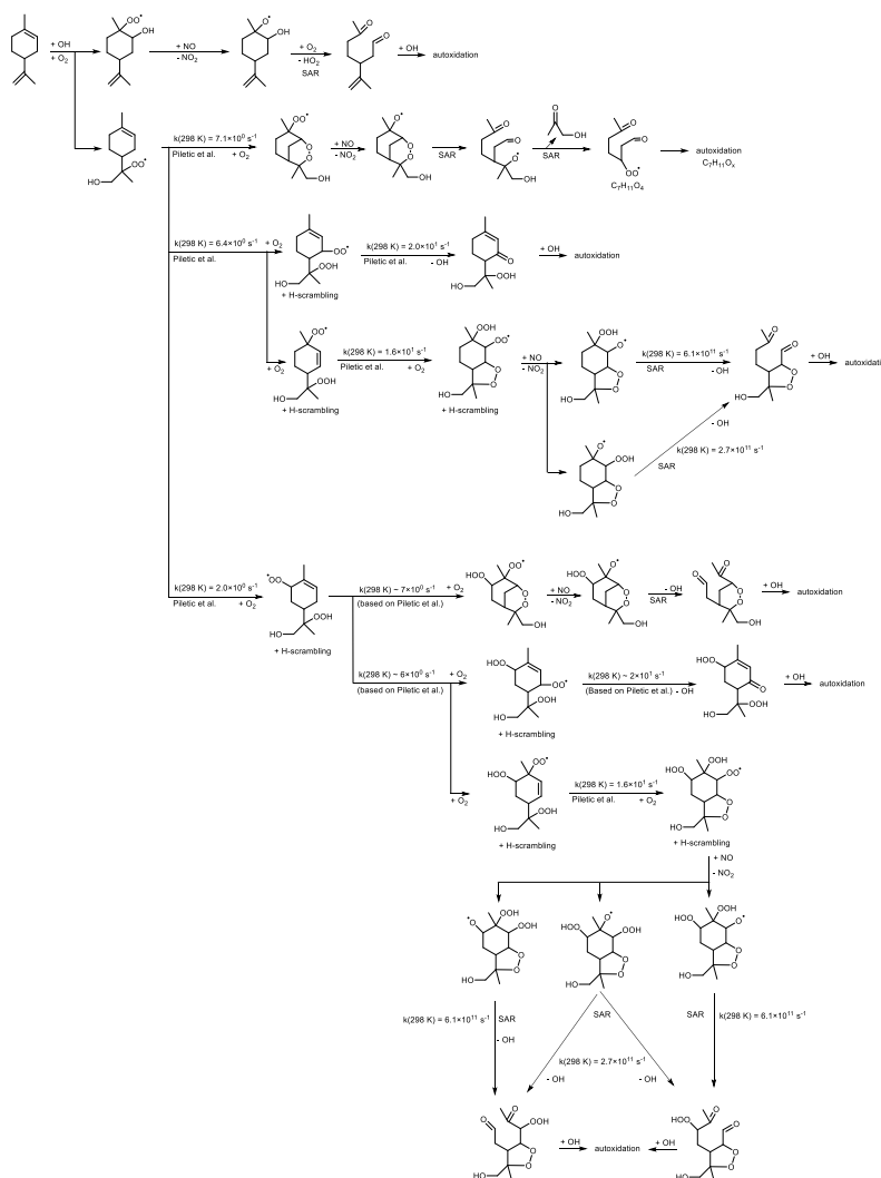
Scheme 1. Example reaction scheme for \text{C}_{10}\text{H}_{17}\text{O}_x \text{RO}_2 formation after \text{OH} -addition in limonene, based on the most likely reactions predicted in theoretical work and SAR predictions. All \text{RO}_2 intermediates have competing reactions (not shown) under current conditions with \text{HO}_2 (forming hydroperoxides) and \text{NO} (forming alkoxy and nitrates). 335
