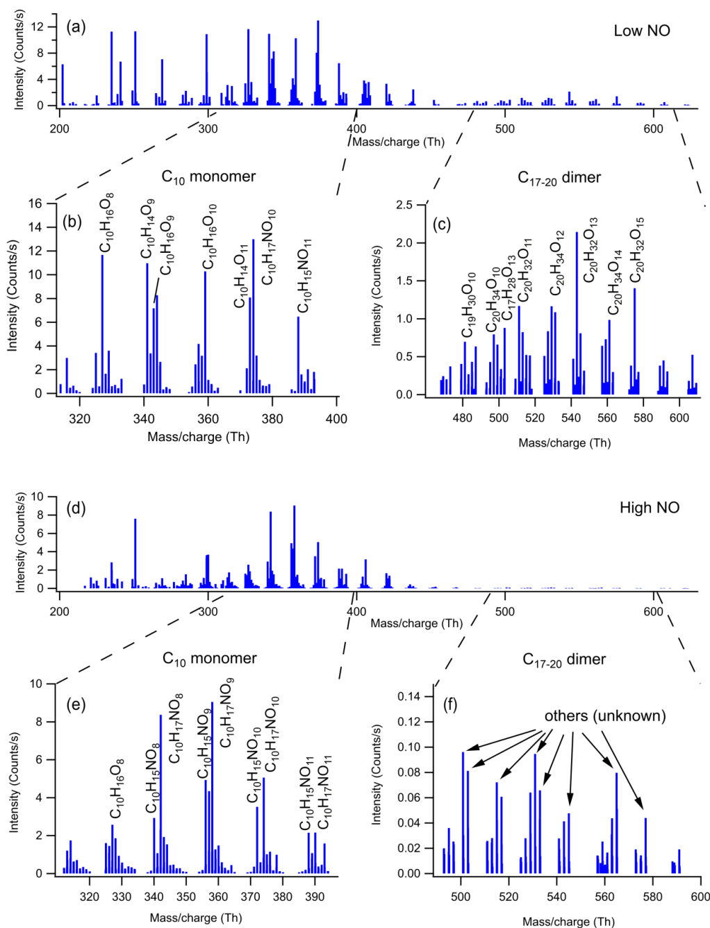
Figure 1. Mass spectrum of the HOM formed in the oxidation of limonene by OH in (a) low and (d) high NO condition. The mass spectra were obtained within 60 min after opening the louvres and were averaged over 60 min.. Figure 1 (b, c, e, f) present expanded mass spectra where major peaks are labelled with their molecular formula.
