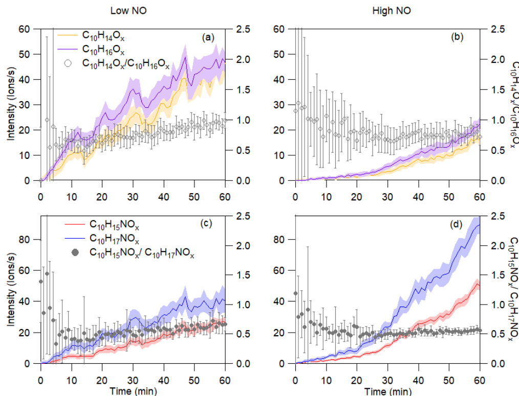
Figure 4. Time series of C_{10}H_{15}O_x • and C_{10}H_{17}O_x • related families of carbonyls and organic nitrates during the first 60 min of the experiments. The carbonyl families C_{10}H_{14}O_x (yellow), C_{10}H_{16}O_x (purple), and their concentration ratio ( C_{10}H_{14}O_x / C_{10}H_{16}O_x ) are shown for (a) low and (b) high NO experiments. Time series for organic nitrate families C_{10}H_{15}NO_x (red) and C_{10}H_{17}NO_x (blue), and concentration ratio of C_{10}H_{15}NO_x / C_{10}H_{17}NO_x , are similarly demonstrated in (c) for low NO and (d) high NO experiments. All data are averaged to 1 min and the error bar represents one standard deviation.
