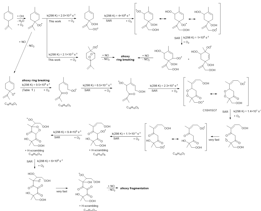
Scheme 2. Example reaction scheme for HOM formation after H-abstraction in limonene, based mostly on SAR prediction and starting at the fastest of 5 allylic H-abstraction sites. Direct autoxidation of the nascent RO 2 is slow, k \sim 10^{-2} \text{ s}^{-1} , and formation of an alkoxy radical is to be expected immediately or after very few autoxidation steps, especially in high NO conditions. Once the ring structure is broken, fast autoxidation steps are accessible. All RO 2 intermediates have competing reactions (not shown) under current conditions with HO 2 (forming hydroperoxides) and NO (forming alkoxy radicals and nitrates). Alkoxy radicals formed thus can fragment, or continue autoxidation after ring breaking or fast migration of an hydroperoxide H-atom, forming a wider variety of HOM.
