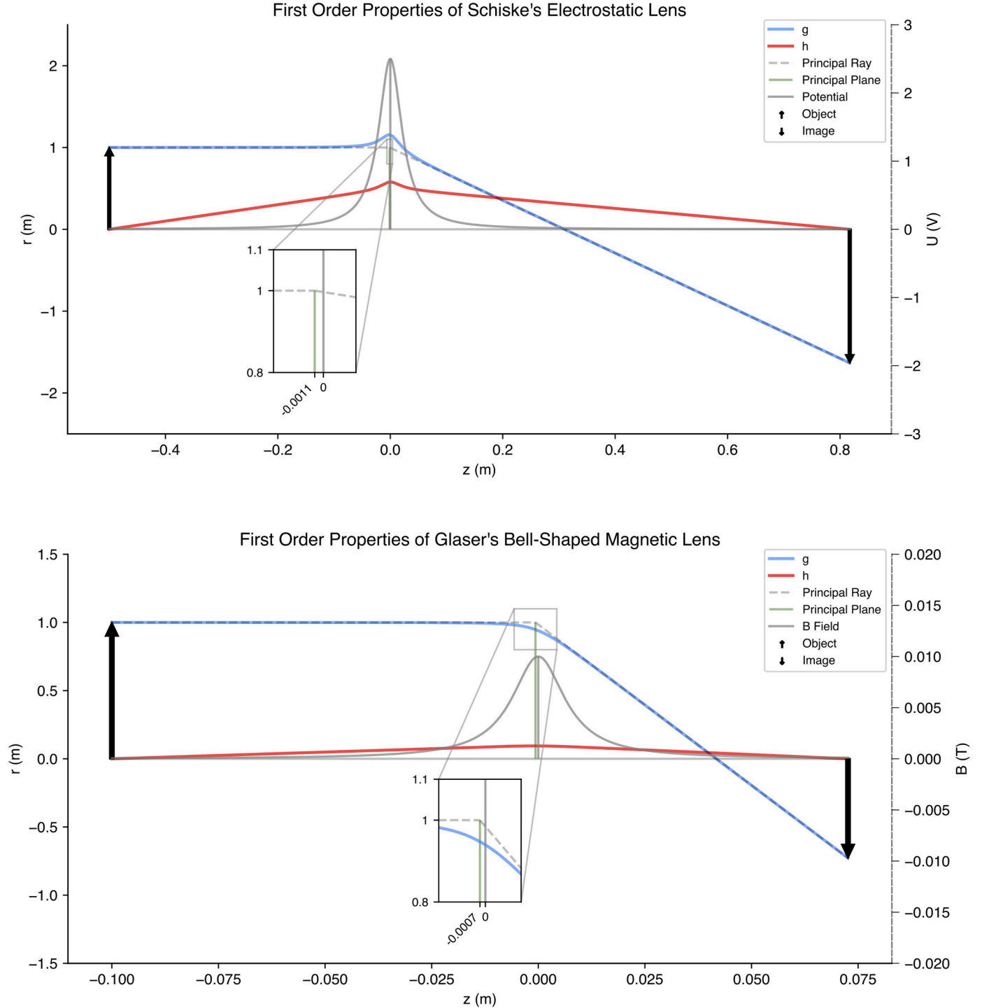
Fig. 1. Linearised ODE solutions to Schiske's Electrostatic Lens & Glaser's Bell Shaped Field. Shown are the rays g (blue) and h (red) and how the object (black up arrow) is imaged (black down arrow) by the lens. The inset shows the principal image plane (where the ray appears to come from) and its location behind the lens.
