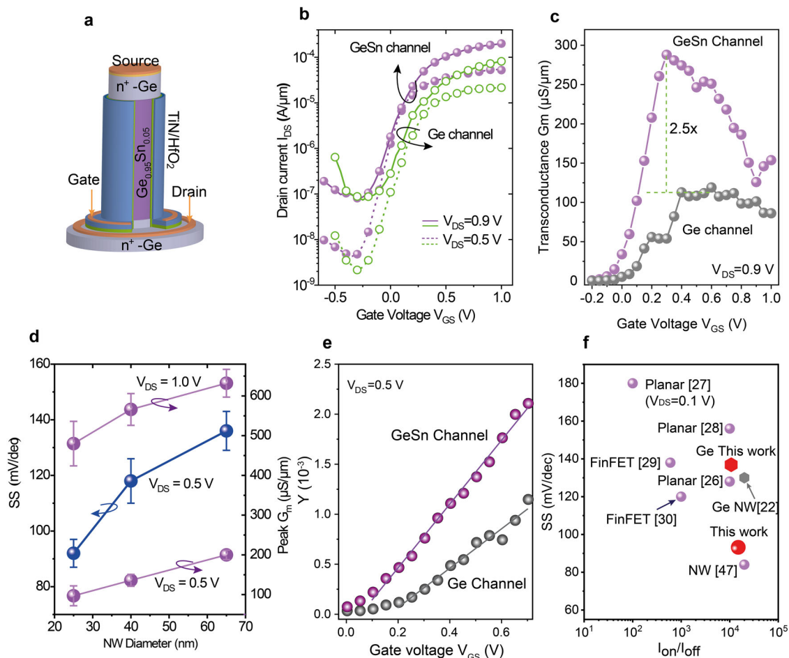
Fig. 4 Electrical performance of vertical Ge/GeSn/Ge gate-all-around (GAA) nanowire (NW) n-FET. a Schematic of an n-VFET with a \text{Ge}_{0.95}\text{Sn}_{0.05} channel and Ge source and drain. b I_D - V_{GS} transfer characteristics for a \text{Ge}/\text{Ge}_{0.95}\text{Sn}_{0.05}/\text{Ge} n-VFET in comparison with a Ge homojunction n-VFET, both with an NW diameter of 25 nm. c 2.5 times higher transconductance, G_m , for GeSn channel n-VFET compared to the Ge n-VFET. d Subthreshold swing (SS) measured at V_{DS} = 0.5 V and peak G_m values as a function of NW diameter, showing improved SS and degraded G_m with decreasing NW diameter. The error bars represent the standard deviations of the measured data from 15 transistors. e Plots of the Y-function for the mobility calculation. f SS benchmarking of current n-VFETs with state-of-the-art GeSn n-FETs, mostly taken at V_{DS} = 0.5 V with the exception of the data in ref. 27 which was given at V_{DS} = 0.1 V.
