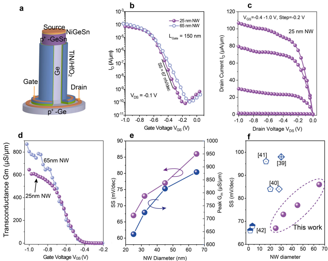
Fig. 3 Electrical performance of vertical GeSn/Ge Gate-all-around (GAA) nanowire (NW) p-FETs. a Schematic of a vertical p-FET (p-VFET) with \text{Ge}_{0.95}\text{Sn}_{0.05} source and Ge channel. b I_D - V_{GS} transfer characteristics for a p-VFET with NW diameters of 25 nm and 65 nm. c I_D - V_{DS} output characteristics for a 25 nm NW diameter p-VFET, showing very good saturation. d Transconductance G_m of p-VFETs with NW diameters of 65 nm and 25 nm. e Subthreshold swing (SS) and peak G_m as a function of NW diameter. The SS improves and the G_m decreases for smaller NW diameters because of the increased top NW contact resistance. f Benchmarking of current GeSn p-VFETs with state-of-the-art published GeSn NW p-FETs in terms of the subthreshold swing SS.
