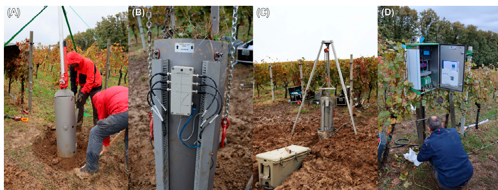
Figure 3. Installation procedure of the high-precision weighing lysimeter system at the SUPREHILL CZO: (A) vertical downpress of the cylinder during excavation; (B) connection of the sensors and system parts; (C) lowering of the cylinders below ground level and placement of the drainage tank (field box); (D) installation of the central control unit.
