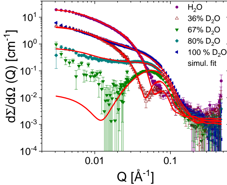
Figure 7: Contrast variation SANS analysis of the PEG-K 3 W(QL) 6 K 2 nanofibers showing the scattering curves at five different H 2 O/D 2 O contrasts where various part of the structure is highlighted. The solid lines corresponds to a simultaneous fit of all scattering curves using the model described in the text
