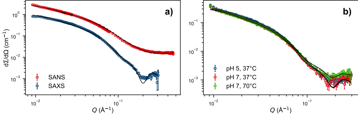
Figure 3: Small-angle scattering curves of K 3 W(QL) 6 K 2 , black lines are model fits. a) The same 10 mg/mL peptide sample in pH 7.4 Tris buffer, measured with SAXS and SANS (100 % D 2 O) at 25 °C. Both curves were fitted with the same set of parameters, see Table 1. b) SAXS curves of the K 3 W(QL) 6 K 2 in pH 7.4 Tris buffer and pH 5.0 MES buffer, at 37 and 70 °C.
