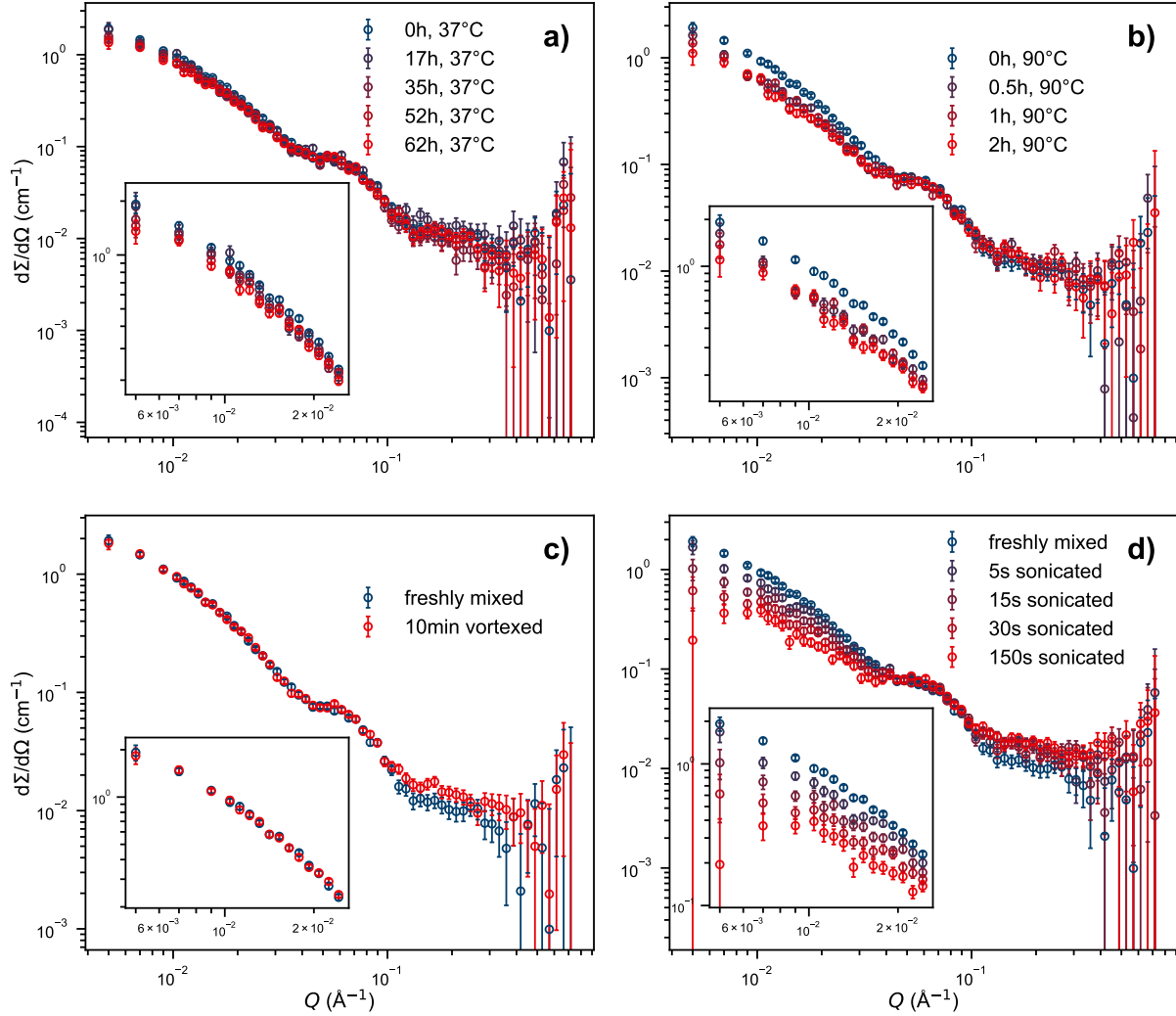
Figure 8: Neutron scattering data of blends of deuterated and protonated PEG-K 3 W(QL) 6 K 2 in a zero-average-contrast Tris buffer (pH 7.4 @25 °C, 56% D 2 O). Molecular exchange is visible as a decrease in scattering intensity. The insets are magnifications of the low- Q region. a) Thermally activated exchange at 37 °C. b) Thermally activated exchange after storing the blended sample in an oven at 90 °C for the indicated duration. c) Mechanically activated exchange using a bench-top vortex mixer. d) Mechanically activated exchange using a tip-sonicator.
