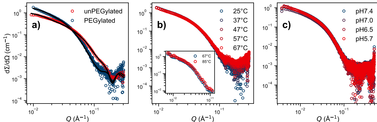
Figure 6: a) Scattering curves of K_3W(QL)_6K_2 and PEG- K_3W(QL)_6K_2 at 25 °C. Black lines represent a simultaneous fit of both datasets. b) Temperature stability of PEG- K_3W(QL)_6K_2 fibers: SAXS curves at 25-67 °C and (inset) SANS curves at 67 and 85 °C. c) SAXS curves of PEG- K_3W(QL)_6K_2 in BisTris buffer solution at different pH.
