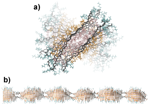
Figure 4: a) Cross-section view of the non-PEGylated K_3W(QL)_6K_2 peptide fiber, where the peptide backbone is black, tryptophan is grey, lysine is teal, glutamine is orange and leucine is pink. b) A representative snapshot of the whole peptide fiber after 15 ns equilibration.
