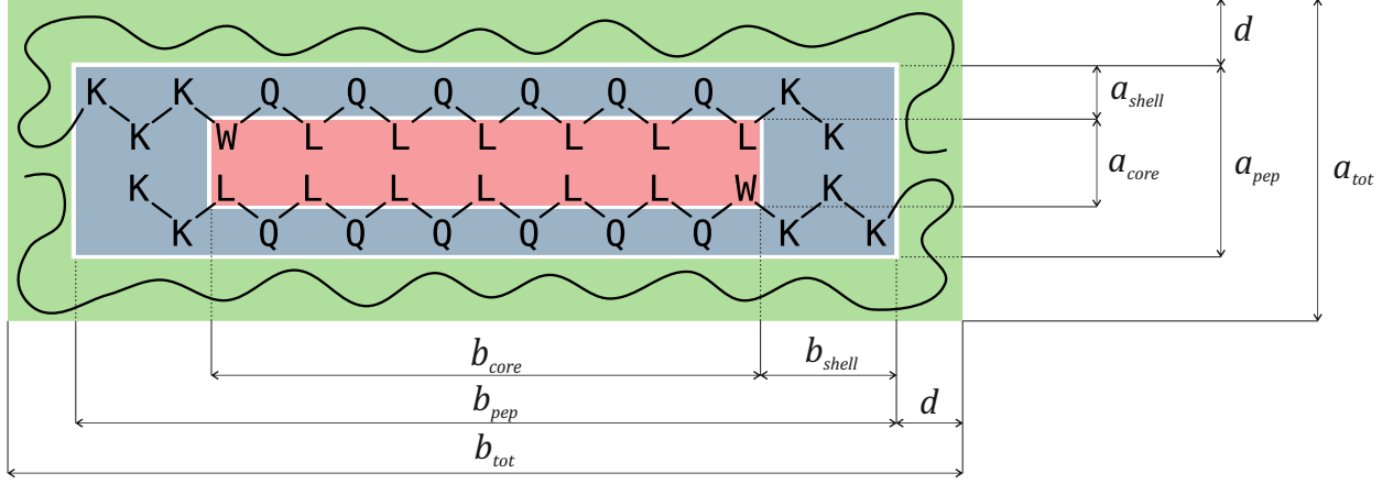
Figure 2: Sketch to illustrate the cross-section of the peptide scattering model. The core (red) is formed by the hydrophobic residues which are shielded from the solvent by the peptide backbone and the hydrophilic residues (blue). In case of the PEGylated peptide, PEG presumably forms a second, solvent-swollen shell around the peptide (green).
