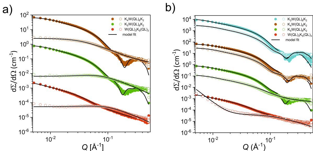
Figure 5: a) SAXS curves of the K_4W(QL)_6K_2 , K_5W(QL)_6K_2 and W(QL)_3K_5(QL)_3 peptides at the concentration 5mg/ml in pH 7.4 Tris buffer (filled circles) and in pH 5 MES buffer (open circles), black lines represent model fits. To avoid overlapping, intensity of K_4W(QL)_6K_2 was multiplied by 100 and intensity of W(QL)_3K_5(QL)_3 by 0.01. b) SAXS curves of the K_3W(QL)_6K_2 , K_4W(QL)_6K_2 , K_5W(QL)_6K_2 and W(QL)_3K_5(QL)_3 peptides at the concentration 5mg/ml in pH 7.4 Tris buffer (filled dots) and 5mg/ml solutions of peptides containing 4M urea (hallow dots), black lines represent model fit. To avoid overlapping, intensity of K_3W(QL)_6K_2 was multiplied by 10000, intensity of K_4W(QL)_6K_2 by 100 and intensity of W(QL)_3K_5(QL)_3 by 0.01. In graphs, every third data point is displayed.
