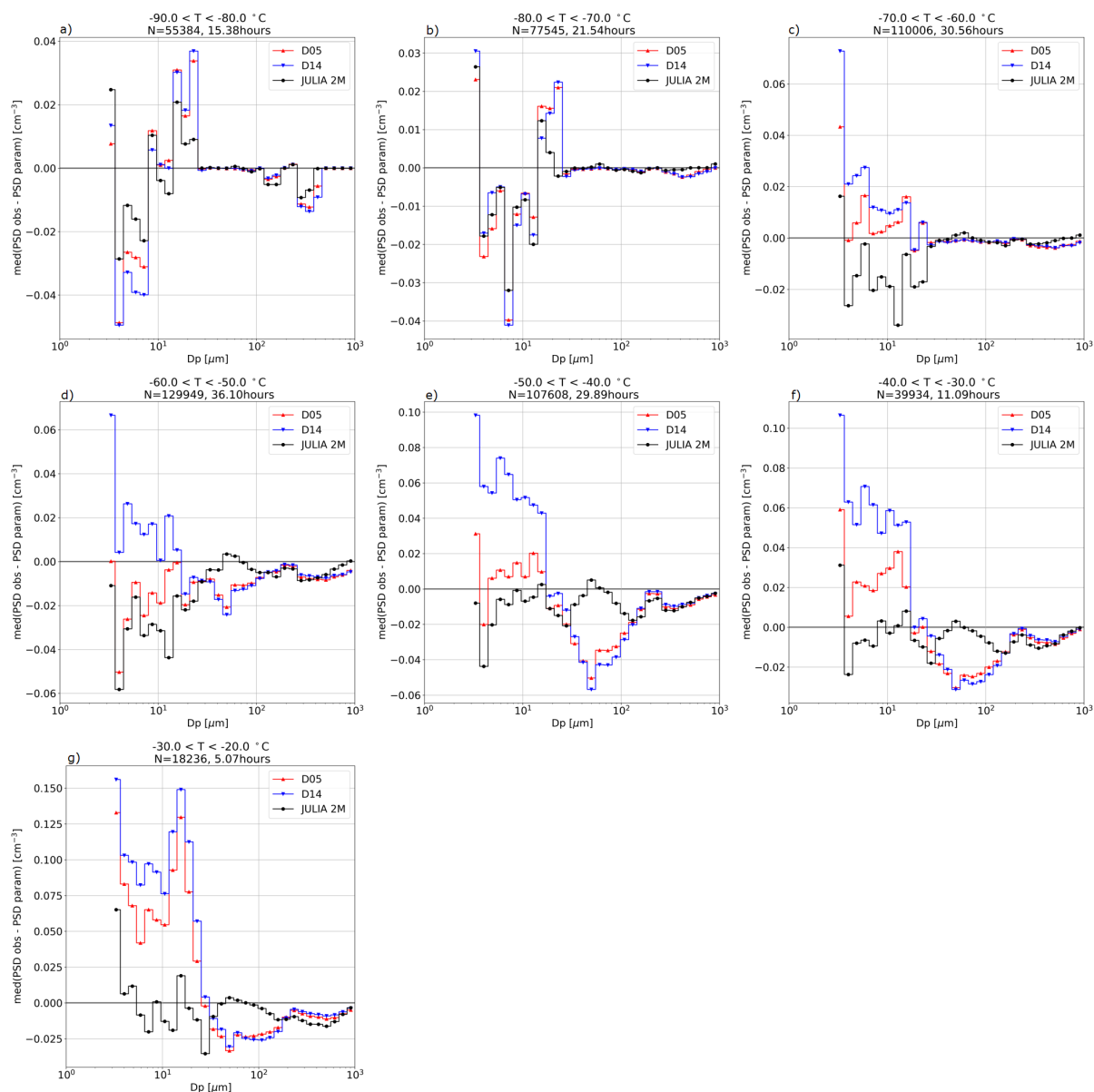
Figure 5. Median of the difference between the single observed PSDs of all campaigns and their corresponding parametrized PSDs, as in Fig. 4c, but for 10K temperature ranges. The parameterizations from the literature are: D05 in red and D14 in blue. JULIA 2M (in black) is the proposed new bimodal parameterization. y-axis is the median of the difference in number concentration between the observed and the parametrized PSDs in \text{cm}^{-3} and the x-axis is the size bins in \mu\text{m} . A detailed overview of the coefficients of each parameterization is given in Table 3.
