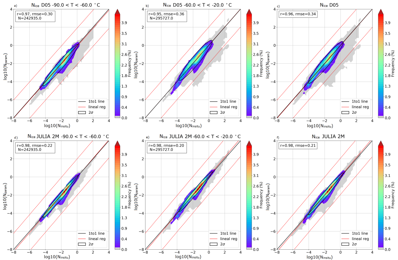
Figure 6. Comparison between the in-situ N_{ice} and parameterized N_{ice} for temperatures between -90^{\circ}\text{C} and -60^{\circ}\text{C} (a) D05, (d) JULIA 2M), temperatures between -60^{\circ}\text{C} and -20^{\circ}\text{C} (b) D05, (e) JULIA 2M) and temperatures lower than 255 K (c) D05, (f) JULIA 2M). The y-axis is the logarithm of the parameterized variable and the x-axis the logarithm of the observed one. Color code indicates frequency (%). The black line corresponds to the 1 to 1 line, the solid red line to the regression line and the dashed red lines to the regression line shifted a factor of \pm 2 . The black ellipse is the 2\sigma area. A detailed overview of the coefficients of each parameterization is given in Table 3.
