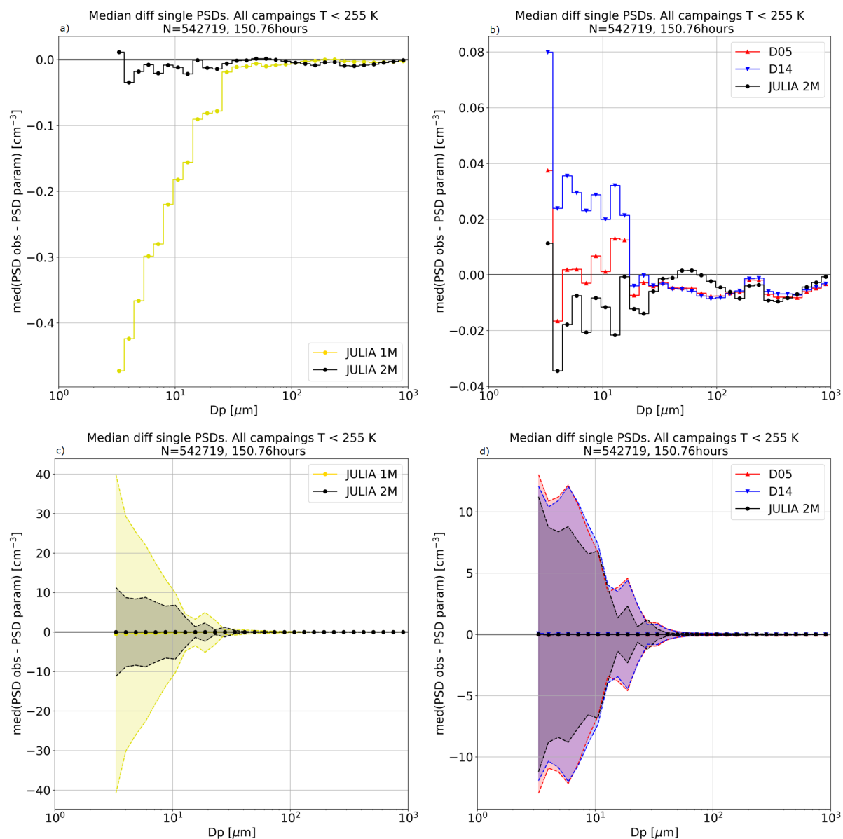
Figure 4. Median of the difference between the single parameterized PSDs and their corresponding observed PSDs. (a, c) Comparison between one mode (JULIA 1M: yellow) and two mode parameterization (JULIA 2M: black); (b, d) comparison between parameterizations from the literature (D05: red, D14: blue) and the two-modes parameterization (JULIA 2M: black) of this study. The shadow region in the lower panels correspond to 1\sigma . y-axis is the median of the difference in number concentration between the observed (from JULIA database) and the parameterized PSDs in \text{cm}^{-3} and the x-axis represent the size bins in \mu\text{m} . A detailed overview of the coefficients of each parameterization is given in Table 3.
