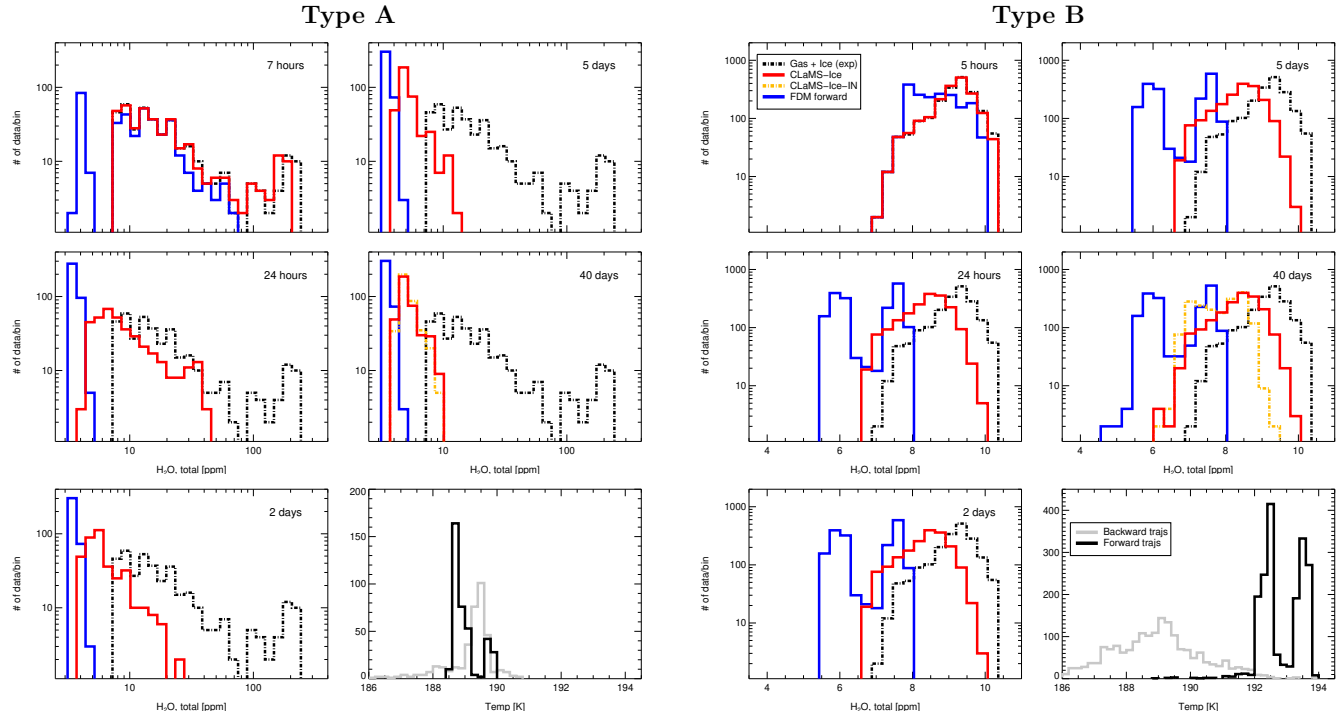
Figure 3. Time evolution of the total H 2 O frequency distribution (number of data points per bin) starting from two in situ observed distributions (left/right, type A/B, dashed black) as derived from forward trajectory calculations using CLaMS-Ice (red), FDM-forward (blue), and from CLaMS-Ice with artificially enhanced heterogeneous ice nucleation (CLaMS-Ice-IN, orange); the latter is shown only 40 days after the initialization. For a better comparison, the initial frequency distribution is shown for all time steps (dashed black). Note that a logarithmic x-axis was applied for type A to take into account the large amount of ice used for initialization, while a simple linear x-axis was used for type B. The contribution of the dehydration driven by the parameterized gravity waves temperature fluctuations is very weak, as estimated from the small difference between the type B CLaMS-Ice distributions after 5 versus after 40 days (this difference vanishes if this parameterization is switched off). The 40-day distributions also show the impact of enhanced ice nucleation by using CLaMS-Ice-IN. The respective last panels show the frequency distribution of the LDP temperatures for the back and forward trajectories.
