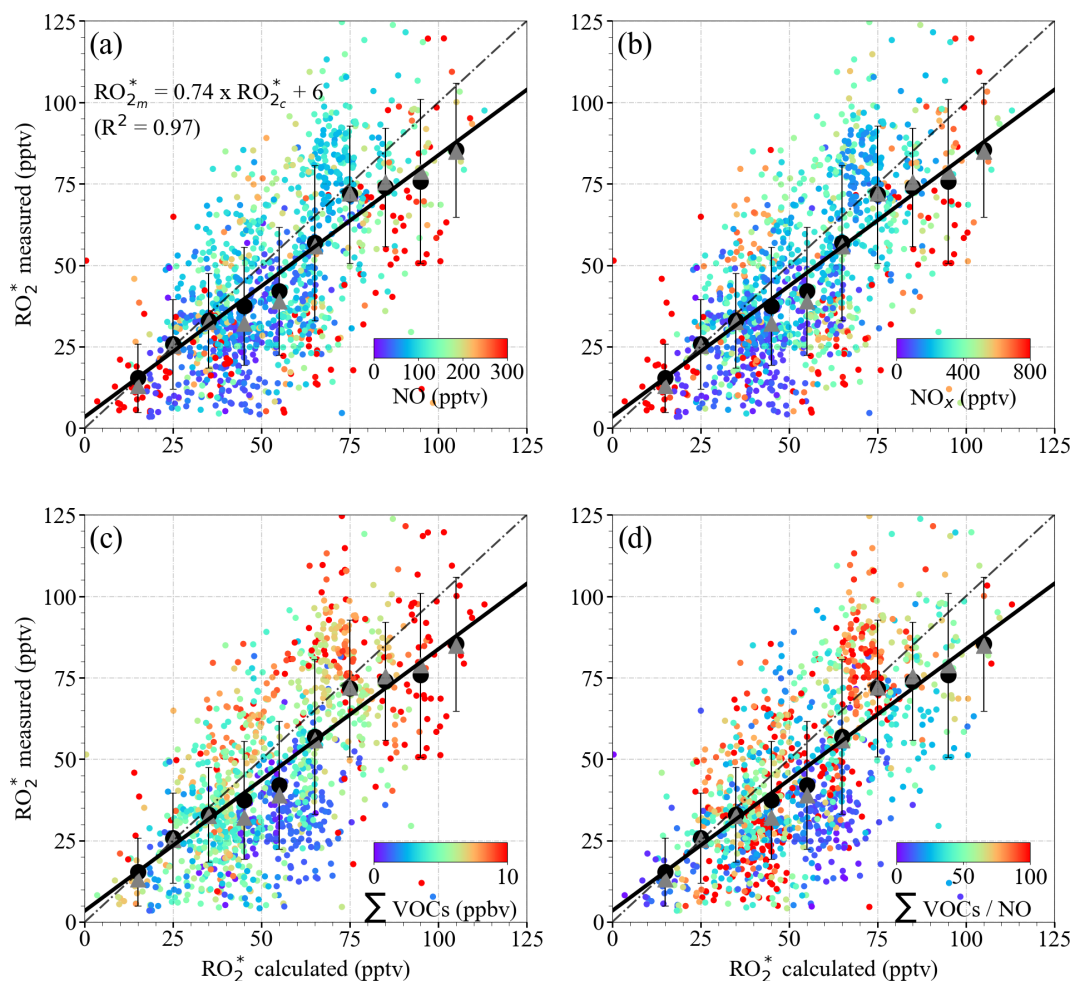
Figure 12. RO_{2m}^* versus RO_{2c}^* using Eq. (9) for \delta = 0.5 colour-coded with the measured (a) NO mixing ratio; (b) NO_x mixing ratio; (c) \Sigma VOCs mixing ratio, where \Sigma VOCs = HCHO + CH_3CHO + (CHO)_2 + CH_3OH + CH_3C(O)CH_3 ; and (d) \Sigma VOCs / NO ratio. The 1 min data (small circles), the mean of the binned RO_{2m}^* over 10 pptv RO_{2c}^* intervals (large circles), and the median of each bin (triangles) are shown. The error bars represent the \pm 1\sigma standard deviation of each bin. The linear regression for the binned values (solid line) and the 1 : 1 relationship (dashed line) are plotted for reference.
