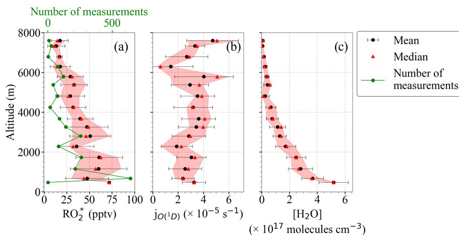
Figure 3. Composite average vertical profiles of (a) \text{RO}_2^* , (b) j_{\text{O}(^1\text{D})} , and (c) [\text{H}_2\text{O}] observations. The measurements are binned over 500 m altitude. The error bars are the \pm 1\sigma standard deviation of each bin. Median values (red triangles), the interquartile 25 %–75 % range (shaded red area), and the number of individual measurements for each bin (in green) are additionally plotted.
