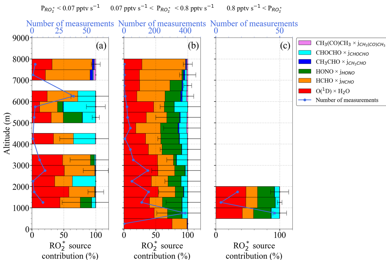
Figure 5. Total P_{RO_2^*} and fractional precursor contributions estimated using Eq. (3) as a function of altitude for (a) P_{RO_2^*} < 0.07 \text{ pptv s}^{-1} , (b) 0.07 \text{ pptv s}^{-1} < P_{RO_2^*} < 0.8 \text{ pptv s}^{-1} , and (c) P_{RO_2^*} > 0.8 \text{ pptv s}^{-1} . Note the different scales in the number of measurements.
