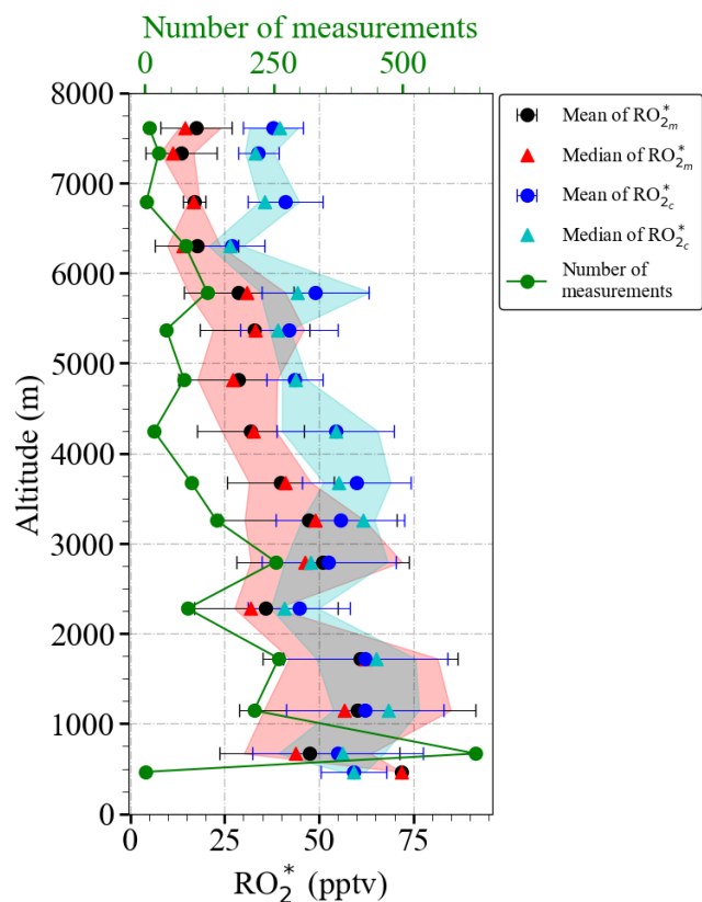
Figure 11. Vertical distribution of the mean \text{RO}_{2\text{m}}^* and mean \text{RO}_{2\text{c}}^* using Eq. (9) for \delta = 0.5 for the EMeRGe data set in Europe. The measurements are binned over 500 m altitude. The error bars are the \pm 1\sigma standard deviation of each bin. Median values (red and cyan triangles), the interquartile 25 %–75 % range (red and blue shaded areas), and the number of individual measurements for each bin (in green) are additionally plotted.
