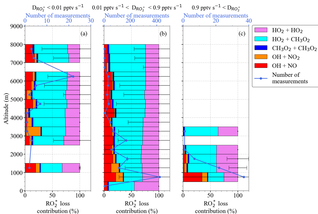
Figure 9. RO_2^* destruction rate ( D_{RO_2^*} ) and fractional contributions from loss reactions in Eq. (6) as a function of altitude for (a) D_{RO_2^*} < 0.01 \text{ pptv s}^{-1} , (b) 0.01 \text{ pptv s}^{-1} < D_{RO_2^*} < 0.9 \text{ pptv s}^{-1} , and (c) D_{RO_2^*} > 0.9 \text{ pptv s}^{-1} . Note the different scales in the number of measurements.
