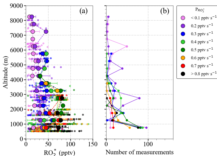
Figure 4. (a) Composite averaged vertical distribution of measured \text{RO}_2^* colour-coded according to the value of P_{\text{RO}_2^*} ; (b) the number of measurements in each altitude bin. Small circles are 1 min individual measurements binned with P_{\text{RO}_2^*} values in 0.1 \text{ pptv s}^{-1} intervals. Larger circles result from a further binning over 500 m altitude steps. All the production rates below 0.1 \text{ pptv s}^{-1} and above 0.8 \text{ pptv s}^{-1} are binned to 0.1 and 0.8 \text{ pptv s}^{-1} , respectively. The error bars are the standard deviation for each altitude bin.
