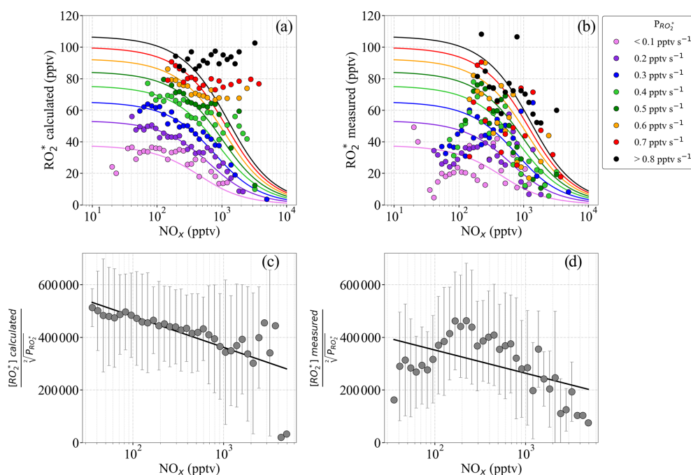
Figure 16. (a) \text{RO}_2^* binned into P_{\text{RO}_2^*} intervals of 0.1 \text{ pptv s}^{-1} versus binned \text{NO}_x ; (b) \text{RO}_2^* binned into P_{\text{RO}_2^*} intervals of 0.1 \text{ pptv s}^{-1} versus binned \text{NO}_x ; (c) ratio of [\text{RO}_2^*]_c to \sqrt{P_{\text{RO}_2^*}} versus \text{NO}_x ; and (d) [\text{RO}_2^*]_m to \sqrt{P_{\text{RO}_2^*}} ratio versus \text{NO}_x . The data in panels (a) and (b) are assigned different colours, as a function of the radical production rate interval. The \text{NO}_x observations are binned into 50 equidistant intervals on a logarithmic scale. The solid lines in panels (a) and (b) are the least square fits, obtained using Eq. (10). In panels (c) and (d), the ratios of [\text{RO}_2^*]_c to \sqrt{P_{\text{RO}_2^*}} and [\text{RO}_2^*]_m to \sqrt{P_{\text{RO}_2^*}} are binned into 50 \text{NO}_x intervals equidistant on the logarithmic scale from 10 to 10 000 pptv. Error bars indicate the \pm 1\sigma standard deviation for the distribution in each bin.
