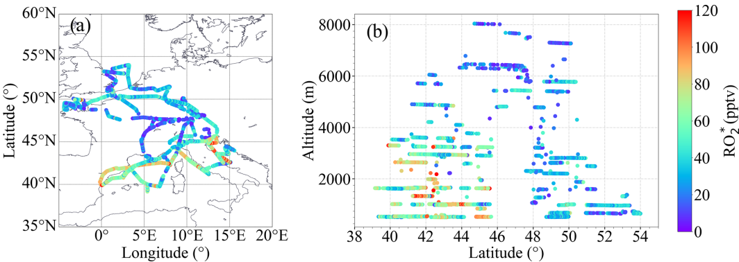
Figure 2. \text{RO}_2^* measured during EMeRGe-Europe: (a) as a function of longitude and latitude and (b) as a function of latitude and altitude.
