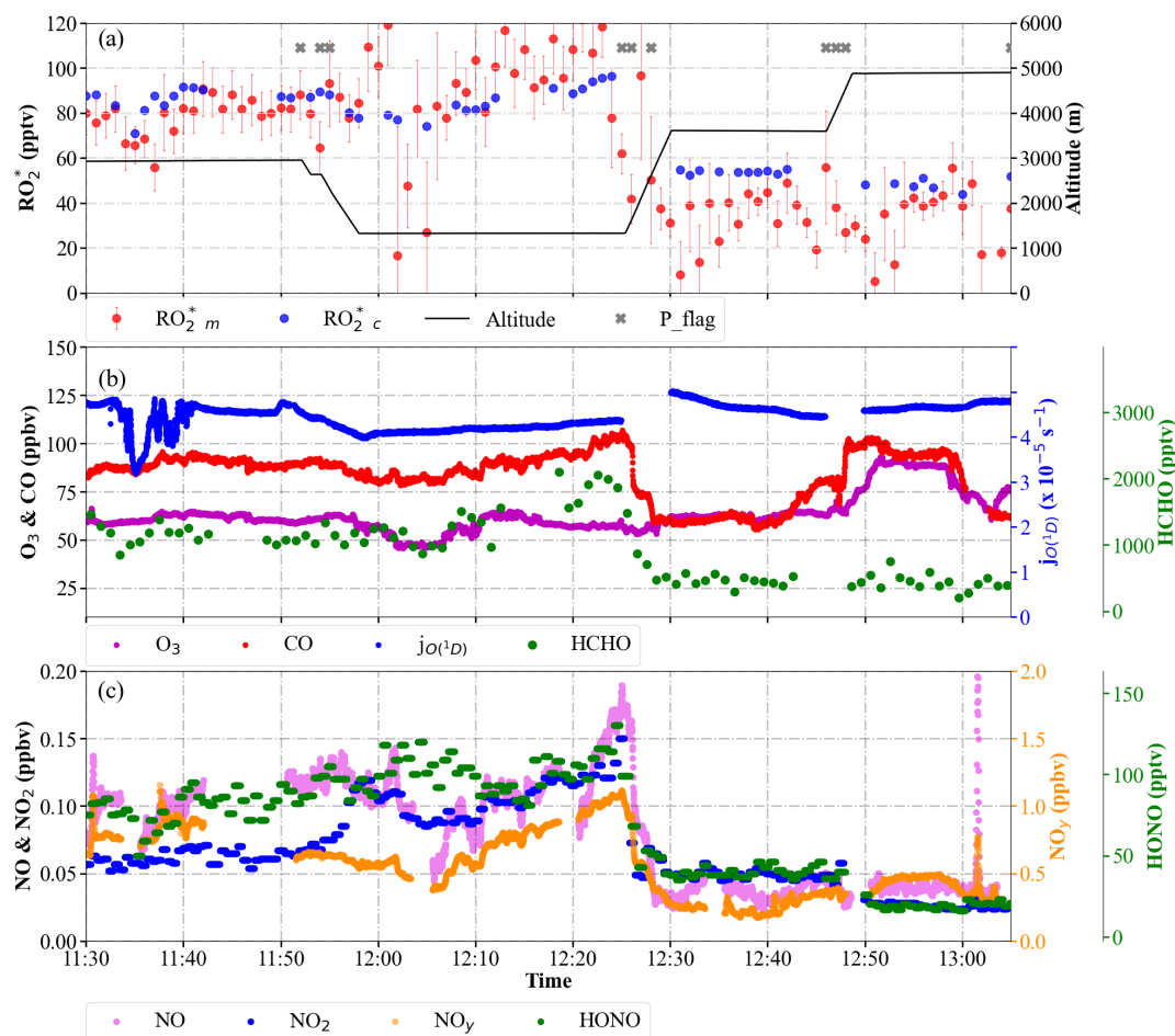
Figure 15. Temporal variation of RO 2 * m and RO 2 * c , selected radical precursors, and j_{O(1D)} along the E-EU-03 flight track: (a) RO 2 * m and RO 2 * c mixing ratios. The flight altitude is indicated in black. The P_flag indicates RO 2 * measurements affected by dynamical pressure variation in the inlet; (b) O 3 , CO, HCHO mixing ratios, and j_{O(1D)} ; (c) NO, NO 2 , NO y , and HONO mixing ratios.
