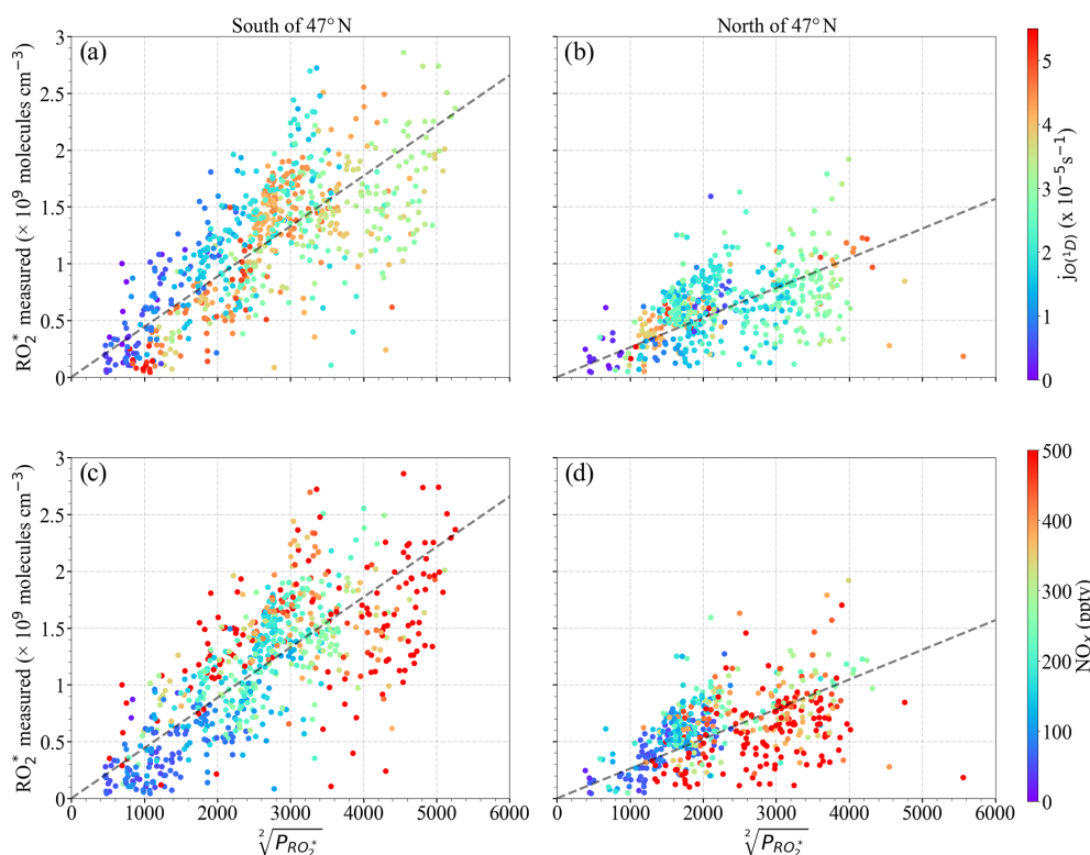
Figure 8. Measured [\text{RO}_2^*] versus \sqrt{P_{\text{RO}_2^*}} for the following latitudes: (a, c) south of 47^\circ\text{N} and (b, d) north of 47^\circ\text{N} . Note that (a) and (b) are colour-coded with j_{\text{O}(^1\text{D})} ; (c) and (d) are colour-coded with the \text{NO}_x mixing ratio. The dashed lines indicate the linear fit for visual support.
