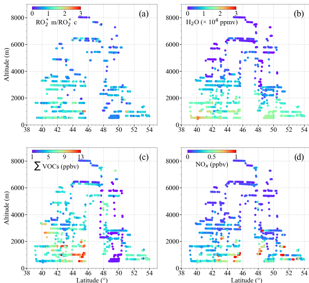
Figure 14. Plots of (a) the ratio of RO_{2m}^* to RO_{2c}^* ( RO_{2m}^* / RO_{2c}^* ) assuming that \delta = 0.5 ; (b) H_2O ; (c) \sum \text{VOCs} ; (d) NO_x as a function of latitude and altitude for the EMeRGe measurements in Europe.
