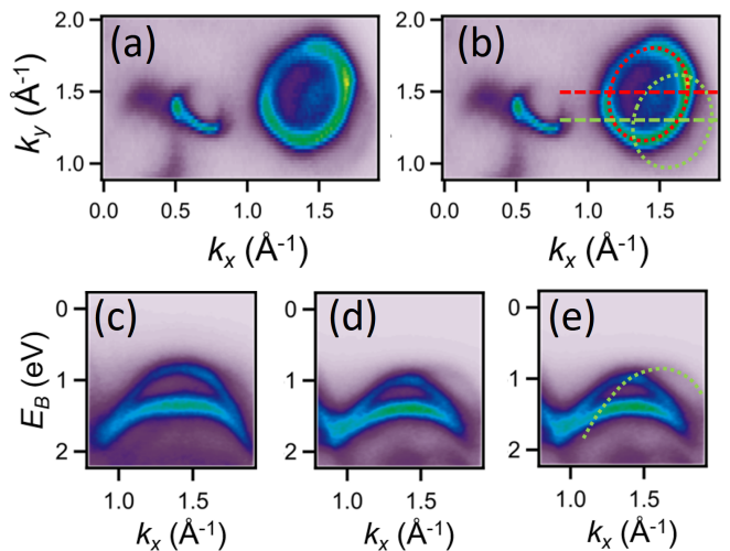
FIG. 4. (a) Details of the spectra from sample A near the \Gamma_1 at E_B = 1.14 eV. (b) Same map as in (a) but with red and green circles indicating the positions of \Gamma_1 from top and bottom layers, respectively. (c) and (d) E_B(k) cuts along the red and green dashed lines indicated in (b), respectively. (e) Same as (d) but with the guide line indicating the dispersion of the bottom layer \Gamma_1 band.
