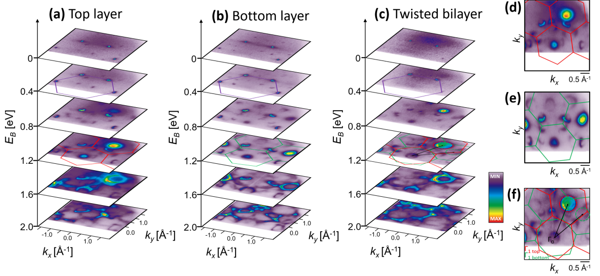
FIG. 2. ARPES spectra from WSe 2 SLs and BL of sample B . (a) and (b) show maps from top and bottom SLs, and (c) from the BL. (d-f) show details of the maps for top SL, bottom SL, and BL, respectively, at E_B = 1.2 eV. Red and green dashed circles in (f) represent the positions of the \Gamma_1 from top and bottom layer, and black arrows depict the twist angle.
