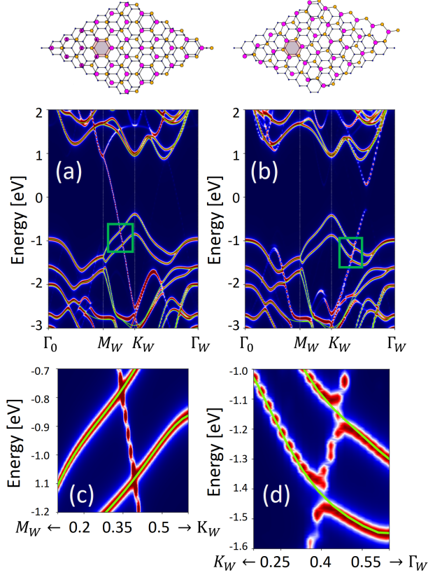
FIG. 10. Theoretical calculations for aligned (a) and 21.79° twisted (b) SL WSe 2 on graphene. The theoretical band structure is deconvoluted onto the Brillouin zone of the freestanding SL WSe 2 . (c) and (d) show magnified areas of the green boxes in (a) and (b), respectively. Green lines (in all panels) show the band structure of a freestanding SL WSe 2 , for comparison.
