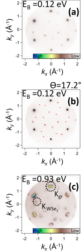
FIG. 9. Maps measured on sample C at the NanoESCA beam-line with p -polarized light at h\nu = 40 eV at 80K. (a) CEM of SL WSe 2 /graphite at E_B = 0.12 eV. (b) same as (a) but overlaid with Dirac copies calculated for 17.2^\circ twist angle between WSe 2 and graphite. (c) CEM at E_B = 0.93 eV, indicating the K points of graphite and WSe 2 .
