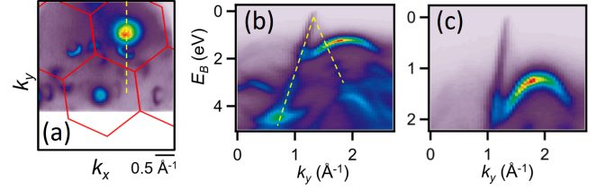
FIG. 7. Crossing between \Gamma_1 and graphite bands in sample B . (a) CEM at E_B = 1.2 eV; yellow dashed line shows the BZ trajectory for maps (b-c). (b) E(k_y) showing the region where graphite and \Gamma_1 band cross; yellow dashed line depicts the graphite Dirac cone dispersion. (c) Magnified region of the crossing.
