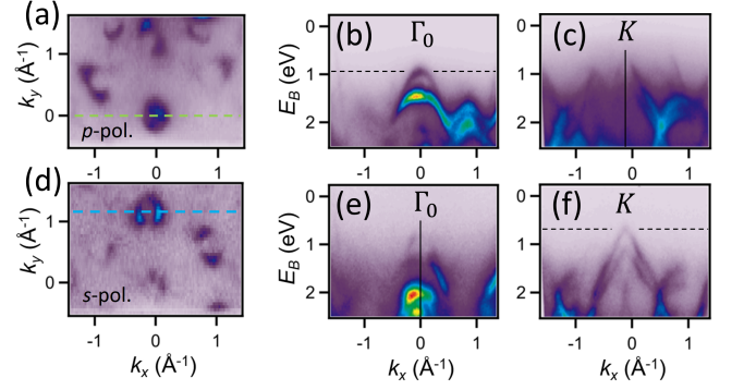
FIG. 6. Selected maps from the BL of sample B . Top row (a-c) CEM at E_B = 1 eV for p -polarized light. Bottom row (d-f) CEM at E_B = 1 eV for s -polarized light. Green dashed line in (a) shows the momentum trajectory for maps (b) and (e). Blue dashed line (d) shows the momentum trajectory for (c) and (f). Black dashed lines in (b) and (f) indicate the local VBM at \Gamma_0 and K points respectively.
