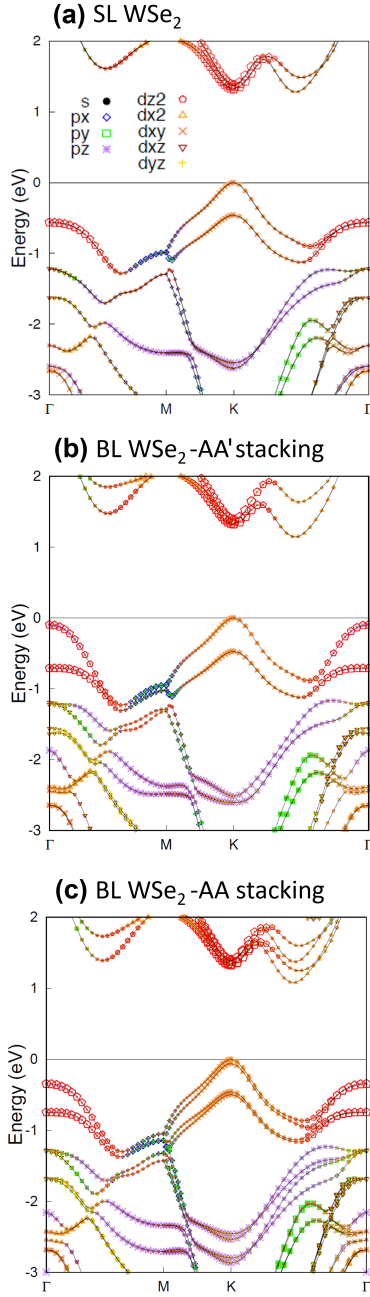
FIG. 5. Calculated orbital characters for the (a) freestanding SL, (b) AA' (2H) BL, and (c) AA BL WSe 2 [17].
