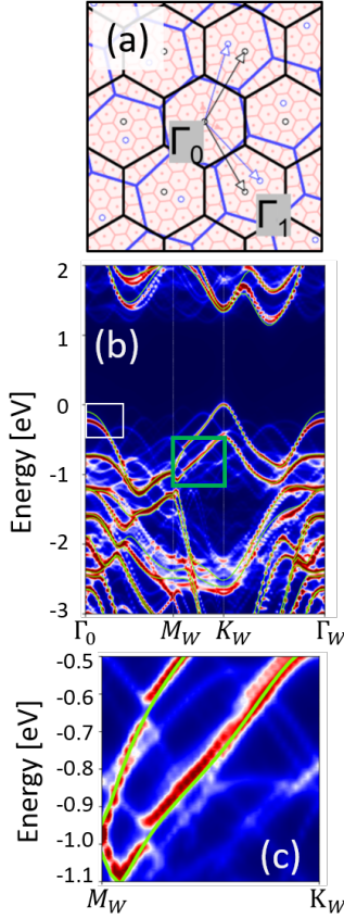
FIG. 11. Theoretical calculations for twisted BL WSe 2 at the twist angle \theta = 60^\circ - 13.17^\circ = 46.83^\circ . (a) Black and blue lines depict BZs of the two SLs and the network red lines the moiré BZs of the twisted layers. (b) Band structure unfolded onto the BZ one of the SL WSe 2 . (c) Magnified region depicted by the green rectangle in (b). For comparison, green solid lines show the bands for the 2H BL WSe 2 .
