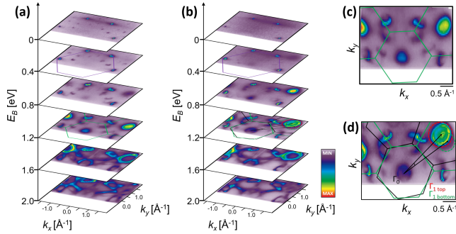
FIG. 3. ARPES spectra from WSe 2 SLs and BL of sample A . (a) shows the maps from the bottom SL and (b) from the BL. (c-d) show details of the maps from bottom SL, and BL, respectively, at E_B = 1.2 eV. Red and green dashed circles in (d) represent the positions of the \Gamma_1 from top and bottom layer, and black arrows depict the twist angle.
