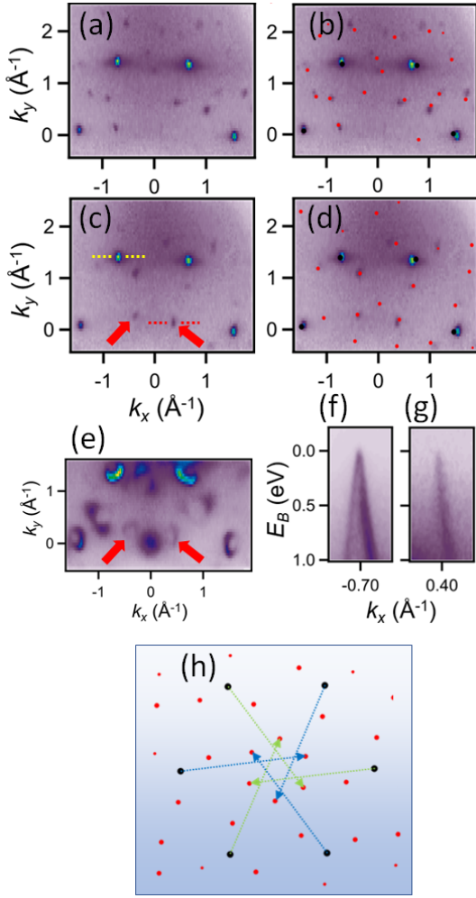
FIG. 8. (a-b) Fermi level CEMs ( E_B = 30 meV) for the bottom SL WSe 2 /graphite in sample B . (c-d) Same for the top SL WSe 2 /graphite in sample B . (e) CEM for the top SL WSe 2 /graphite at E_B = 1 eV. (f) and (g) show E_B(k_x) maps of zero order graphite K point and one of the copies along the trajectories indicated respectively by yellow and red dashed lines in (c). Red arrows in (c) and (e) identify selected copies of graphite K points, confirming conical shapes of their dispersions. (h) Arrangement of copies related to (d) with indicated \mathbf{G}_W vectors of SL WSe 2 . Different color of the arrows reflect the trigonal symmetry of SL WSe 2 .
