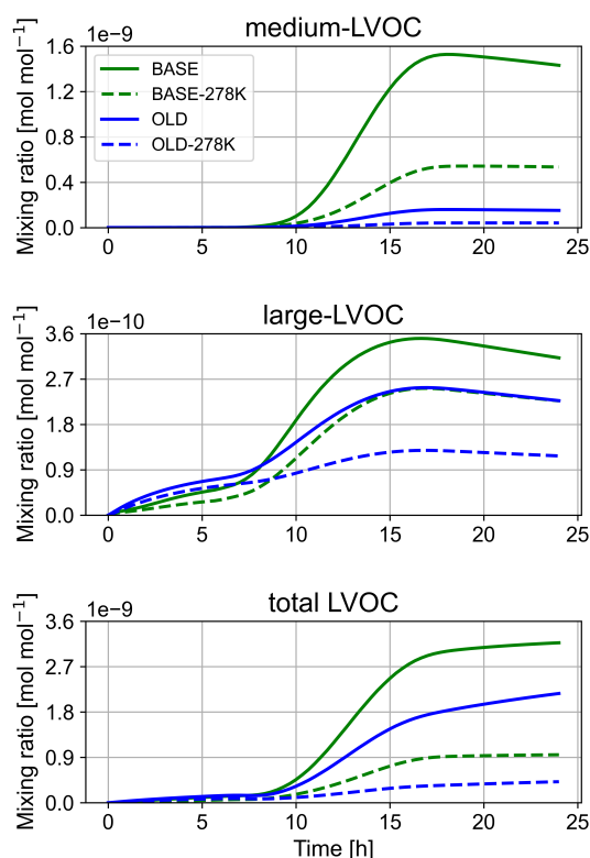
Figure 6. Temperature dependence of the LVOC formation. Results from the BASE run are shown in green, while results from the OLD run are depicted in blue. The lower temperature runs BASE-278K and OLD-278K are displayed as dashed lines.
