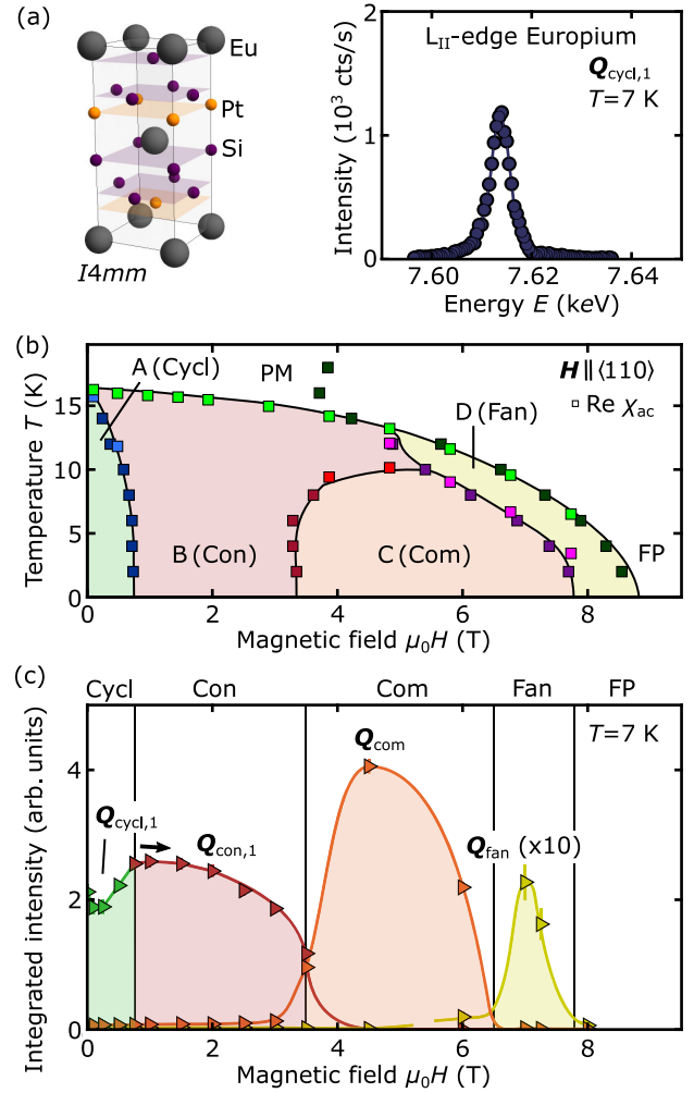
FIG. 1. Crystallographic and magnetic properties of EuPtSi 3 . (a) Tetragonal unit cell of EuPtSi 3 , space group I4mm , and resonant enhancement of the magnetic Bragg intensity when tuning the incident photon energy across the L II edge of europium, characteristic of magnetism predominantly carried by Eu 2+ moments. (b) Magnetic phase diagram for field parallel to [\bar{1}10] , as inferred from susceptibility \text{Re}\chi_{ac} [61]. Antiferromagnetic phases with cyclodial (Cycl, green), conical (Con, red), commensurate (Com, orange), and fanlike (Fan, yellow) order as well as paramagnetic (PM) and field-polarized (FP) regimes may be distinguished. (c) Field dependence of the REXS intensities at Bragg positions characteristic of the different magnetic phases.
