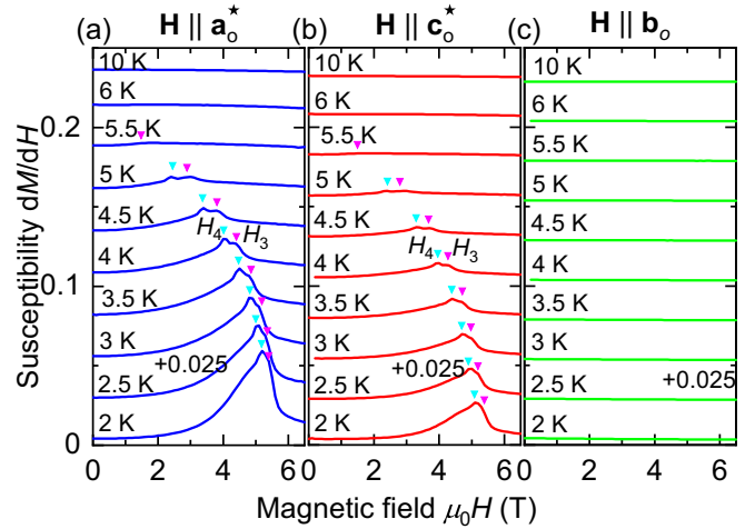
FIG. 6. (a) Susceptibility, dM/dH , calculated from the measured magnetization of orthorhombic \text{CePdAl}_3 for (a) \mathbf{H} \parallel \mathbf{a}_o^* , (b) \mathbf{H} \parallel \mathbf{c}_o^* , and (c) \mathbf{H} \parallel \mathbf{b}_o . Data are shifted by 0.025 for clarity. Peaks correspond to field-induced transitions marked by arrows at H_3 (pink) and H_4 (light blue). The peaks disappear above T_1 .
