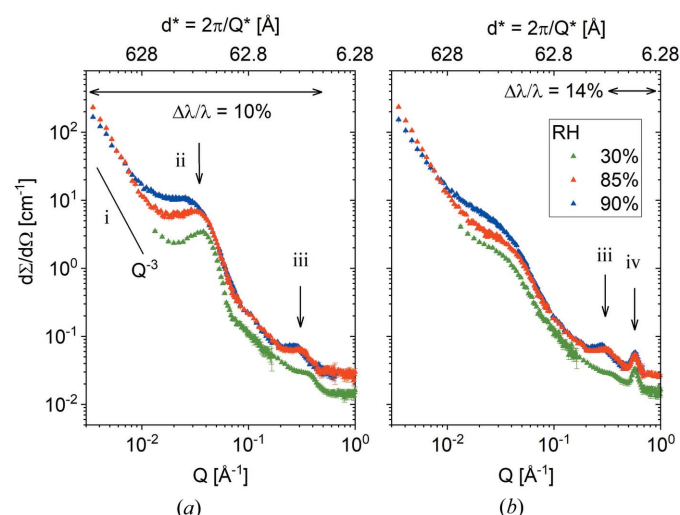
Figure 4 SANS patterns from the sample M0 exposed to different RH states at room temperature, as averaged over the meridional (a) and equatorial (b) sectors. The scattering features are indicated by roman numbers as follows: (i) the power-law behaviour at low Q ; (ii) the interlamellar reflection; (iii) the ionomer peak; (iv) the 010 crystalline reflection. \Delta\lambda/\lambda in different Q ranges is also indicated.
