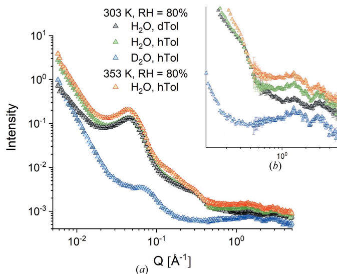
Figure 7 SANS patterns measured in TOF mode at TAIKAN from the sample M2 in different contrast conditions as exposed to different RH/T conditions and averaged over the meridional sectors. The RH and T conditions are indicated in the legend. The main plot (a) presents the full patterns measured over a wide Q range by combining different detection banks, while the inset (b) depicts the WANS patterns.
