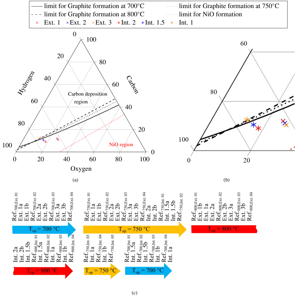
Figure 2: (a) calculated C-H-O ternary diagram and (b) detail view of the area where the tested gas compositions are located and (c) the test procedure over time.
