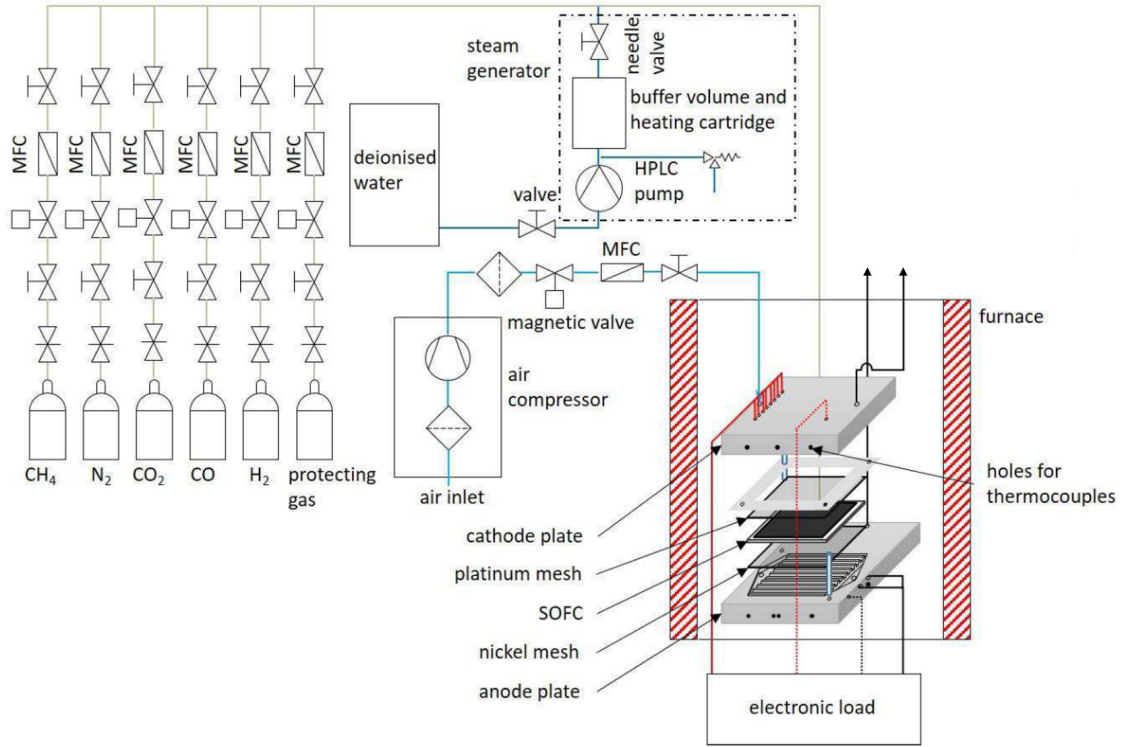
Figure 1: Scheme of the used single cell test rig [30].
