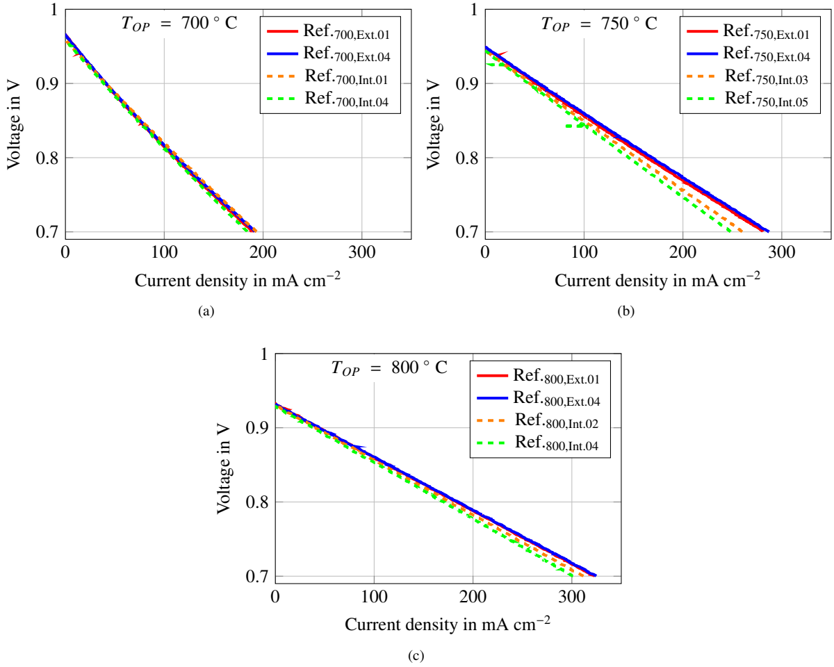
Figure 6: I-V curves of reference measurements at an operating temperature of (a) 700 °C, (b) 750 °C and (c) 800 °C, (—) at the beginning of testing, (—) after testing externally reformed gas compositions, (- - -) after testing the first internal reformed gas compositions and (- - -) at the end of testing at the respective operating temperature.
