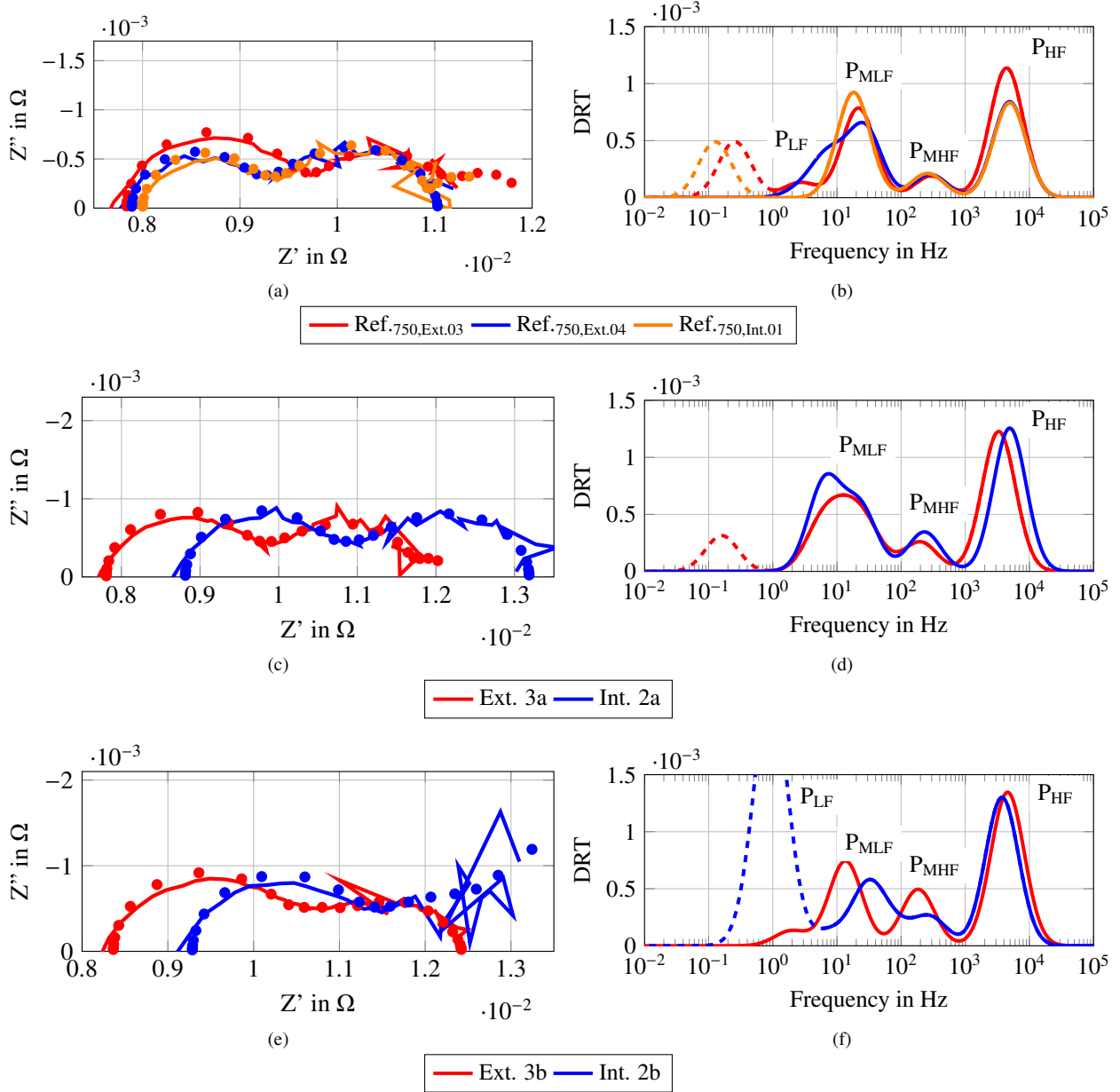
Figure 8: Nyquist plots (a), (c) and (e) of (-) measured EIS, (o) from DRT recalculated EIS and DRT plots (b), (d) and (f) of direct internally (Int.) reformed methane, externally reformed (Ext.) methane and their surrounding reference measurements (Ref.750,Ext.03, Ref.750,Ext.04 and Ref.750,Int.01) at 750 °C and 100 mA cm -2 .
