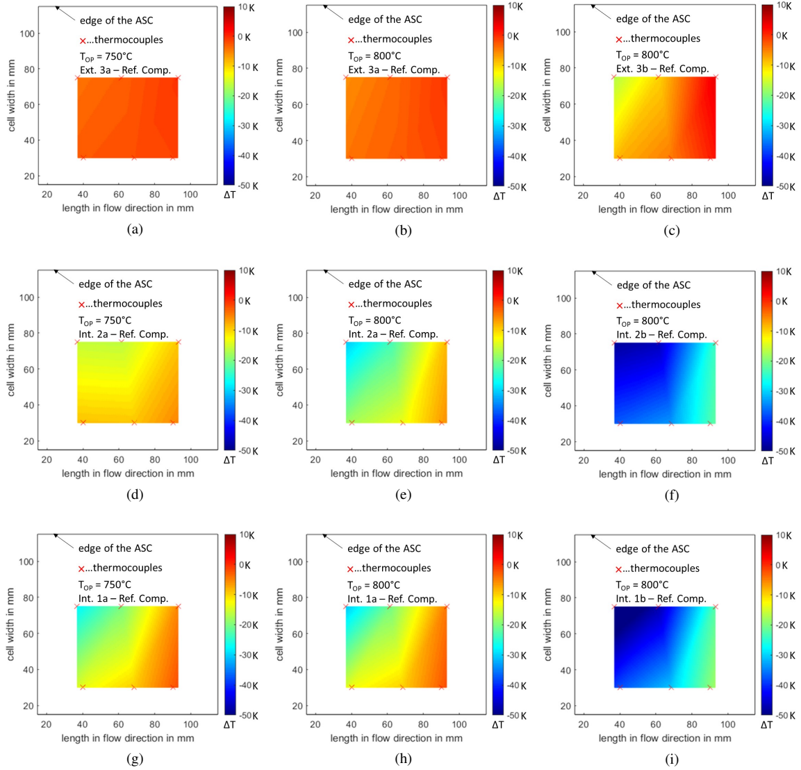
Figure 5: Measured temperature profiles as temperature difference between tested reforming conditions and their respective reference measurement (Ref. Comp.) at 100 \text{ mA cm}^{-2} .
