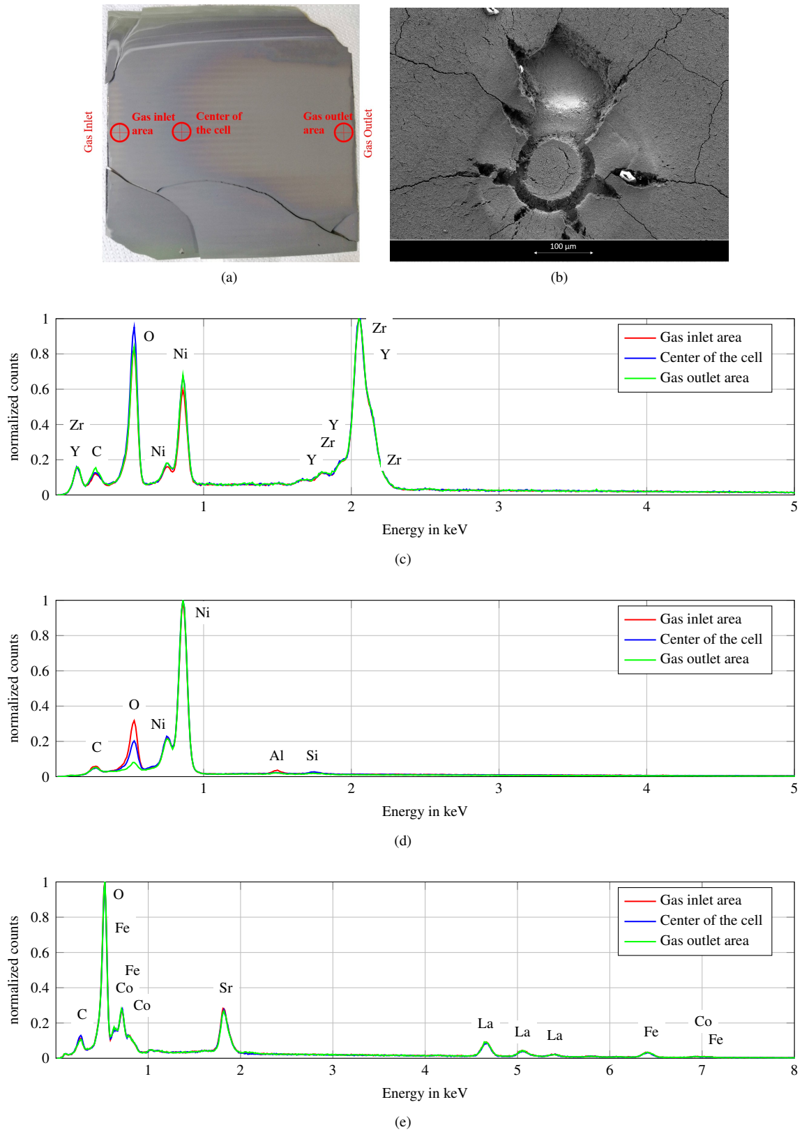
Figure 4: (a) investigated areas of the cell, (b) SEM image of cathode delamination and cracking at the center area of the cell. EDS of the (c) fuel electrode, (d) Ni-mesh of the fuel electrode and (e) air electrode.
