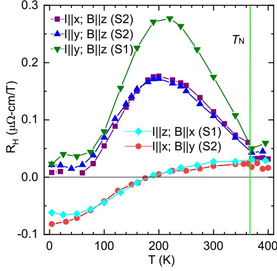
Figure 5.15: Temperature dependence of Hall coefficient ( R_H ) for different samples, under different conditions.
