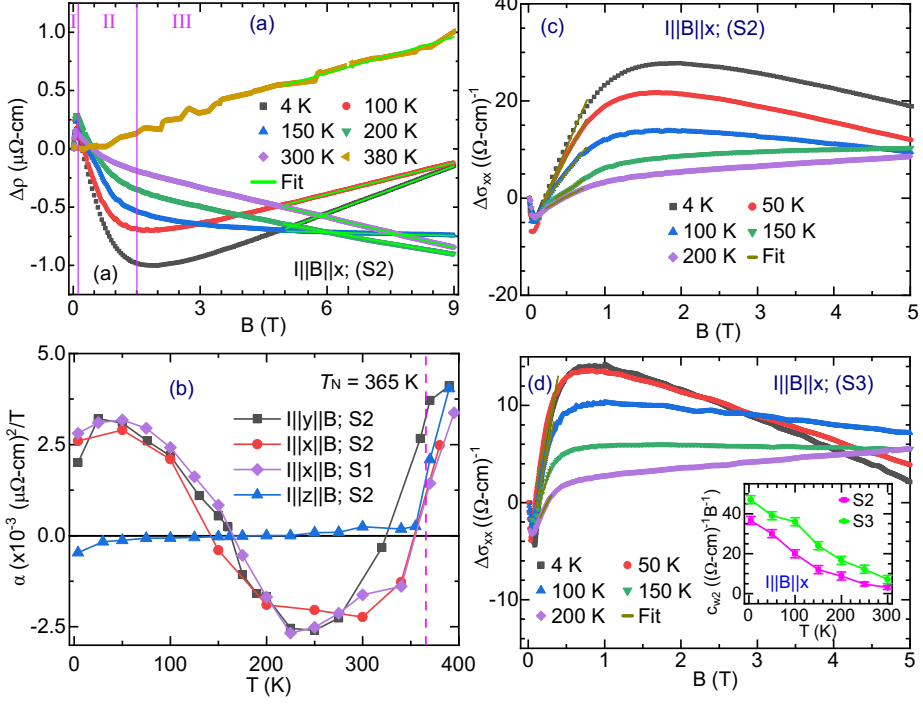
Figure 5.4: (a) shows LMR along the x axis, corresponding to the \text{Mn}_3\text{Ge} . Here, \Delta\rho = \rho(B) - \rho(0) . At high field ( B > 5 \text{ T} ), the data is fitted with \rho_{[\text{high } B]} = \alpha(B/\rho_0) , and fitting is denoted as ‘Fit’. I, II, and III denote three different field regimes where the nature of LMR is different. (b) Temperature dependence of \alpha (high field slope) corresponding to different samples. (c), and (d) show LMC along the x axis, for S2 and S3 samples, respectively. Here, \Delta\sigma_{ii} = \sigma_{ii}(B) - \sigma_{ii}(0) . In the case of S2 and S3 samples, LMC below 0.8 T and 0.4 T, respectively, is fitted with \sigma_{[\text{low } B]} = c_{w2}B . The evolution of c_{w2} with temperature is shown in (d) inset.
