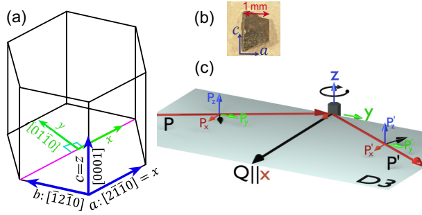
Figure 6.1: (a) Crystallographic axes in the hexagonal and Cartesian coordinate. (b) Picture of the crystal used during the neutron diffraction. (c) Illustration of the diffraction geometry of the CRYOPAD setup. The sample is rotated in the x - y plane. P' and P denote scattered and incident neutron beam.
