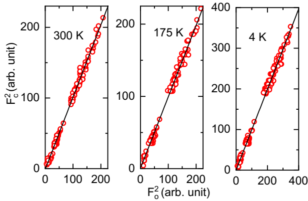
Figure 5.18: Calculated vs. observed intensity corresponding to model I, at different temperatures. F_c^2 , and F_o^2 denote calculated and observed intensities, respectively.
